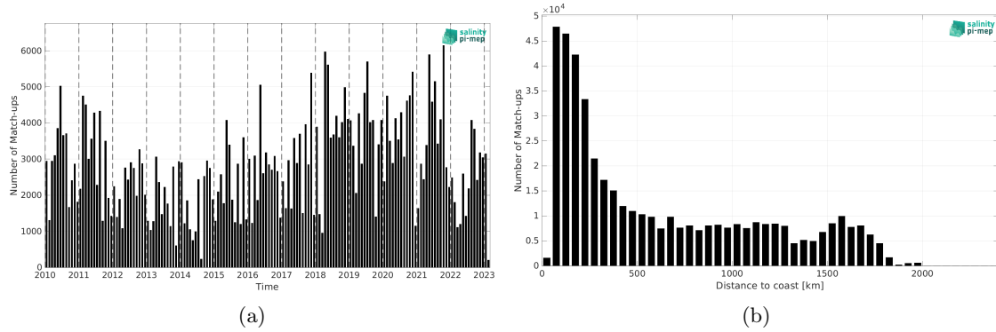
Figure 2: Number of match-ups between TSG (LEGOS-DM) and CCI SSS L4 Merged-OI v5.5 - 7-day running (ESA) SSS as a function of time (a) and as function of the distance to coast (b) over the Tropical Atlantic Ocean Pi-MEP region and for the full satellite product period.
