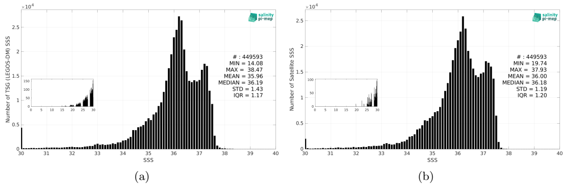
Figure 3: Histograms of SSS from TSG (LEGOS-DM) (a) and CCI SSS L4 Merged-OI v5.5 - 7-day running (ESA) (b) considering all match-up pairs per bins of 0.1 over the Tropical Atlantic Ocean Pi-MEP region and for the full satellite product period.
