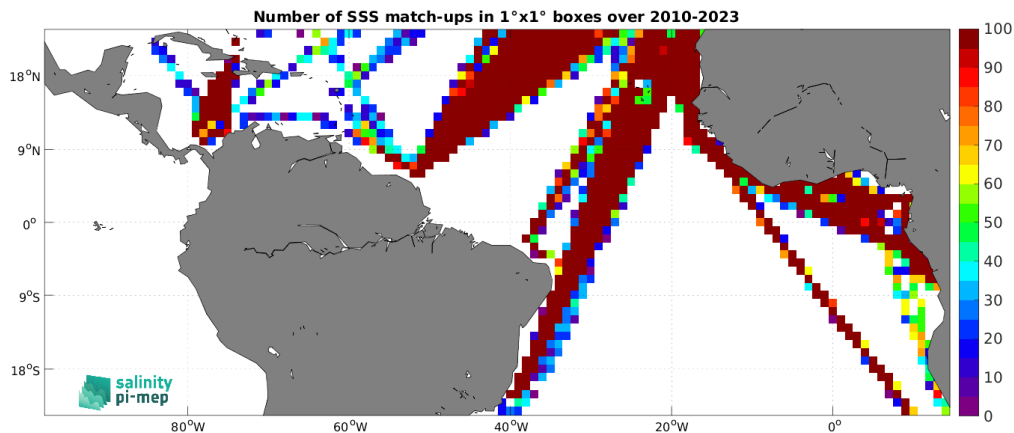
Figure 5: Number of SSS match-ups between TSG (LEGOS-DM) SSS and the CCI SSS L4 Merged-OI v5.5 - 7-day running (ESA) SSS product for the Tropical Atlantic Ocean Pi-MEP region over 1^\circ \times 1^\circ boxes and for the full satellite product period.
