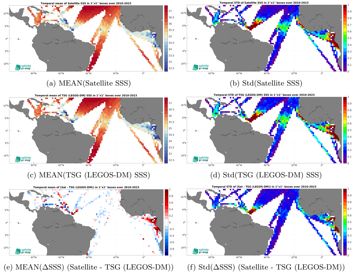
Figure 7: Temporal mean (left) and Std (right) of SSS from CCI SSS L4 Merged-OI v5.5 - 7-day running (ESA) (top), TSG (LEGOS-DM) ( in situ ) dataset (middle), and of \Delta SSS (Satellite - TSG (LEGOS-DM)). Only match-up pairs are used to generate these maps.
