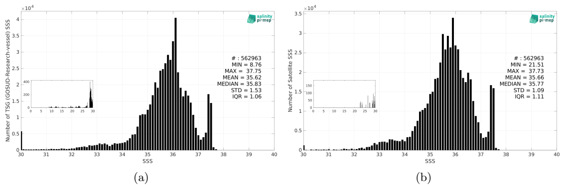
Figure 3: Histograms of SSS from TSG (GOSUD-Research-vessel) (a) and CCI SSS L4 Merged-OI v5.5 - 7-day running (ESA) (b) considering all match-up pairs per bins of 0.1 over the Tropical Atlantic Ocean Pi-MEP region and for the full satellite product period.
