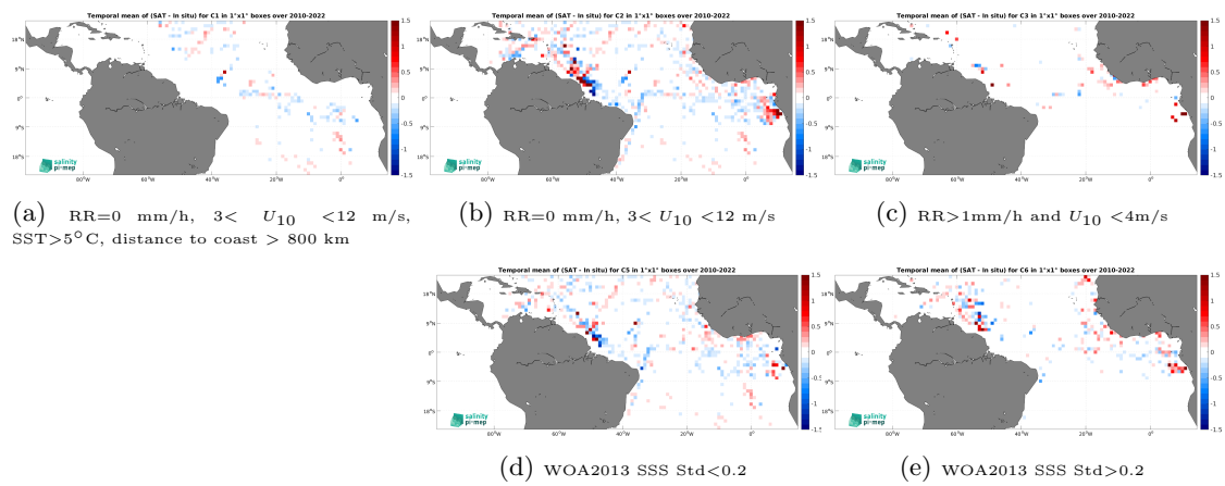
Figure 14: Temporal mean gridded over spatial boxes of size 1^\circ \times 1^\circ of \Delta\text{SSS} (CCI SSS L4 Merged-OI v5.5 - 7-day running (ESA) - TSG (GOSUD-Research-vessel)) for 5 different subdatasets corresponding to:RR=0 mm/h, 3 < U_{10} < 12 m/s, SST >5^\circ\text{C} , distance to coast > 800 km (a), RR=0 mm/h, 3 < U_{10} < 12 m/s (b), RR >1 mm/h and U_{10} < 4 m/s (c), WOA2013 SSS Std <0.2 (d), WOA2013 SSS Std >0.2 (e).
