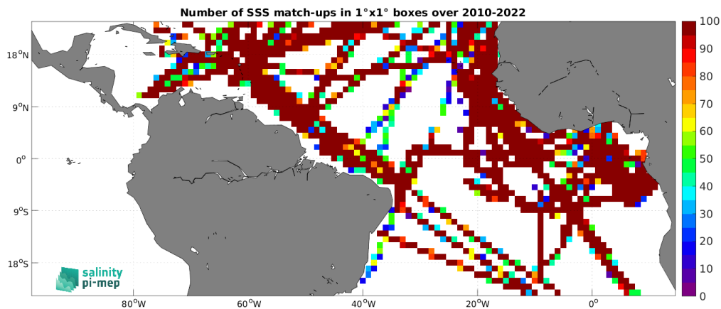
Figure 5: Number of SSS match-ups between TSG (GOSUD-Research-vessel) SSS and the CCI SSS L4 Merged-OI v5.5 - 7-day running (ESA) SSS product for the Tropical Atlantic Ocean Pi-MEP region over 1^\circ \times 1^\circ boxes and for the full satellite product period.
