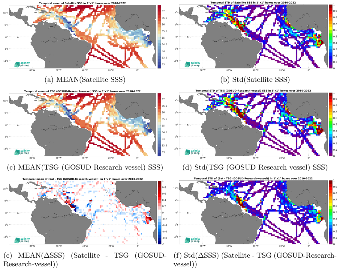
Figure 7: Temporal mean (left) and Std (right) of SSS from CCI SSS L4 Merged-OI v5.5 - 7-day running (ESA) (top), TSG (GOSUD-Research-vessel) (middle), and of \Delta SSS (Satellite - TSG (GOSUD-Research-vessel)). Only match-up pairs are used to generate these maps.
