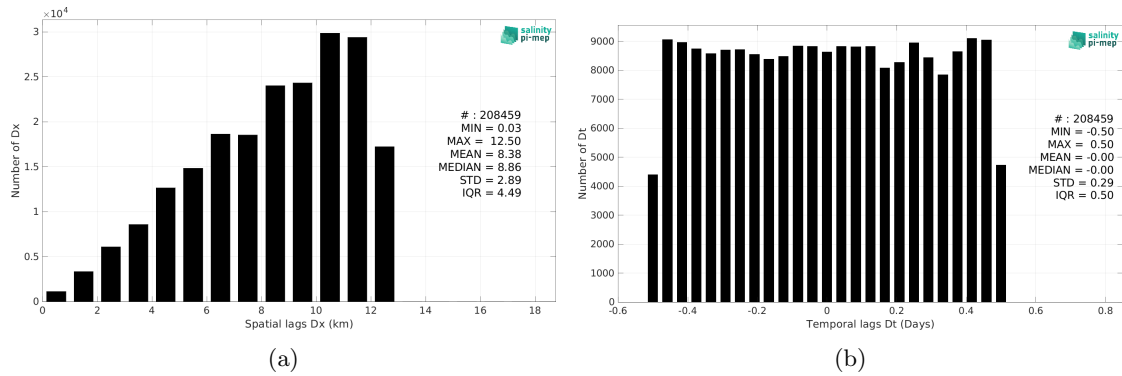
Figure 6: Histograms of the spatial (a) and temporal (b) lags between the location/time of the TSG (CSIC-UTM) measurement and the date of the corresponding CCI SSS L4 Merged-OI v5.5 - 7-day running (ESA) SSS pixel.
