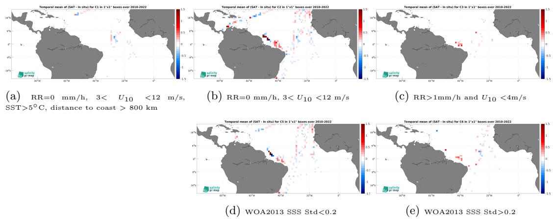
Figure 14: Temporal mean gridded over spatial boxes of size 1^\circ \times 1^\circ of \Delta\text{SSS} (CCI SSS L4 Merged-OI v5.5 - 7-day running (ESA) - TSG (CSIC-UTM)) for 5 different subdatasets corresponding to:RR=0 mm/h, 3 < U_{10} < 12 m/s, SST >5^\circ\text{C} , distance to coast > 800 km (a), RR=0 mm/h, 3 < U_{10} < 12 m/s (b), RR >1 mm/h and U_{10} < 4 m/s (c), WOA2013 SSS Std <0.2 (d), WOA2013 SSS Std >0.2 (e).
