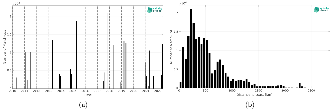
Figure 2: Number of match-ups between TSG (CSIC-UTM) and CCI SSS L4 Merged-OI v5.5 - 7-day running (ESA) SSS as a function of time (a) and as function of the distance to coast (b) over the Tropical Atlantic Ocean Pi-MEP region and for the full satellite product period.
