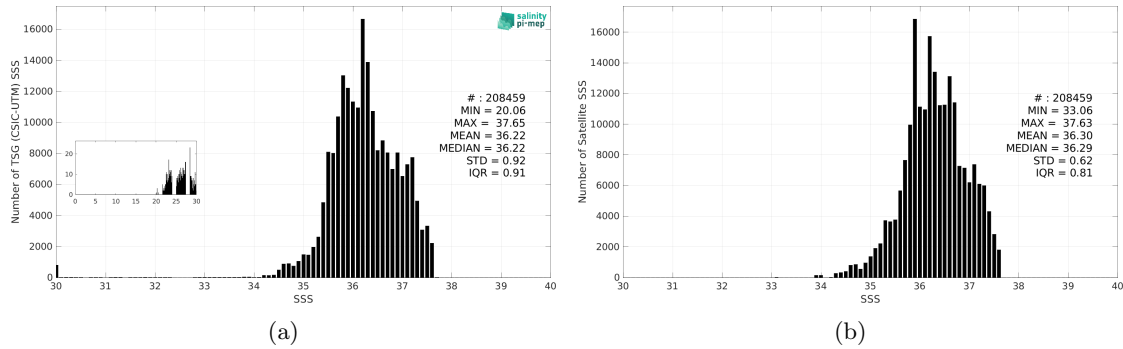
Figure 3: Histograms of SSS from TSG (CSIC-UTM) (a) and CCI SSS L4 Merged-OI v5.5 - 7-day running (ESA) (b) considering all match-up pairs per bins of 0.1 over the Tropical Atlantic Ocean Pi-MEP region and for the full satellite product period.
