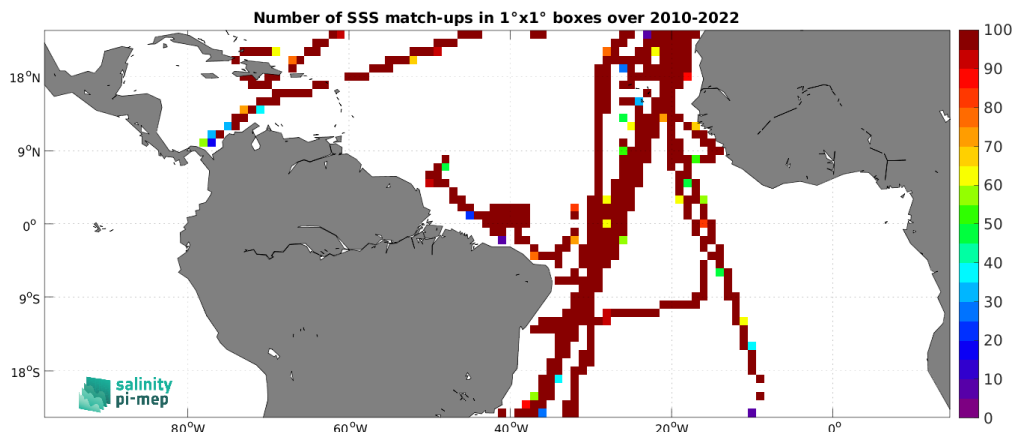
Figure 5: Number of SSS match-ups between TSG (CSIC-UTM) SSS and the CCI SSS L4 Merged-OI v5.5 - 7-day running (ESA) SSS product for the Tropical Atlantic Ocean Pi-MEP region over 1^\circ \times 1^\circ boxes and for the full satellite product period.
