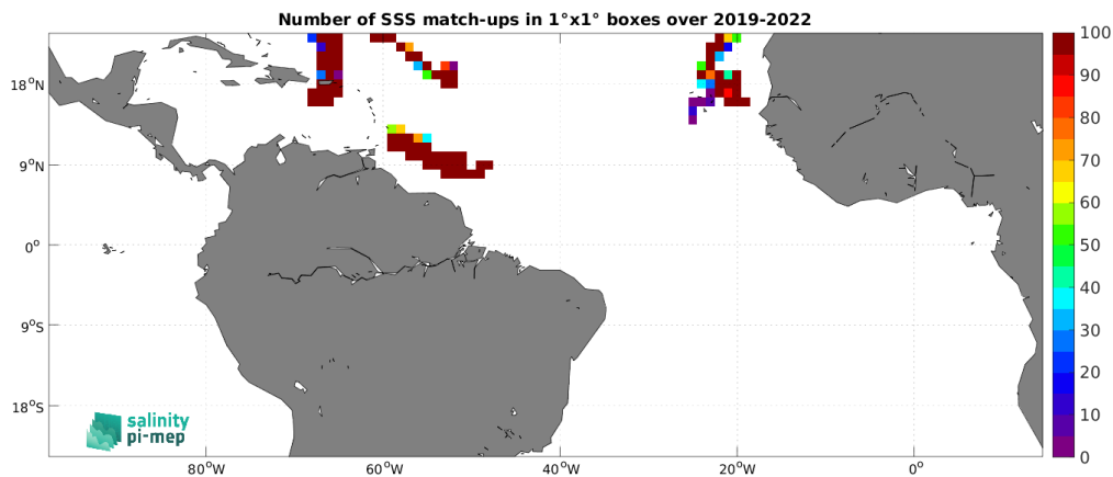
Figure 5: Number of SSS match-ups between Saildrone SSS and the CCI SSS L4 Merged-OI v5.5 - 7-day running (ESA) SSS product for the Tropical Atlantic Ocean Pi-MEP region over 1^\circ \times 1^\circ boxes and for the full satellite product period.
