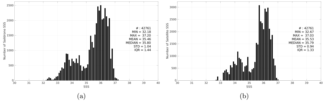
Figure 3: Histograms of SSS from Saildrone (a) and CCI SSS L4 Merged-OI v5.5 - 7-day running (ESA) (b) considering all match-up pairs per bins of 0.1 over the Tropical Atlantic Ocean Pi-MEP region and for the full satellite product period.
