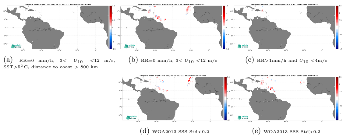
Figure 14: Temporal mean gridded over spatial boxes of size 1^\circ \times 1^\circ of \Delta\text{SSS} (CCI SSS L4 Merged-OI v5.5 - 7-day running (ESA) - Saildrone) for 5 different subdatasets corresponding to:RR=0 mm/h, 3 < U_{10} < 12 m/s, SST >5^\circ\text{C} , distance to coast > 800 km (a), RR=0 mm/h, 3 < U_{10} < 12 m/s (b), RR >1 mm/h and U_{10} < 4 m/s (c), WOA2013 SSS Std <0.2 (d), WOA2013 SSS Std >0.2 (e).
