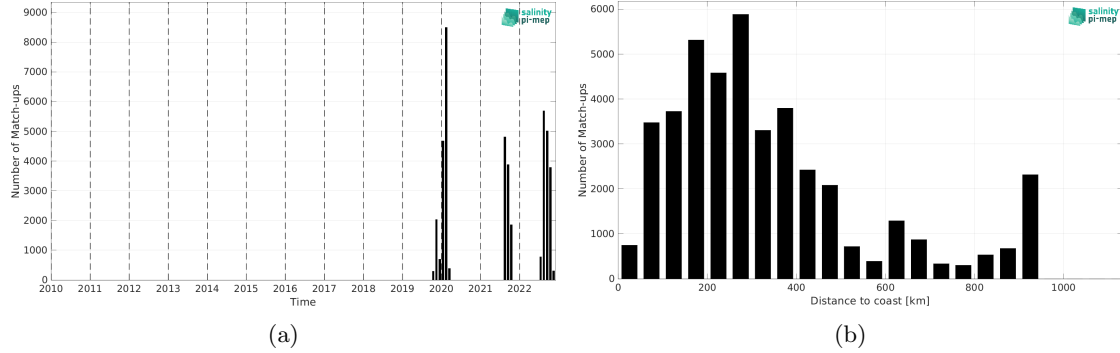
Figure 2: Number of match-ups between Saildrone and CCI SSS L4 Merged-OI v5.5 - 7-day running (ESA) SSS as a function of time (a) and as function of the distance to coast (b) over the Tropical Atlantic Ocean Pi-MEP region and for the full satellite product period.
