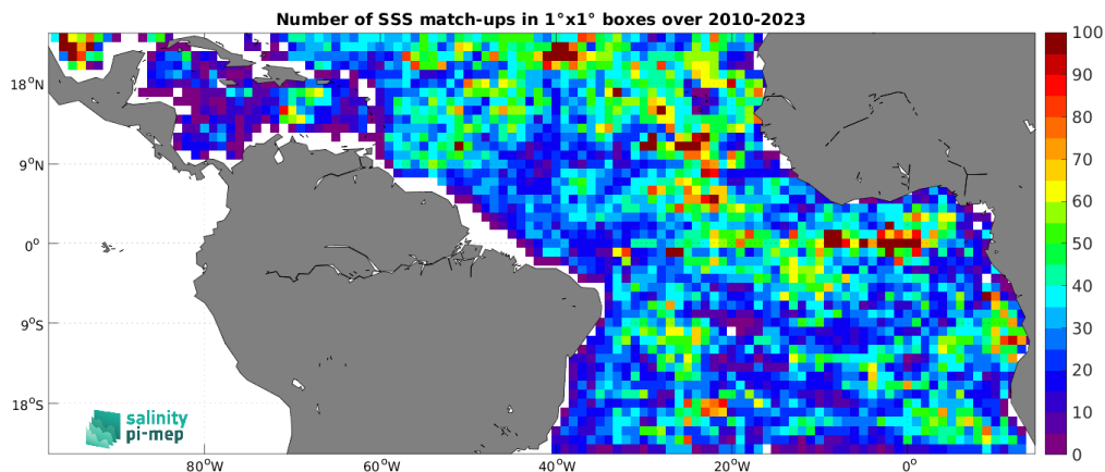
Figure 5: Number of SSS match-ups between Argo SSS and the CCI SSS L4 Merged-OI v5.5 - 7-day running (ESA) SSS product for the Tropical Atlantic Ocean Pi-MEP region over 1^\circ \times 1^\circ boxes and for the full satellite product period.
