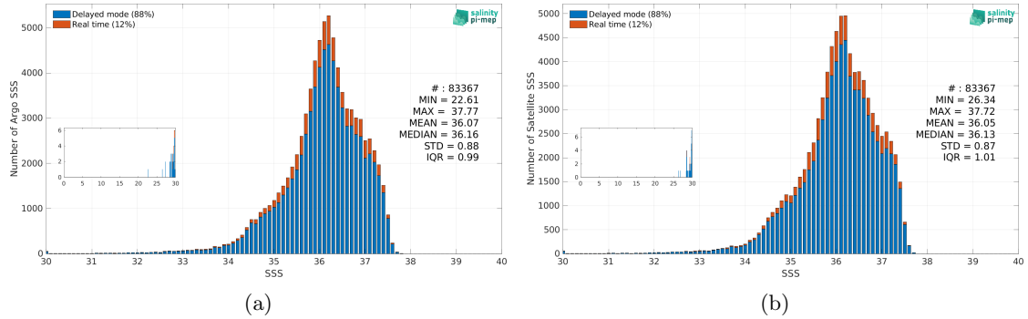
Figure 3: Histograms of SSS from Argo (a) and CCI SSS L4 Merged-OI v5.5 - 7-day running (ESA) (b) considering all match-up pairs per bins of 0.1 over the Tropical Atlantic Ocean Pi-MEP region and for the full satellite product period.
