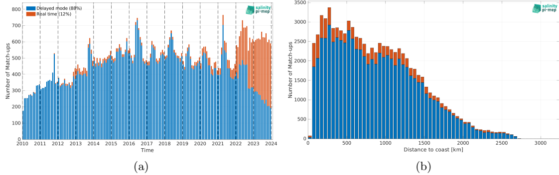
Figure 2: Number of match-ups between Argo and CCI SSS L4 Merged-OI v5.5 - 7-day running (ESA) SSS as a function of time (a) and as function of the distance to coast (b) over the Tropical Atlantic Ocean Pi-MEP region and for the full satellite product period.
