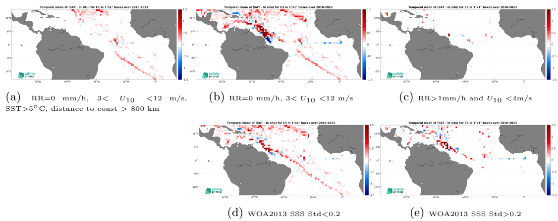
Figure 14: Temporal mean gridded over spatial boxes of size 1^\circ \times 1^\circ of \Delta\text{SSS} (CCI SSS L4 Merged-OI v5.5 - 30-day running (ESA) - TSG (SAMOS)) for 5 different subdatasets corresponding to:RR=0 mm/h, 3 < U_{10} < 12 m/s, SST>5°C, distance to coast > 800 km (a), RR=0 mm/h, 3 < U_{10} < 12 m/s (b), RR>1mm/h and U_{10} < 4 m/s (c), WOA2013 SSS Std<0.2 (d), WOA2013 SSS Std>0.2 (e).
