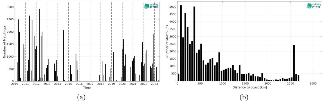
Figure 2: Number of match-ups between TSG (SAMOS) and CCI SSS L4 Merged-OI v5.5 - 30-day running (ESA) SSS as a function of time (a) and as function of the distance to coast (b) over the Tropical Atlantic Ocean Pi-MEP region and for the full satellite product period.
