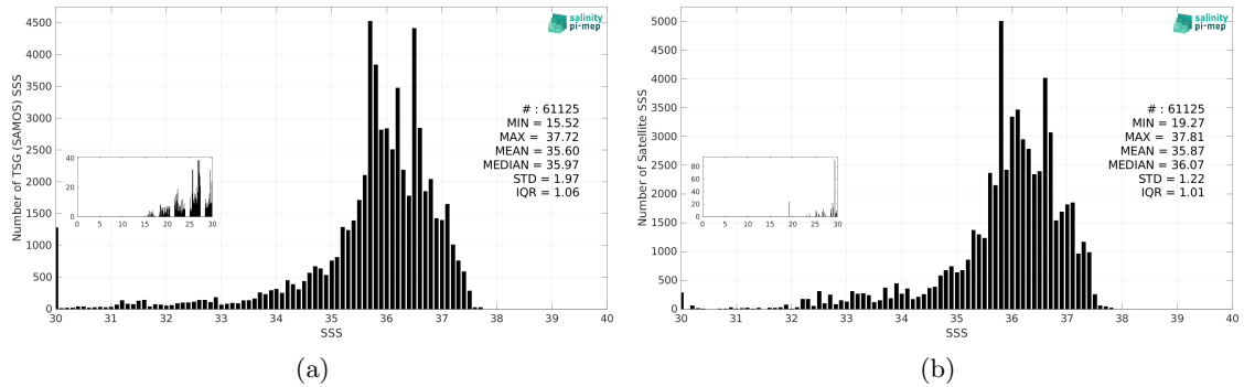
Figure 3: Histograms of SSS from TSG (SAMOS) (a) and CCI SSS L4 Merged-OI v5.5 - 30-day running (ESA) (b) considering all match-up pairs per bins of 0.1 over the Tropical Atlantic Ocean Pi-MEP region and for the full satellite product period.
