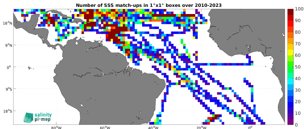
Figure 5: Number of SSS match-ups between TSG (SAMOS) SSS and the CCI SSS L4 Merged-OI v5.5 - 30-day running (ESA) SSS product for the Tropical Atlantic Ocean Pi-MEP region over 1^\circ \times 1^\circ boxes and for the full satellite product period.
