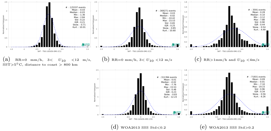
Figure 15: Normalized histogram of \Delta\text{SSS} (CCI SSS L4 Merged-OI v5.5 - 30-day running (ESA) - TSG (LEGOS-DM)) for 5 different subdatasets corresponding to: RR=0 mm/h, 3 < U_{10} < 12 m/s, SST > 5^\circ\text{C} , distance to coast > 800 km (a), RR=0 mm/h, 3 < U_{10} < 12 m/s (b), RR > 1 mm/h and U_{10} < 4 m/s (c), WOA2013 SSS Std < 0.2 (d), WOA2013 SSS Std > 0.2 (e).
