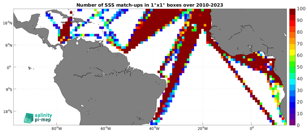
Figure 5: Number of SSS match-ups between TSG (LEGOS-DM) SSS and the CCI SSS L4 Merged-OI v5.5 - 30-day running (ESA) SSS product for the Tropical Atlantic Ocean Pi-MEP region over 1^\circ \times 1^\circ boxes and for the full satellite product period.
