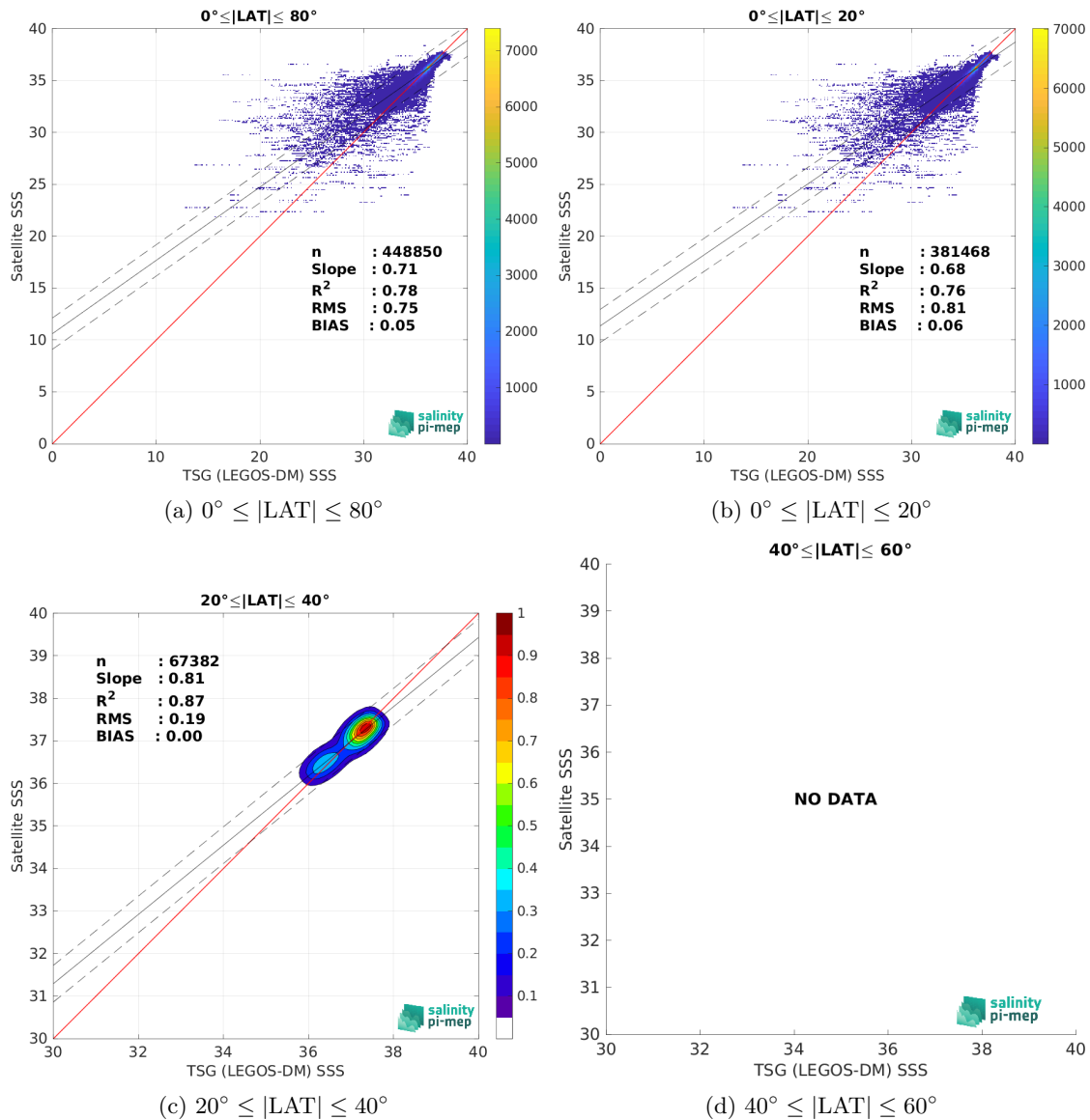
Figure 10: Contour maps of the concentration of CCI SSS L4 Merged-OI v5.5 - 30-day running (ESA) SSS (y-axis) versus TSG (LEGOS-DM) SSS (x-axis) at match-up pairs for different latitude bands. For each plot, the red line shows x=y . The black thin and dashed lines indicate a linear fit through the data cloud and the \pm 95\% confidence levels, respectively. The number match-up pairs n , the slope and R^2 coefficient of the linear fit, the root mean square (RMS) and the mean bias between satellite and in situ data are indicated for each latitude band in each plots.
