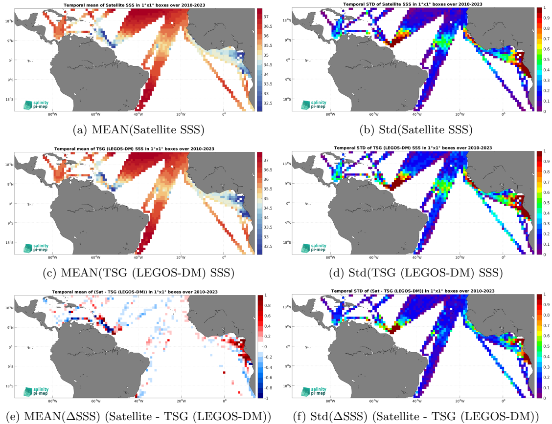
Figure 7: Temporal mean (left) and Std (right) of SSS from CCI SSS L4 Merged-OI v5.5 - 30-day running (ESA) (top), TSG (LEGOS-DM) (middle), and of \Delta SSS (Satellite - TSG (LEGOS-DM)). Only match-up pairs are used to generate these maps.
