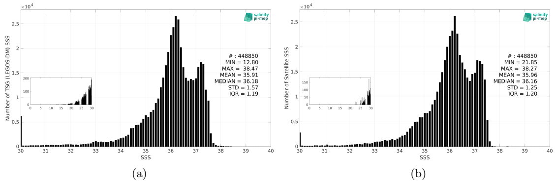
Figure 3: Histograms of SSS from TSG (LEGOS-DM) (a) and CCI SSS L4 Merged-OI v5.5 - 30-day running (ESA) (b) considering all match-up pairs per bins of 0.1 over the Tropical Atlantic Ocean Pi-MEP region and for the full satellite product period.
