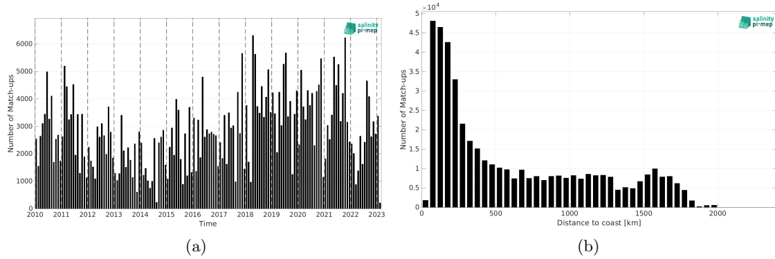
Figure 2: Number of match-ups between TSG (LEGOS-DM) and CCI SSS L4 Merged-OI v5.5 - 30-day running (ESA) SSS as a function of time (a) and as function of the distance to coast (b) over the Tropical Atlantic Ocean Pi-MEP region and for the full satellite product period.
