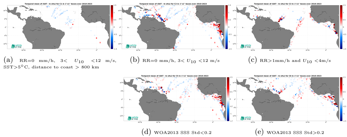
Figure 14: Temporal mean gridded over spatial boxes of size 1^\circ \times 1^\circ of \Delta\text{SSS} (CCI SSS L4 Merged-OI v5.5 - 30-day running (ESA) - TSG (LEGOS-DM)) for 5 different subdatasets corresponding to:RR=0 mm/h, 3 < U_{10} < 12 m/s, SST>5°C, distance to coast > 800 km (a), RR=0 mm/h, 3 < U_{10} < 12 m/s (b), RR>1mm/h and U_{10} < 4 m/s (c), WOA2013 SSS Std<0.2 (d), WOA2013 SSS Std>0.2 (e).
