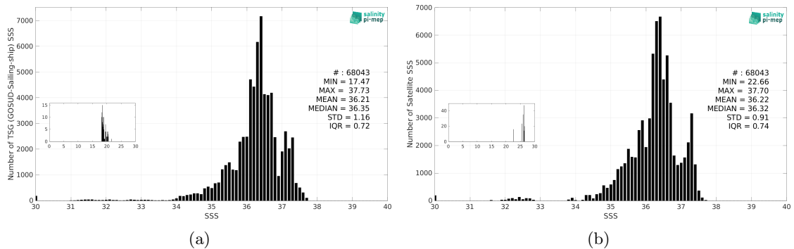
Figure 3: Histograms of SSS from TSG (GOSUD-Sailing-ship) (a) and CCI SSS L4 Merged-OI v5.5 - 30-day running (ESA) (b) considering all match-up pairs per bins of 0.1 over the Tropical Atlantic Ocean Pi-MEP region and for the full satellite product period.
