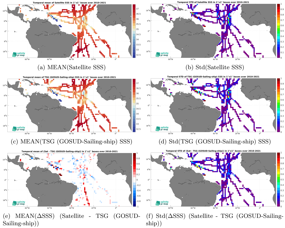
Figure 7: Temporal mean (left) and Std (right) of SSS from CCI SSS L4 Merged-OI v5.5 - 30-day running (ESA) (top), TSG (GOSUD-Sailing-ship) (middle), and of \Delta SSS (Satellite - TSG (GOSUD-Sailing-ship)). Only match-up pairs are used to generate these maps.
