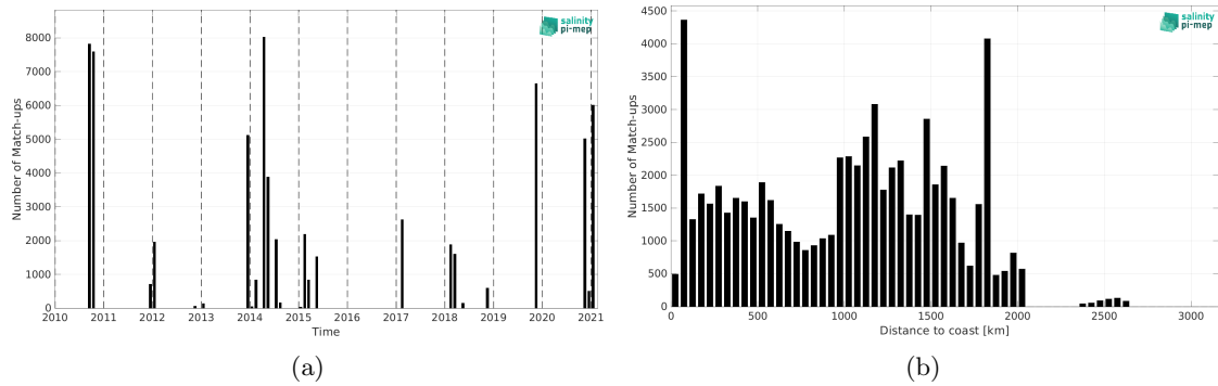
Figure 2: Number of match-ups between TSG (GOSUD-Sailing-ship) and CCI SSS L4 Merged-OI v5.5 - 30-day running (ESA) SSS as a function of time (a) and as function of the distance to coast (b) over the Tropical Atlantic Ocean Pi-MEP region and for the full satellite product period.
