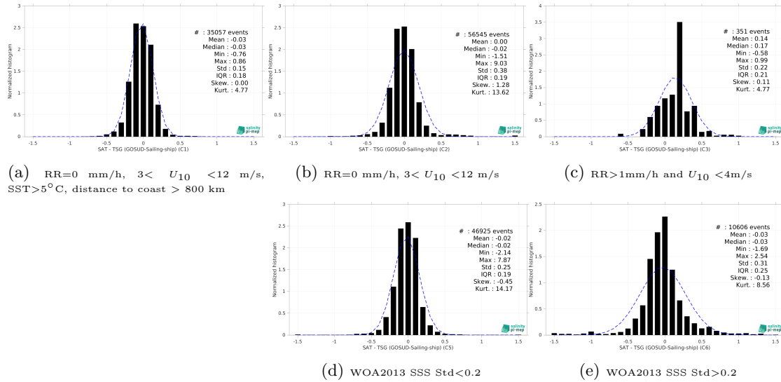
Figure 15: Normalized histogram of \Delta SSS (CCI SSS L4 Merged-OI v5.5 - 30-day running (ESA) - TSG (GOSUD-Sailing-ship)) for 5 different subdatasets corresponding to: RR=0 mm/h, 3 < U_{10} < 12 m/s, SST>5°C, distance to coast > 800 km (a), RR=0 mm/h, 3 < U_{10} < 12 m/s (b), RR>1mm/h and U_{10} < 4 m/s (c), WOA2013 SSS Std<0.2 (d), WOA2013 SSS Std>0.2 (e).
