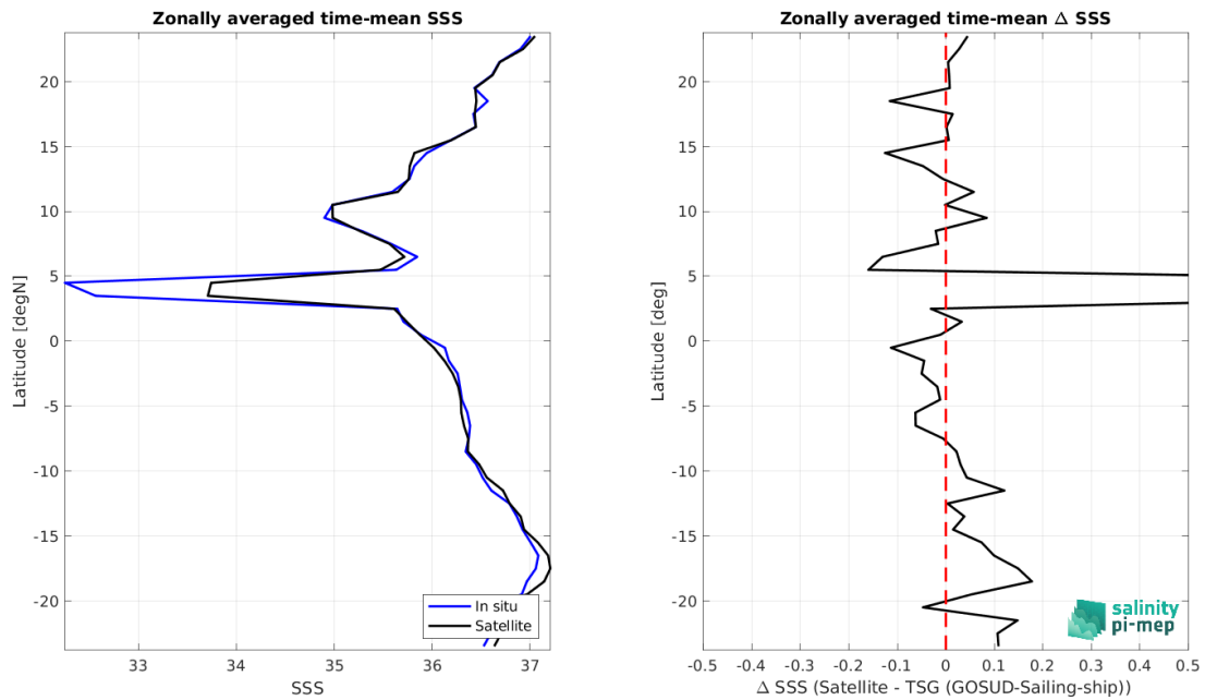
Figure 9: Left panel: Zonal mean SSS from CCI SSS L4 Merged-OI v5.5 - 30-day running (ESA) satellite product (black) and from TSG (GOSUD-Sailing-ship) (blue). Right panel: Zonal mean of \Delta SSS (Satellite - TSG (GOSUD-Sailing-ship)) for all the collected Pi-MEP match-up pairs estimated over the full satellite product period.
