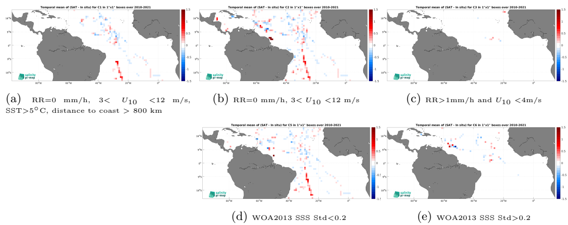
Figure 14: Temporal mean gridded over spatial boxes of size 1^\circ \times 1^\circ of \Delta\text{SSS} (CCI SSS L4 Merged-OI v5.5 - 30-day running (ESA) - TSG (GOSUD-Sailing-ship)) for 5 different subdatasets corresponding to:RR=0 mm/h, 3 < U_{10} < 12 m/s, SST >5^\circ\text{C} , distance to coast > 800 km (a), RR=0 mm/h, 3 < U_{10} < 12 m/s (b), RR >1 mm/h and U_{10} < 4 m/s (c), WOA2013 SSS Std <0.2 (d), WOA2013 SSS Std >0.2 (e).
