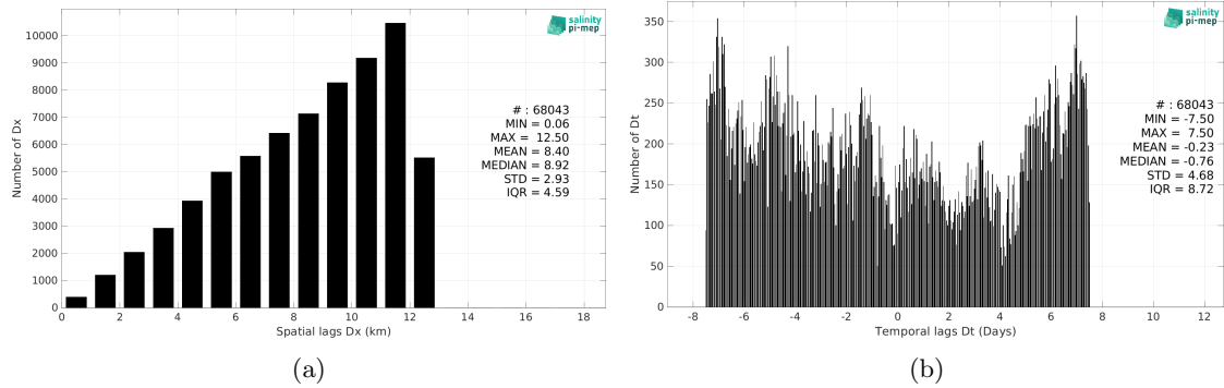
Figure 6: Histograms of the spatial (a) and temporal (b) lags between the location/time of the TSG (GOSUD-Sailing-ship) measurement and the date of the corresponding CCI SSS L4 Merged-OI v5.5 - 30-day running (ESA) SSS pixel.
