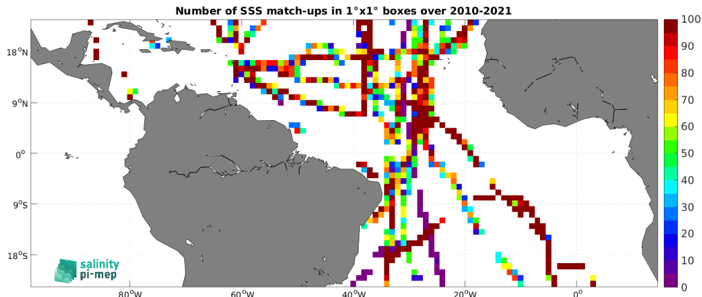
Figure 5: Number of SSS match-ups between TSG (GOSUD-Sailing-ship) SSS and the CCI SSS L4 Merged-OI v5.5 - 30-day running (ESA) SSS product for the Tropical Atlantic Ocean Pi-MEP region over 1^\circ \times 1^\circ boxes and for the full satellite product period.
