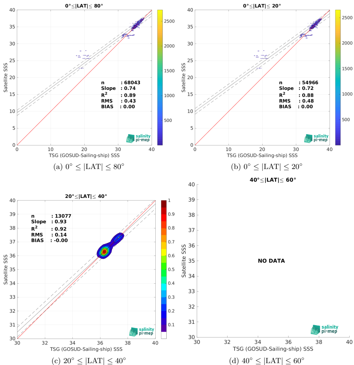
Figure 10: Contour maps of the concentration of CCI SSS L4 Merged-OI v5.5 - 30-day running (ESA) SSS (y-axis) versus TSG (GOSUD-Sailing-ship) SSS (x-axis) at match-up pairs for different latitude bands. For each plot, the red line shows x=y . The black thin and dashed lines indicate a linear fit through the data cloud and the \pm 95\% confidence levels, respectively. The number match-up pairs n , the slope and R^2 coefficient of the linear fit, the root mean square (RMS) and the mean bias between satellite and in situ data are indicated for each latitude band in each plots.
