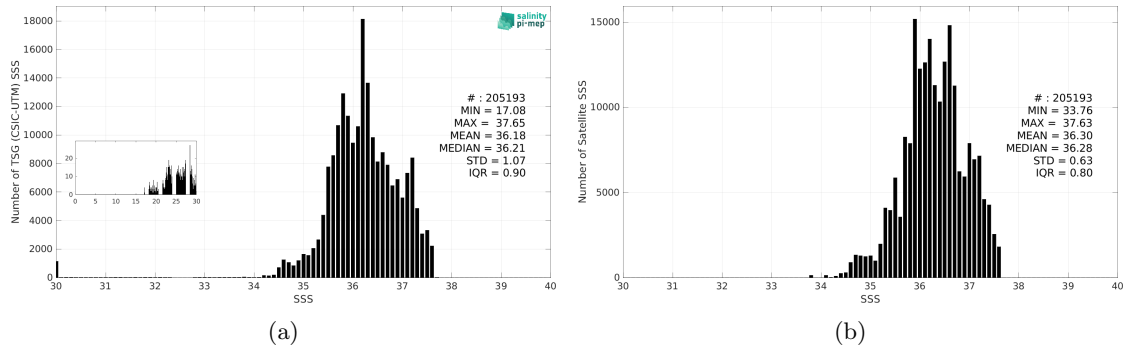
Figure 3: Histograms of SSS from TSG (CSIC-UTM) (a) and CCI SSS L4 Merged-OI v5.5 - 30-day running (ESA) (b) considering all match-up pairs per bins of 0.1 over the Tropical Atlantic Ocean Pi-MEP region and for the full satellite product period.
