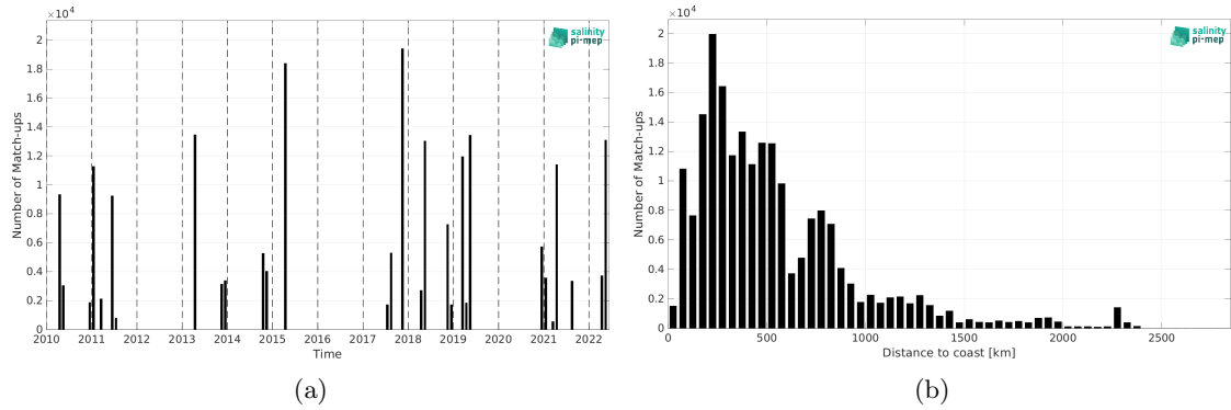
Figure 2: Number of match-ups between TSG (CSIC-UTM) and CCI SSS L4 Merged-OI v5.5 - 30-day running (ESA) SSS as a function of time (a) and as function of the distance to coast (b) over the Tropical Atlantic Ocean Pi-MEP region and for the full satellite product period.
