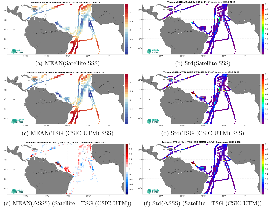
Figure 7: Temporal mean (left) and Std (right) of SSS from CCI SSS L4 Merged-OI v5.5 - 30-day running (ESA) (top), TSG (CSIC-UTM) (middle), and of \Delta SSS (Satellite - TSG (CSIC-UTM)). Only match-up pairs are used to generate these maps.
