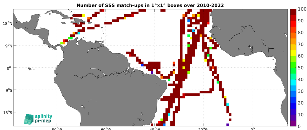
Figure 5: Number of SSS match-ups between TSG (CSIC-UTM) SSS and the CCI SSS L4 Merged-OI v5.5 - 30-day running (ESA) SSS product for the Tropical Atlantic Ocean Pi-MEP region over 1^\circ \times 1^\circ boxes and for the full satellite product period.
