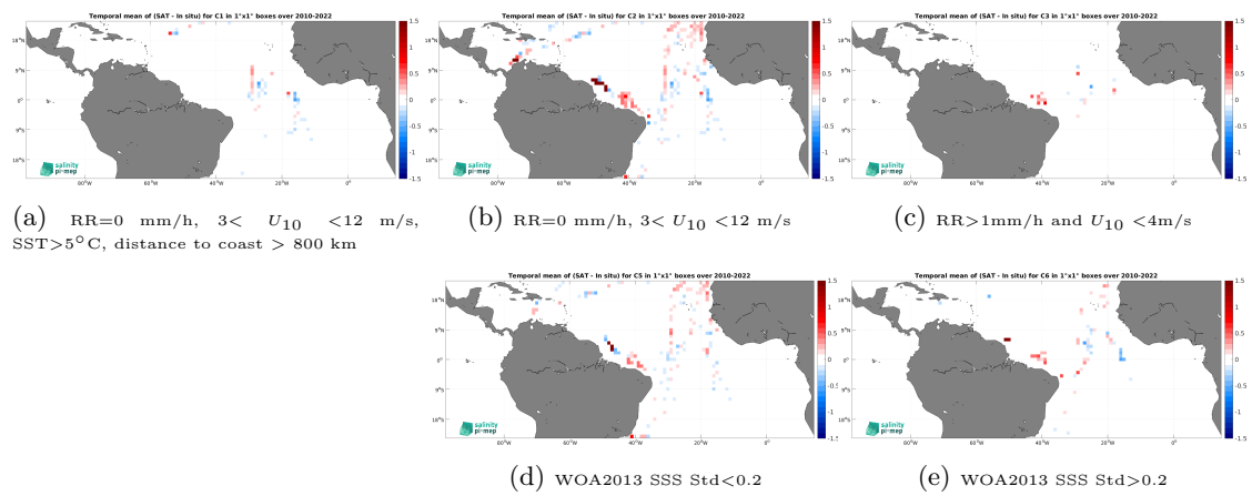
Figure 14: Temporal mean gridded over spatial boxes of size 1^\circ \times 1^\circ of \Delta\text{SSS} (CCI SSS L4 Merged-OI v5.5 - 30-day running (ESA) - TSG (CSIC-UTM)) for 5 different subdatasets corresponding to:RR=0 mm/h, 3 < U_{10} < 12 m/s, SST >5^\circ\text{C} , distance to coast > 800 km (a), RR=0 mm/h, 3 < U_{10} < 12 m/s (b), RR >1 mm/h and U_{10} < 4 m/s (c), WOA2013 SSS Std <0.2 (d), WOA2013 SSS Std >0.2 (e).
