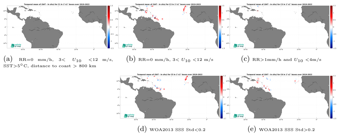
Figure 14: Temporal mean gridded over spatial boxes of size 1^\circ \times 1^\circ of \Delta\text{SSS} (CCI SSS L4 Merged-OI v5.5 - 30-day running (ESA) - Saildrone) for 5 different subdatasets corresponding to:RR=0 mm/h, 3 < U_{10} < 12 m/s, SST >5^\circ\text{C} , distance to coast > 800 km (a), RR=0 mm/h, 3 < U_{10} < 12 m/s (b), RR >1 mm/h and U_{10} < 4 m/s (c), WOA2013 SSS Std <0.2 (d), WOA2013 SSS Std >0.2 (e).
