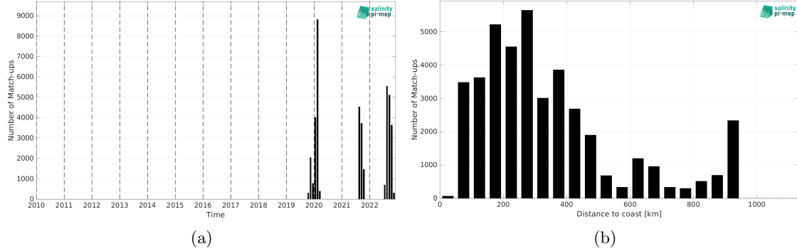
Figure 2: Number of match-ups between Saildrone and CCI SSS L4 Merged-OI v5.5 - 30-day running (ESA) SSS as a function of time (a) and as function of the distance to coast (b) over the Tropical Atlantic Ocean Pi-MEP region and for the full satellite product period.
