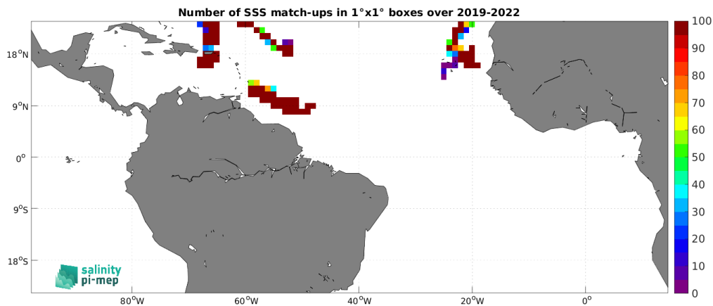
Figure 5: Number of SSS match-ups between Saildrone SSS and the CCI SSS L4 Merged-OI v5.5 - 30-day running (ESA) SSS product for the Tropical Atlantic Ocean Pi-MEP region over 1^\circ \times 1^\circ boxes and for the full satellite product period.
