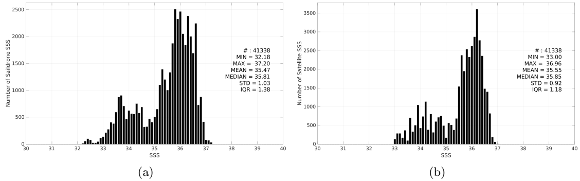
Figure 3: Histograms of SSS from Saildrone (a) and CCI SSS L4 Merged-OI v5.5 - 30-day running (ESA) (b) considering all match-up pairs per bins of 0.1 over the Tropical Atlantic Ocean Pi-MEP region and for the full satellite product period.
