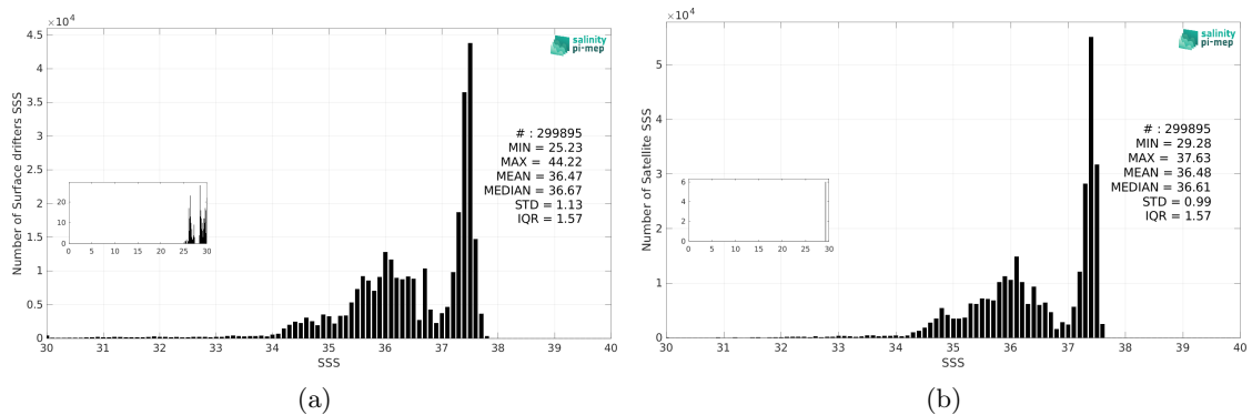
Figure 3: Histograms of SSS from Surface drifters (a) and CCI SSS L4 Merged-OI v5.5 - 30-day running (ESA) (b) considering all match-up pairs per bins of 0.1 over the Tropical Atlantic Ocean Pi-MEP region and for the full satellite product period.
