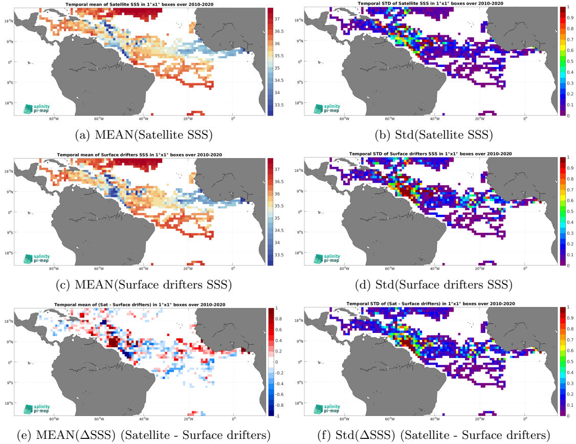
Figure 6: Temporal mean (left) and Std (right) of SSS from CCI SSS L4 Merged-OI v5.5 - 30-day running (ESA) (top), Surface drifters (middle), and of \Delta SSS (Satellite - Surface drifters). Only match-up pairs are used to generate these maps.
