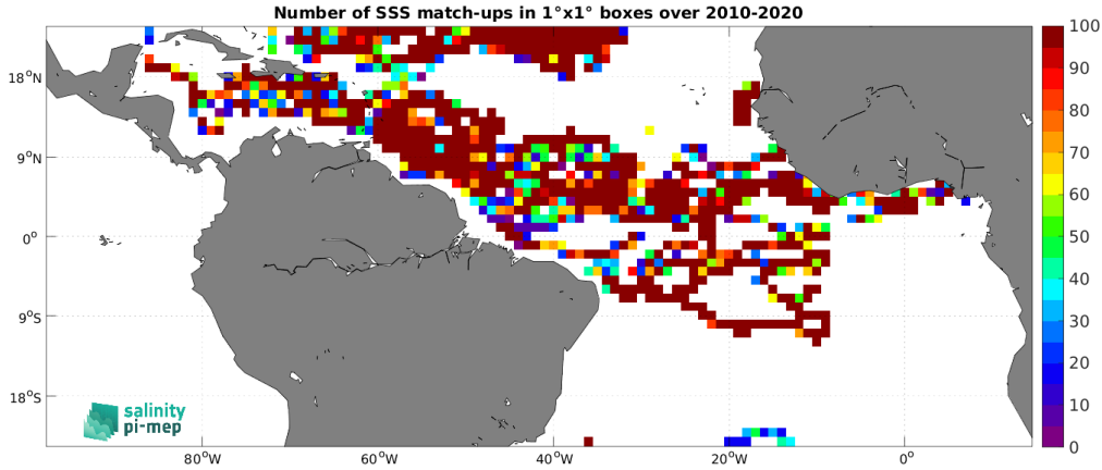
Figure 4: Number of SSS match-ups between Surface drifters SSS and the CCI SSS L4 Merged-OI v5.5 - 30-day running (ESA) SSS product for the Tropical Atlantic Ocean Pi-MEP region over 1^\circ \times 1^\circ boxes and for the full satellite product period.
