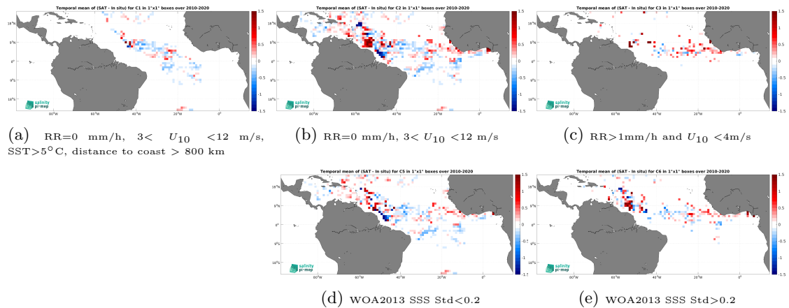
Figure 13: Temporal mean gridded over spatial boxes of size 1^\circ \times 1^\circ of \Delta\text{SSS} (CCI SSS L4 Merged-OI v5.5 - 30-day running (ESA) - Surface drifters) for 5 different subdatasets corresponding to:RR=0 mm/h, 3 < U_{10} < 12 m/s, SST >5^\circ\text{C} , distance to coast > 800 km (a), RR=0 mm/h, 3 < U_{10} < 12 m/s (b), RR >1 mm/h and U_{10} < 4 m/s (c), WOA2013 SSS Std <0.2 (d), WOA2013 SSS Std >0.2 (e).
