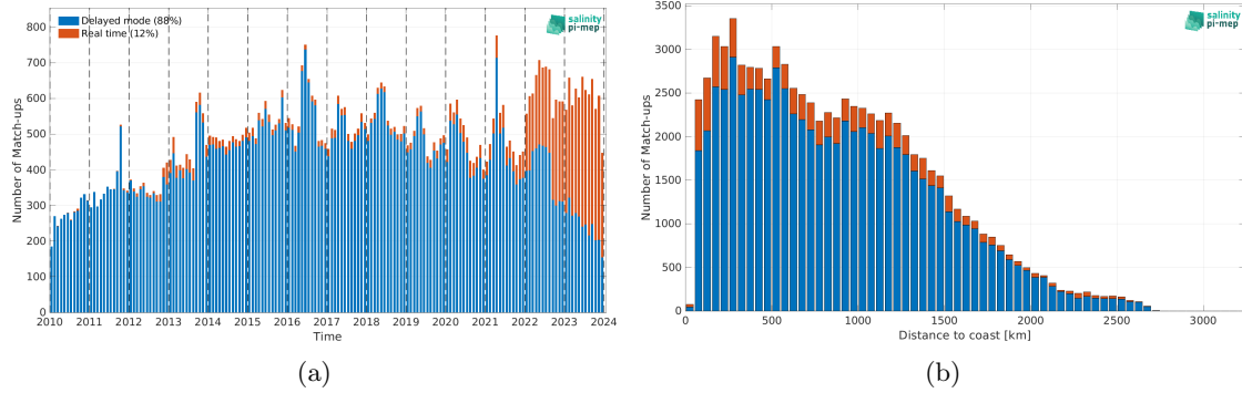
Figure 2: Number of match-ups between Argo and CCI SSS L4 Merged-OI v5.5 - 30-day running (ESA) SSS as a function of time (a) and as function of the distance to coast (b) over the Tropical Atlantic Ocean Pi-MEP region and for the full satellite product period.
