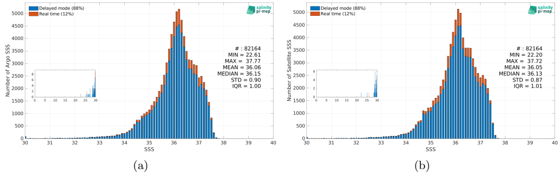
Figure 3: Histograms of SSS from Argo (a) and CCI SSS L4 Merged-OI v5.5 - 30-day running (ESA) (b) considering all match-up pairs per bins of 0.1 over the Tropical Atlantic Ocean Pi-MEP region and for the full satellite product period.
