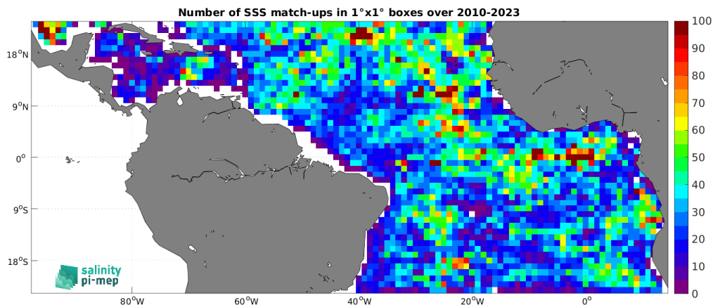
Figure 5: Number of SSS match-ups between Argo SSS and the CCI SSS L4 Merged-OI v5.5 - 30-day running (ESA) SSS product for the Tropical Atlantic Ocean Pi-MEP region over 1^\circ \times 1^\circ boxes and for the full satellite product period.
