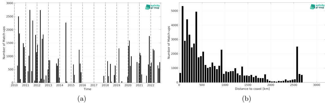
Figure 2: Number of match-ups between TSG (SAMOS) and CCI SSS L4 Merged-OI v4.41 - 7-day running (ESA) SSS as a function of time (a) and as function of the distance to coast (b) over the Tropical Atlantic Ocean Pi-MEP region and for the full satellite product period.
