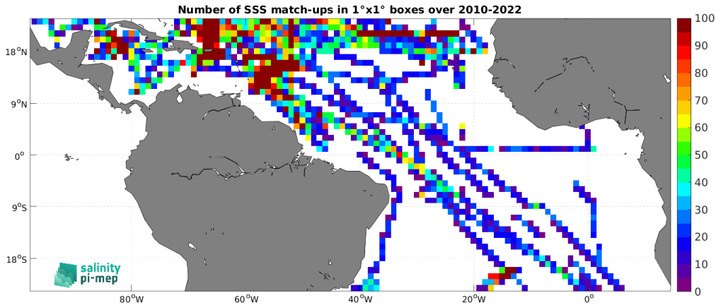
Figure 5: Number of SSS match-ups between TSG (SAMOS) SSS and the CCI SSS L4 Merged-OI v4.41 - 7-day running (ESA) SSS product for the Tropical Atlantic Ocean Pi-MEP region over 1^\circ \times 1^\circ boxes and for the full satellite product period.
