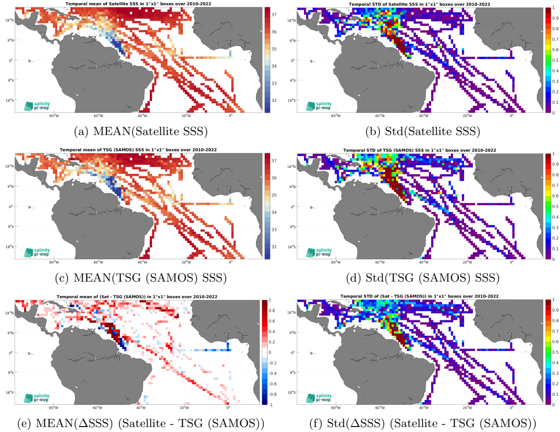
Figure 7: Temporal mean (left) and Std (right) of SSS from CCI SSS L4 Merged-OI v4.41 - 7-day running (ESA) (top), TSG (SAMOS) (middle), and of \Delta\text{SSS} (Satellite - TSG (SAMOS)). Only match-up pairs are used to generate these maps.
