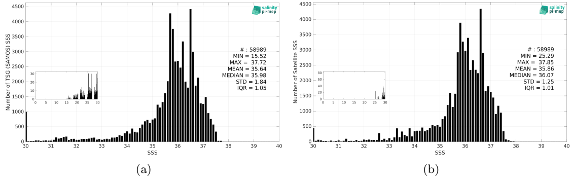
Figure 3: Histograms of SSS from TSG (SAMOS) (a) and CCI SSS L4 Merged-OI v4.41 - 7-day running (ESA) (b) considering all match-up pairs per bins of 0.1 over the Tropical Atlantic Ocean Pi-MEP region and for the full satellite product period.
