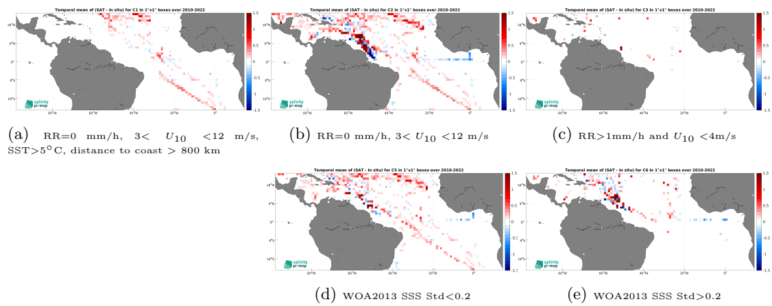
Figure 14: Temporal mean gridded over spatial boxes of size 1^\circ \times 1^\circ of \Delta\text{SSS} (CCI SSS L4 Merged-OI v4.41 - 7-day running (ESA) - TSG (SAMOS)) for 5 different subdatasets corresponding to:RR=0 mm/h, 3 < U_{10} < 12 m/s, SST>5°C, distance to coast > 800 km (a), RR=0 mm/h, 3 < U_{10} < 12 m/s (b), RR>1mm/h and U_{10} < 4 m/s (c), WOA2013 SSS Std<0.2 (d), WOA2013 SSS Std>0.2 (e).
