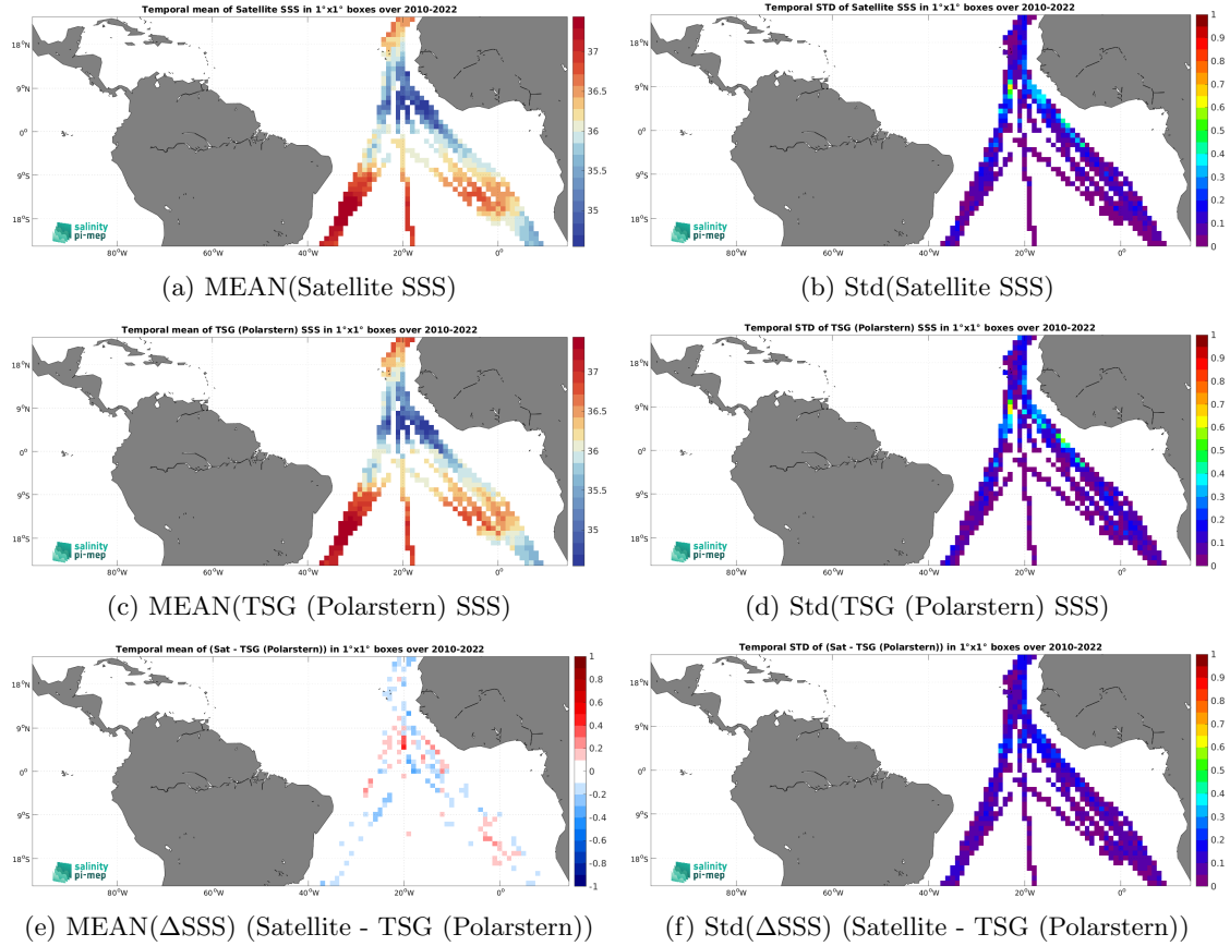
Figure 7: Temporal mean (left) and Std (right) of SSS from CCI SSS L4 Merged-OI v4.41 - 7-day running (ESA) (top), TSG (Polarstern) (middle), and of \Delta\text{SSS}(\text{Satellite} - \text{TSG}(\text{Polarstern})) . Only match-up pairs are used to generate these maps.
