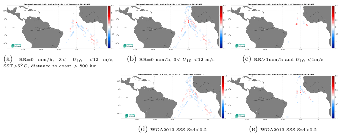
Figure 14: Temporal mean gridded over spatial boxes of size 1^\circ \times 1^\circ of \Delta\text{SSS} (CCI SSS L4 Merged-OI v4.41 - 7-day running (ESA) - TSG (Polarstern)) for 5 different subdatasets corresponding to:RR=0 mm/h, 3 < U_{10} < 12 m/s, SST >5^\circ\text{C} , distance to coast > 800 km (a), RR=0 mm/h, 3 < U_{10} < 12 m/s (b), RR >1 mm/h and U_{10} < 4 m/s (c), WOA2013 SSS Std <0.2 (d), WOA2013 SSS Std >0.2 (e).
