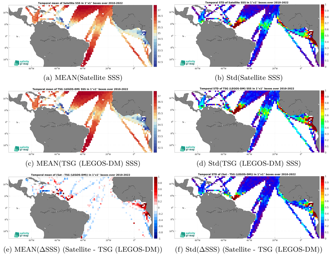
Figure 7: Temporal mean (left) and Std (right) of SSS from CCI SSS L4 Merged-OI v4.41 - 7-day running (ESA) (top), TSG (LEGOS-DM) (middle), and of \Delta\text{SSS} (Satellite - TSG (LEGOS-DM)). Only match-up pairs are used to generate these maps.
