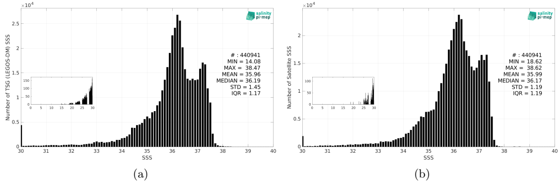
Figure 3: Histograms of SSS from TSG (LEGOS-DM) (a) and CCI SSS L4 Merged-OI v4.41 - 7-day running (ESA) (b) considering all match-up pairs per bins of 0.1 over the Tropical Atlantic Ocean Pi-MEP region and for the full satellite product period.
