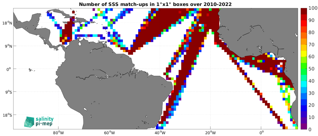
Figure 5: Number of SSS match-ups between TSG (LEGOS-DM) SSS and the CCI SSS L4 Merged-OI v4.41 - 7-day running (ESA) SSS product for the Tropical Atlantic Ocean Pi-MEP region over 1^\circ \times 1^\circ boxes and for the full satellite product period.
