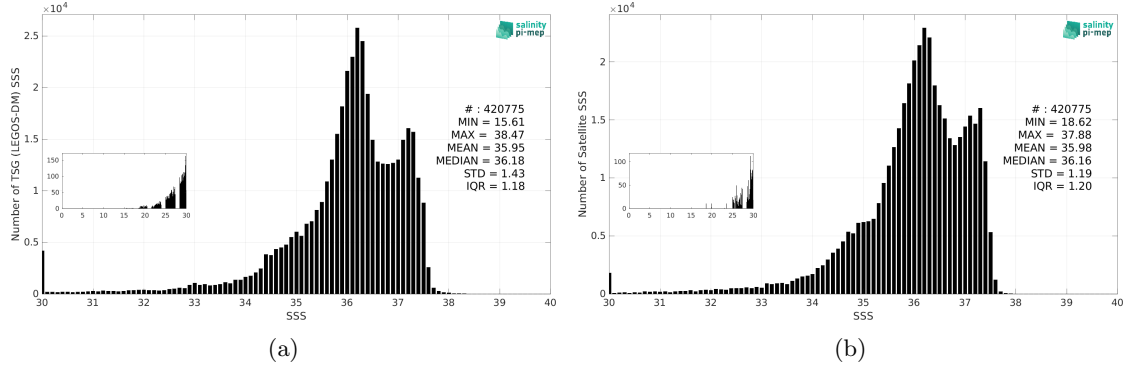
Figure 3: Histograms of SSS from TSG (LEGOS-DM) (a) and CCI SSS L4 Merged-OI v4.41 - 7-day running (ESA) (b) considering all match-up pairs per bins of 0.1 over the Tropical Atlantic Ocean Pi-MEP region and for the full satellite product period.
