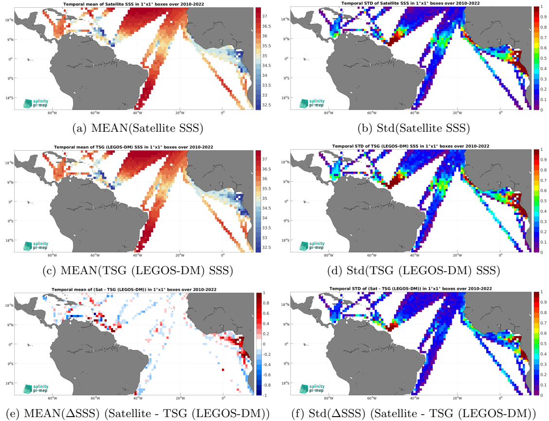
Figure 7: Temporal mean (left) and Std (right) of SSS from CCI SSS L4 Merged-OI v4.41 - 7-day running (ESA) (top), TSG (LEGOS-DM) (middle), and of \Delta\text{SSS}(\text{Satellite} - \text{TSG}(\text{LEGOS-DM})) . Only match-up pairs are used to generate these maps.
