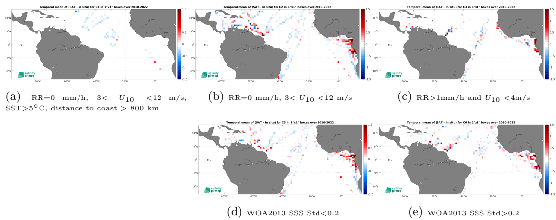
Figure 14: Temporal mean gridded over spatial boxes of size 1^\circ \times 1^\circ of \Delta\text{SSS} (CCI SSS L4 Merged-OI v4.41 - 7-day running (ESA) - TSG (LEGOS-DM)) for 5 different subdatasets corresponding to:RR=0 mm/h, 3 < U_{10} < 12 m/s, SST >5^\circ\text{C} , distance to coast > 800 km (a), RR=0 mm/h, 3 < U_{10} < 12 m/s (b), RR >1 mm/h and U_{10} < 4 m/s (c), WOA2013 SSS Std <0.2 (d), WOA2013 SSS Std >0.2 (e).
