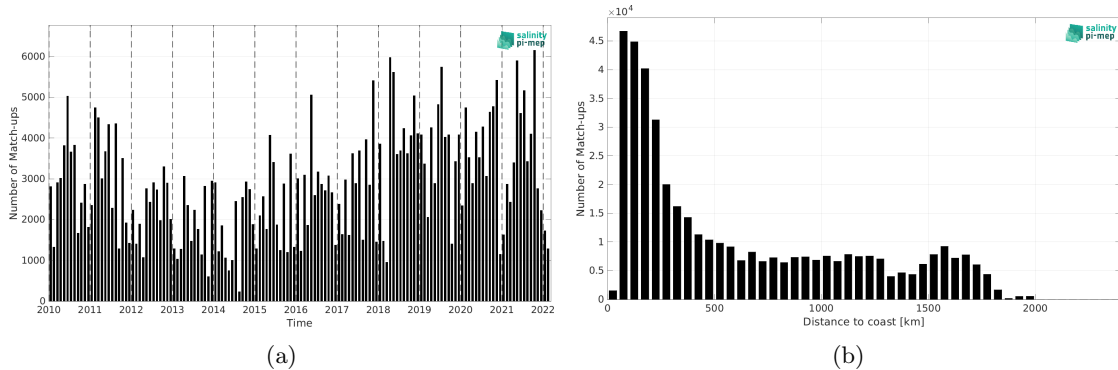
Figure 2: Number of match-ups between TSG (LEGOS-DM) and CCI SSS L4 Merged-OI v4.41 - 7-day running (ESA) SSS as a function of time (a) and as function of the distance to coast (b) over the Tropical Atlantic Ocean Pi-MEP region and for the full satellite product period.
