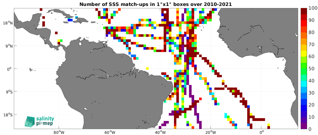
Figure 5: Number of SSS match-ups between TSG (GOSUD-Sailing-ship) SSS and the CCI SSS L4 Merged-OI v4.41 - 7-day running (ESA) SSS product for the Tropical Atlantic Ocean Pi-MEP region over 1^\circ \times 1^\circ boxes and for the full satellite product period.
