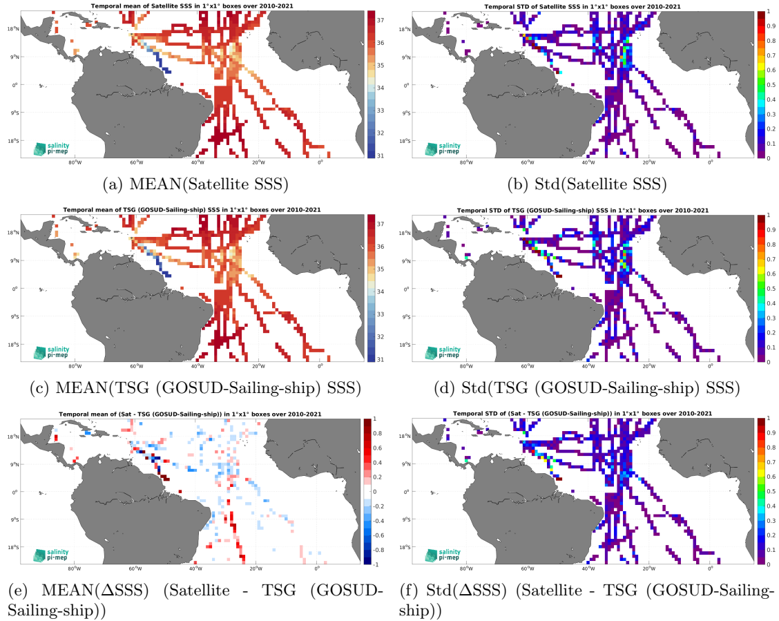
Figure 7: Temporal mean (left) and Std (right) of SSS from CCI SSS L4 Merged-OI v4.41 - 7-day running (ESA) (top), TSG (GOSUD-Sailing-ship) (middle), and of \Delta\text{SSS} (Satellite - TSG (GOSUD-Sailing-ship)). Only match-up pairs are used to generate these maps.
