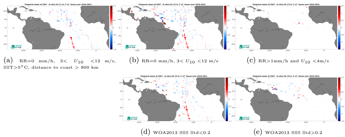
Figure 14: Temporal mean gridded over spatial boxes of size 1^\circ \times 1^\circ of \Delta\text{SSS} (CCI SSS L4 Merged-OI v4.41 - 7-day running (ESA) - TSG (GOSUD-Sailing-ship)) for 5 different subdatasets corresponding to:RR=0 mm/h, 3 < U_{10} < 12 m/s, SST >5^\circ\text{C} , distance to coast > 800 km (a), RR=0 mm/h, 3 < U_{10} < 12 m/s (b), RR >1 mm/h and U_{10} < 4 m/s (c), WOA2013 SSS Std <0.2 (d), WOA2013 SSS Std >0.2 (e).
