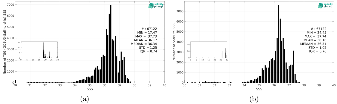
Figure 3: Histograms of SSS from TSG (GOSUD-Sailing-ship) (a) and CCI SSS L4 Merged-OI v4.41 - 7-day running (ESA) (b) considering all match-up pairs per bins of 0.1 over the Tropical Atlantic Ocean Pi-MEP region and for the full satellite product period.
