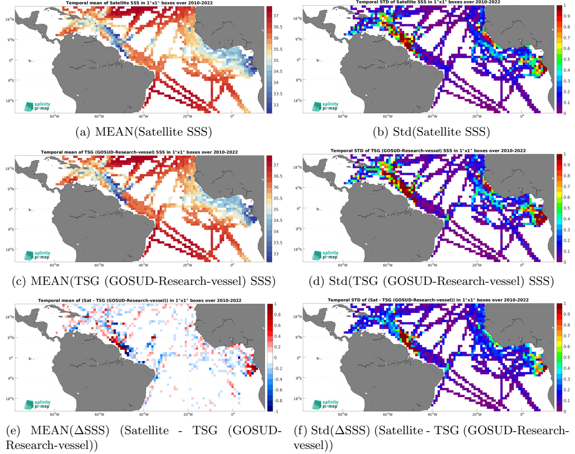
Figure 7: Temporal mean (left) and Std (right) of SSS from CCI SSS L4 Merged-OI v4.41 - 7-day running (ESA) (top), TSG (GOSUD-Research-vessel) (middle), and of \Delta\text{SSS} (Satellite - TSG (GOSUD-Research-vessel)). Only match-up pairs are used to generate these maps.
