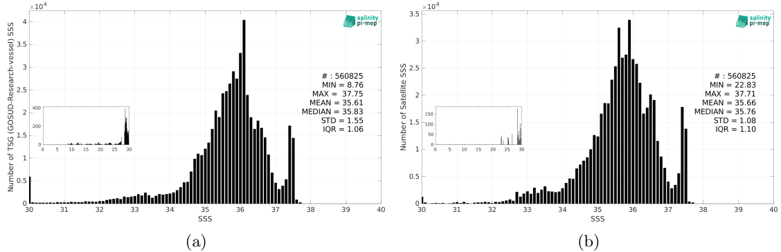
Figure 3: Histograms of SSS from TSG (GOSUD-Research-vessel) (a) and CCI SSS L4 Merged-OI v4.41 - 7-day running (ESA) (b) considering all match-up pairs per bins of 0.1 over the Tropical Atlantic Ocean Pi-MEP region and for the full satellite product period.
