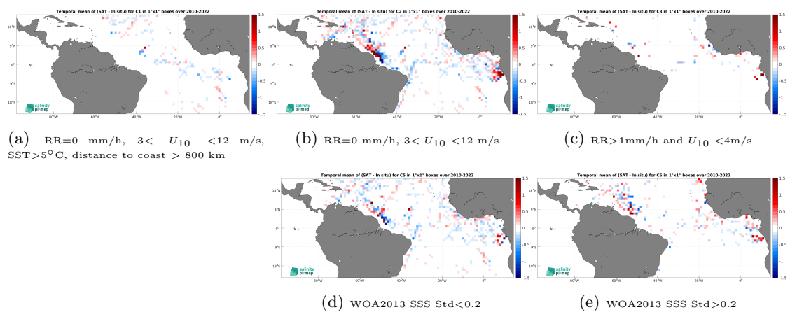
Figure 14: Temporal mean gridded over spatial boxes of size 1^\circ \times 1^\circ of \Delta\text{SSS} (CCI SSS L4 Merged-OI v4.41 - 7-day running (ESA) - TSG (GOSUD-Research-vessel)) for 5 different subdatasets corresponding to:RR=0 mm/h, 3 < U_{10} < 12 m/s, SST >5^\circ\text{C} , distance to coast > 800 km (a), RR=0 mm/h, 3 < U_{10} < 12 m/s (b), RR >1 mm/h and U_{10} < 4 m/s (c), WOA2013 SSS Std <0.2 (d), WOA2013 SSS Std >0.2 (e).
