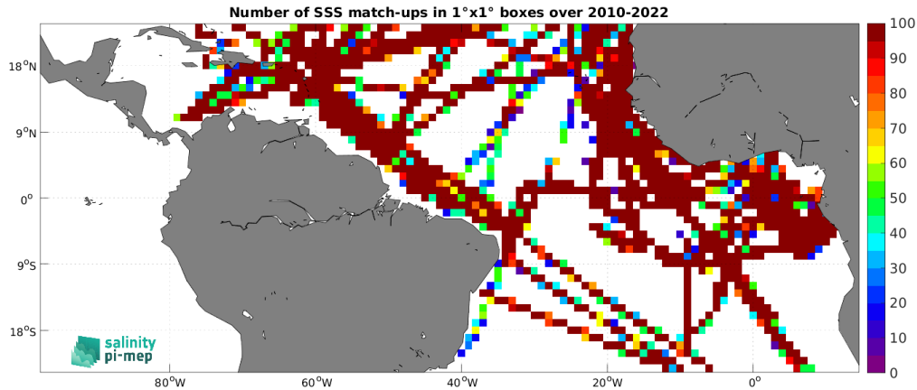
Figure 5: Number of SSS match-ups between TSG (GOSUD-Research-vessel) SSS and the CCI SSS L4 Merged-OI v4.41 - 7-day running (ESA) SSS product for the Tropical Atlantic Ocean Pi-MEP region over 1^\circ \times 1^\circ boxes and for the full satellite product period.
