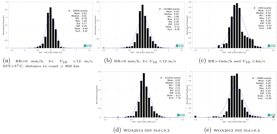
Figure 15: Normalized histogram of \Delta\text{SSS} (CCI SSS L4 Merged-OI v4.41 - 7-day running (ESA) - TSG (CSIC-UTM)) for 5 different subdatasets corresponding to: RR=0 mm/h, 3 < U_{10} < 12 m/s, SST>5°C, distance to coast > 800 km (a), RR=0 mm/h, 3 < U_{10} < 12 m/s (b), RR>1mm/h and U_{10} < 4 m/s (c), WOA2013 SSS Std<0.2 (d), WOA2013 SSS Std>0.2 (e).
