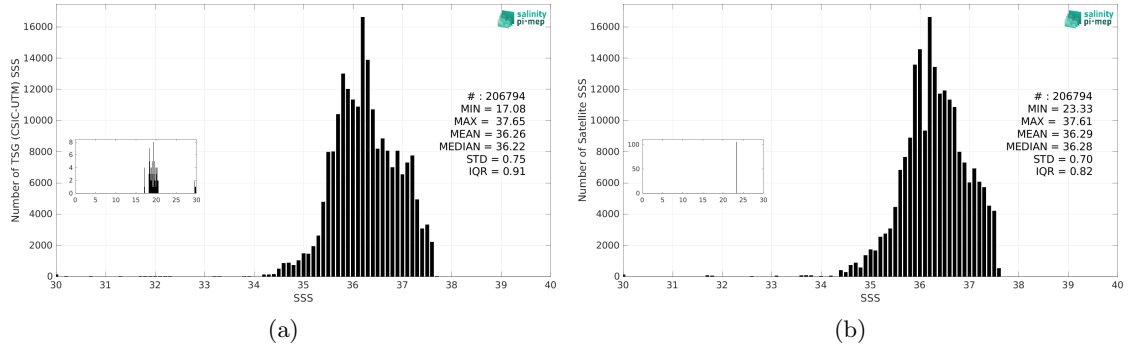
Figure 3: Histograms of SSS from TSG (CSIC-UTM) (a) and CCI SSS L4 Merged-OI v4.41 - 7-day running (ESA) (b) considering all match-up pairs per bins of 0.1 over the Tropical Atlantic Ocean Pi-MEP region and for the full satellite product period.
