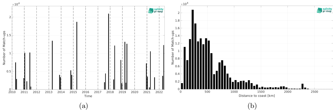
Figure 2: Number of match-ups between TSG (CSIC-UTM) and CCI SSS L4 Merged-OI v4.41 - 7-day running (ESA) SSS as a function of time (a) and as function of the distance to coast (b) over the Tropical Atlantic Ocean Pi-MEP region and for the full satellite product period.
