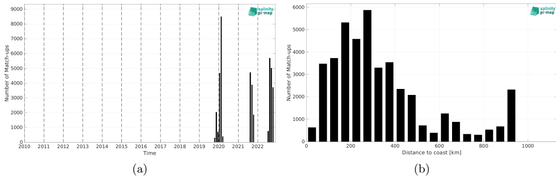
Figure 2: Number of match-ups between Saildrone and CCI SSS L4 Merged-OI v4.41 - 7-day running (ESA) SSS as a function of time (a) and as function of the distance to coast (b) over the Tropical Atlantic Ocean Pi-MEP region and for the full satellite product period.
