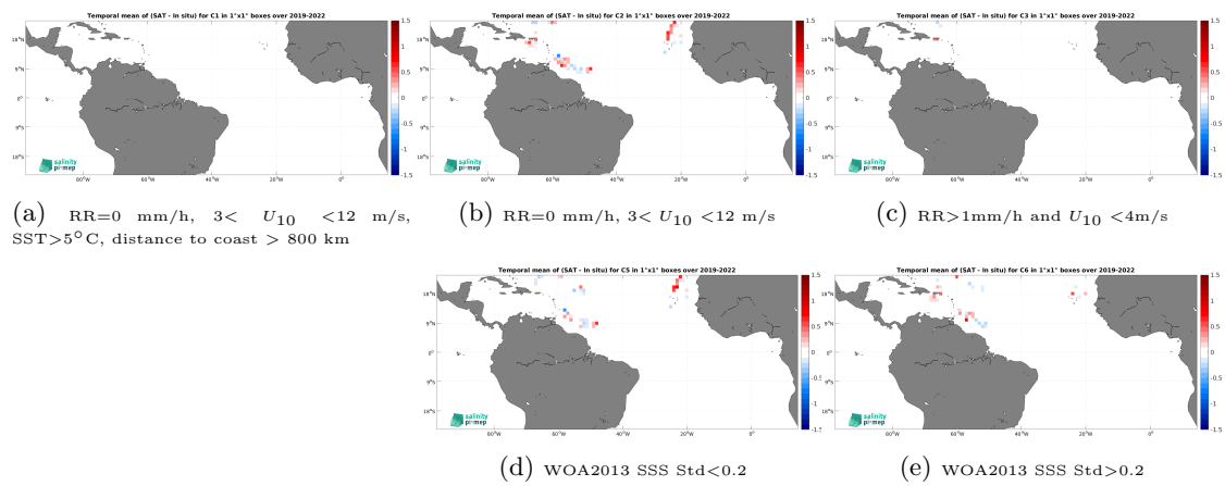
Figure 14: Temporal mean gridded over spatial boxes of size 1^\circ \times 1^\circ of \Delta\text{SSS} (CCI SSS L4 Merged-OI v4.41 - 7-day running (ESA) - Saildrone) for 5 different subdatasets corresponding to:RR=0 mm/h, 3 < U_{10} < 12 m/s, SST >5^\circ\text{C} , distance to coast > 800 km (a), RR=0 mm/h, 3 < U_{10} < 12 m/s (b), RR >1 mm/h and U_{10} < 4 m/s (c), WOA2013 SSS Std <0.2 (d), WOA2013 SSS Std >0.2 (e).
