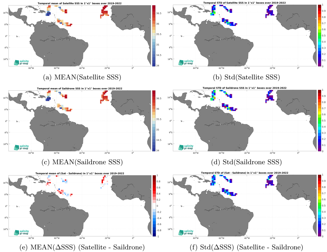
Figure 7: Temporal mean (left) and Std (right) of SSS from CCI SSS L4 Merged-OI v4.41 - 7-day running (ESA) (top), Saildrone (middle), and of \Delta\text{SSS} (Satellite - Saildrone). Only match-up pairs are used to generate these maps.
