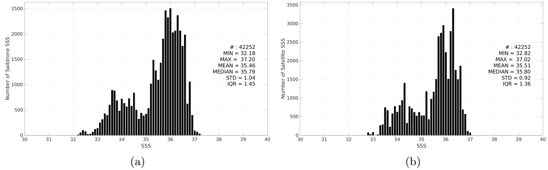
Figure 3: Histograms of SSS from Saildrone (a) and CCI SSS L4 Merged-OI v4.41 - 7-day running (ESA) (b) considering all match-up pairs per bins of 0.1 over the Tropical Atlantic Ocean Pi-MEP region and for the full satellite product period.
