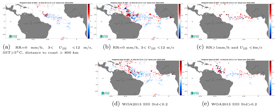
Figure 13: Temporal mean gridded over spatial boxes of size 1^\circ \times 1^\circ of \Delta\text{SSS} (CCI SSS L4 Merged-OI v4.41 - 7-day running (ESA) - Surface drifters) for 5 different subdatasets corresponding to:RR=0 mm/h, 3 < U_{10} < 12 m/s, SST >5^\circ\text{C} , distance to coast > 800 km (a), RR=0 mm/h, 3 < U_{10} < 12 m/s (b), RR >1 mm/h and U_{10} < 4 m/s (c), WOA2013 SSS Std <0.2 (d), WOA2013 SSS Std >0.2 (e).
