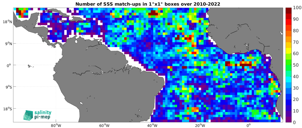
Figure 5: Number of SSS match-ups between Argo SSS and the CCI SSS L4 Merged-OI v4.41 - 7-day running (ESA) SSS product for the Tropical Atlantic Ocean Pi-MEP region over 1^\circ \times 1^\circ boxes and for the full satellite product period.
