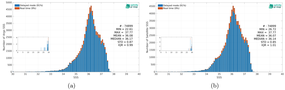
Figure 3: Histograms of SSS from Argo (a) and CCI SSS L4 Merged-OI v4.41 - 7-day running (ESA) (b) considering all match-up pairs per bins of 0.1 over the Tropical Atlantic Ocean Pi-MEP region and for the full satellite product period.
