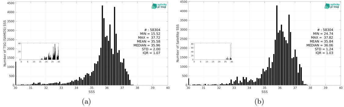
Figure 3: Histograms of SSS from TSG (SAMOS) (a) and CCI SSS L4 Merged-OI v4.41 - 30-day running (ESA) (b) considering all match-up pairs per bins of 0.1 over the Tropical Atlantic Ocean Pi-MEP region and for the full satellite product period.
