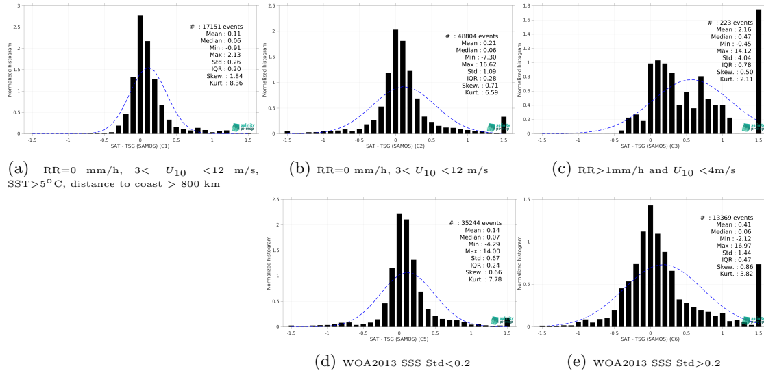
Figure 15: Normalized histogram of \Delta\text{SSS} (CCI SSS L4 Merged-OI v4.41 - 30-day running (ESA) - TSG (SAMOS)) for 5 different subdatasets corresponding to: RR=0 mm/h, 3 < U_{10} < 12 m/s, SST>5°C, distance to coast > 800 km (a), RR=0 mm/h, 3 < U_{10} < 12 m/s (b), RR>1mm/h and U_{10} < 4 m/s (c), WOA2013 SSS Std<0.2 (d), WOA2013 SSS Std>0.2 (e).
