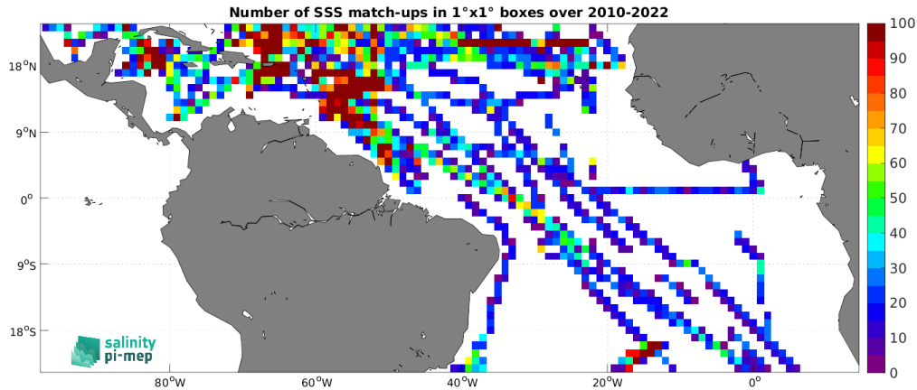
Figure 5: Number of SSS match-ups between TSG (SAMOS) SSS and the CCI SSS L4 Merged-OI v4.41 - 30-day running (ESA) SSS product for the Tropical Atlantic Ocean Pi-MEP region over 1^\circ \times 1^\circ boxes and for the full satellite product period.
