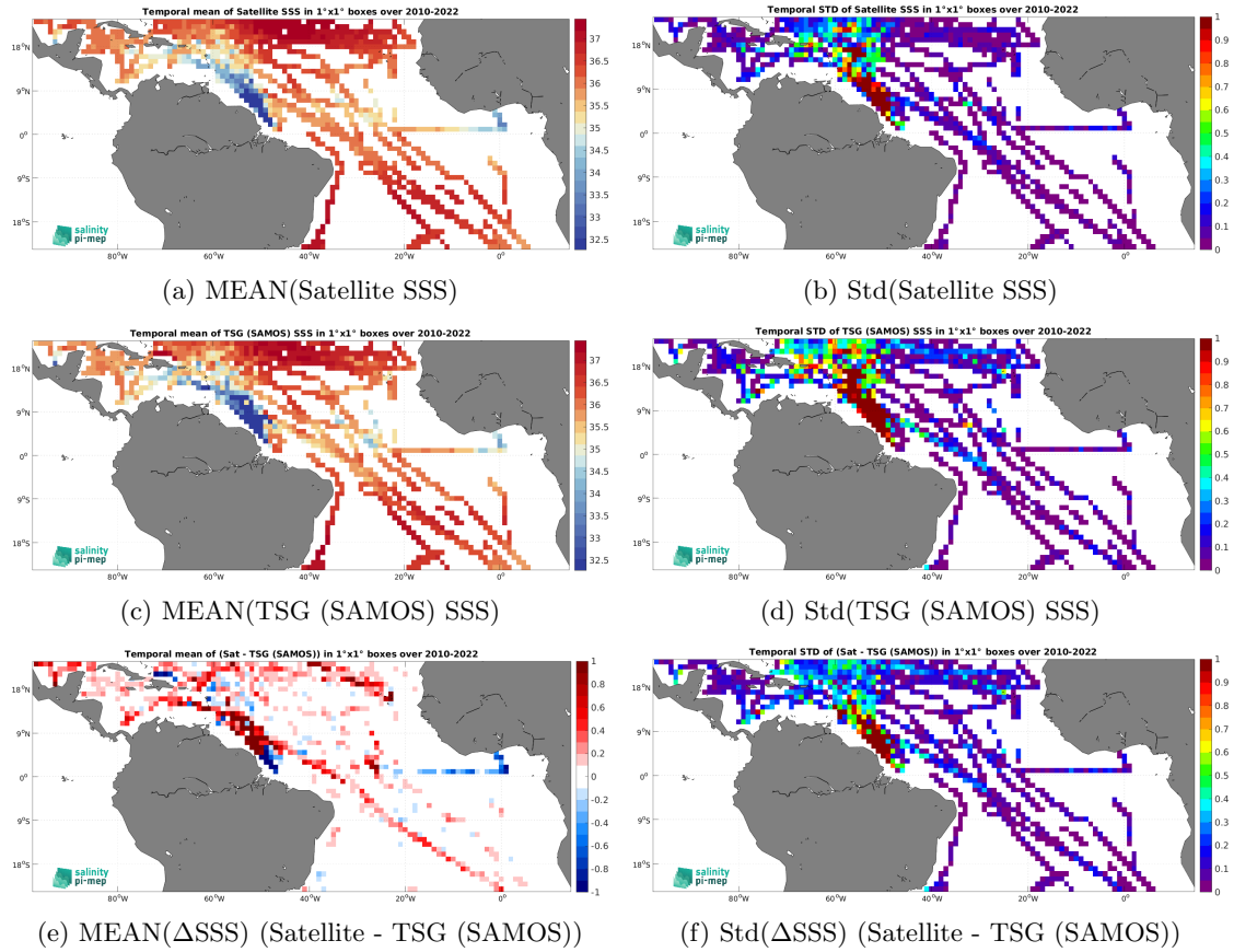
Figure 7: Temporal mean (left) and Std (right) of SSS from CCI SSS L4 Merged-OI v4.41 - 30-day running (ESA) (top), TSG (SAMOS) (middle), and of \Delta\text{SSS} (Satellite - TSG (SAMOS)). Only match-up pairs are used to generate these maps.
