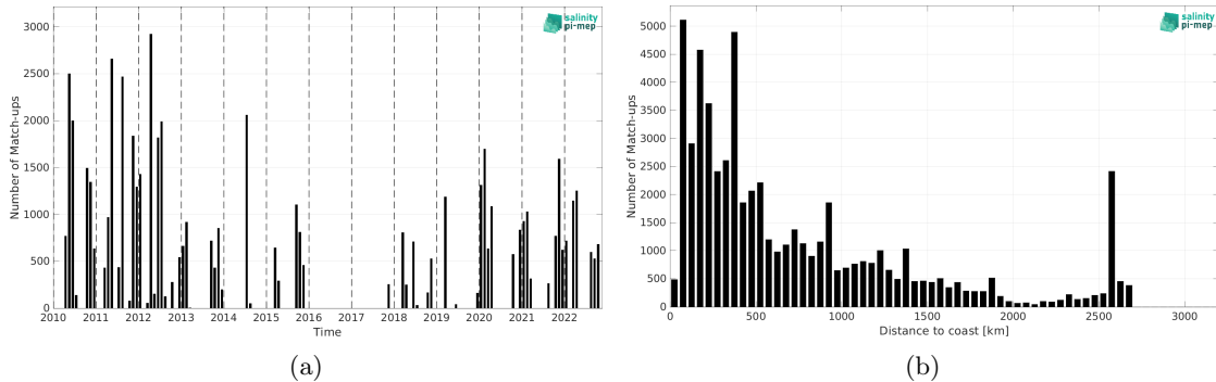
Figure 2: Number of match-ups between TSG (SAMOS) and CCI SSS L4 Merged-OI v4.41 - 30-day running (ESA) SSS as a function of time (a) and as function of the distance to coast (b) over the Tropical Atlantic Ocean Pi-MEP region and for the full satellite product period.
