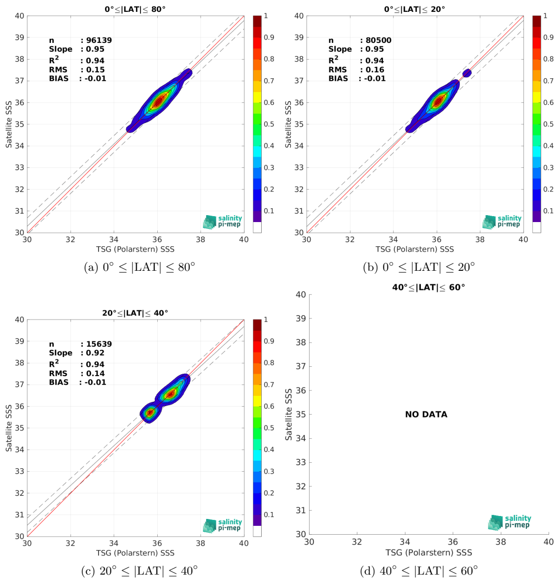
Figure 10: Contour maps of the concentration of CCI SSS L4 Merged-OI v4.41 - 30-day running (ESA) SSS (y-axis) versus TSG (Polarstern) SSS (x-axis) at match-up pairs for different latitude bands. For each plot, the red line shows x=y . The black thin and dashed lines indicate a linear fit through the data cloud and the \pm 95\% confidence levels, respectively. The number match-up pairs n , the slope and R^2 coefficient of the linear fit, the root mean square (RMS) and the mean bias between satellite and in situ data are indicated for each latitude band in each plots.
