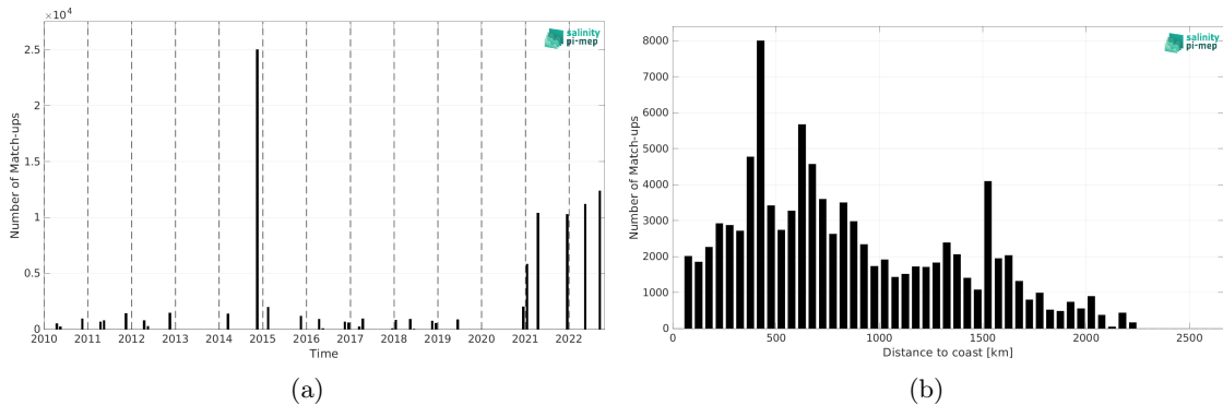
Figure 2: Number of match-ups between TSG (Polarstern) and CCI SSS L4 Merged-OI v4.41 - 30-day running (ESA) SSS as a function of time (a) and as function of the distance to coast (b) over the Tropical Atlantic Ocean Pi-MEP region and for the full satellite product period.
