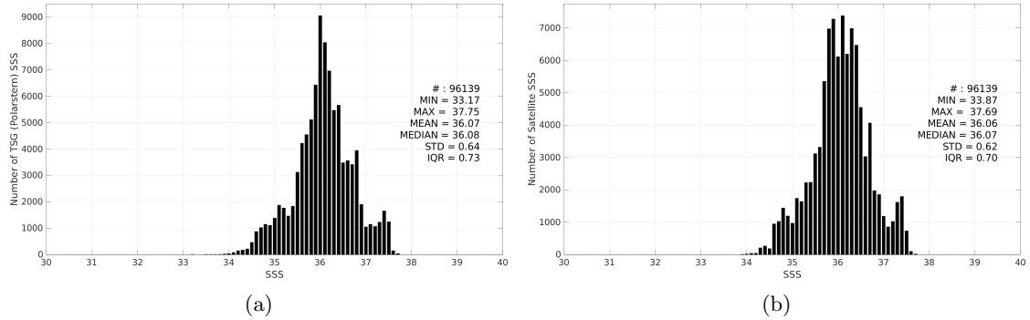
Figure 3: Histograms of SSS from TSG (Polarstern) (a) and CCI SSS L4 Merged-OI v4.41 - 30-day running (ESA) (b) considering all match-up pairs per bins of 0.1 over the Tropical Atlantic Ocean Pi-MEP region and for the full satellite product period.
