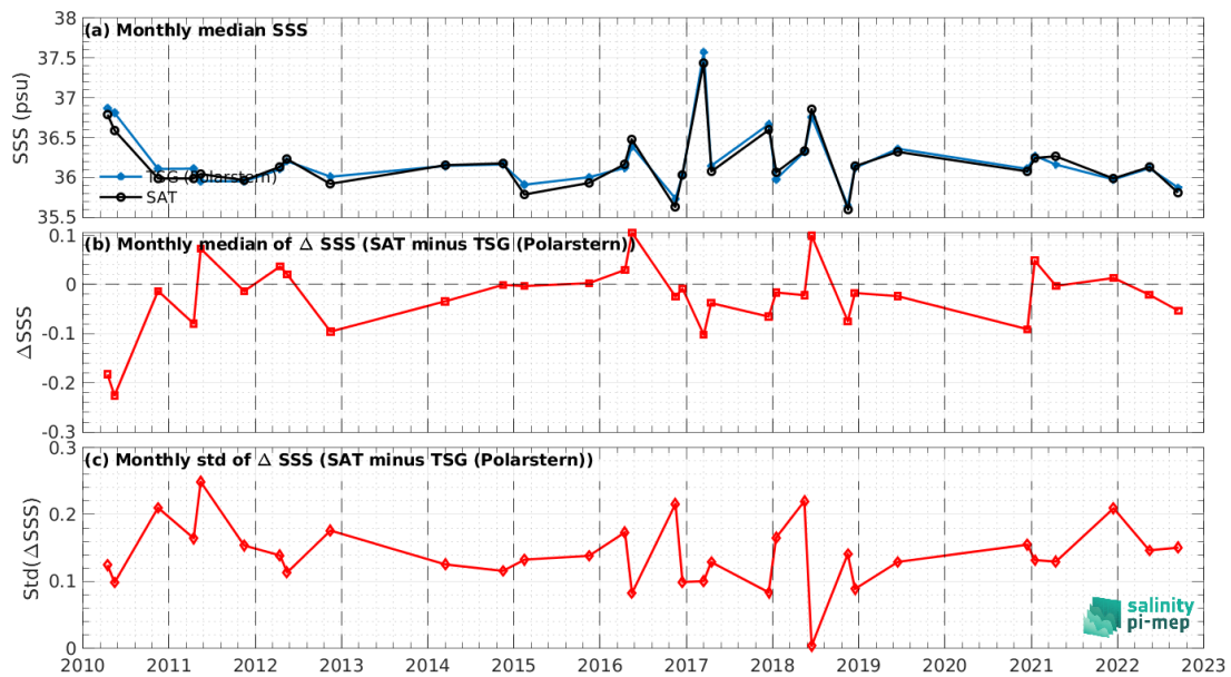
Figure 8: Time series of the monthly median SSS (top), median of \Delta\text{SSS} (Satellite - TSG (Polarstern)) and Std of \Delta\text{SSS} (Satellite - TSG (Polarstern)) over the Tropical Atlantic Ocean Pi-MEP region considering all match-ups collected by the Pi-MEP.
