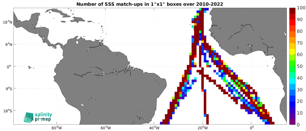
Figure 5: Number of SSS match-ups between TSG (Polarstern) SSS and the CCI SSS L4 Merged-OI v4.41 - 30-day running (ESA) SSS product for the Tropical Atlantic Ocean Pi-MEP region over 1^\circ \times 1^\circ boxes and for the full satellite product period.
