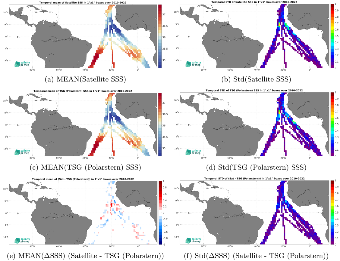
Figure 7: Temporal mean (left) and Std (right) of SSS from CCI SSS L4 Merged-OI v4.41 - 30-day running (ESA) (top), TSG (Polarstern) (middle), and of \Delta\text{SSS}(\text{Satellite} - \text{TSG}(\text{Polarstern})) . Only match-up pairs are used to generate these maps.
