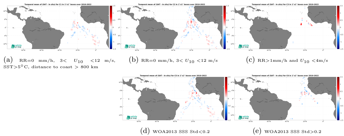
Figure 14: Temporal mean gridded over spatial boxes of size 1^\circ \times 1^\circ of \Delta\text{SSS} (CCI SSS L4 Merged-OI v4.41 - 30-day running (ESA) - TSG (Polarstern)) for 5 different subdatasets corresponding to:RR=0 mm/h, 3 < U_{10} < 12 m/s, SST >5^\circ\text{C} , distance to coast > 800 km (a), RR=0 mm/h, 3 < U_{10} < 12 m/s (b), RR >1 mm/h and U_{10} < 4 m/s (c), WOA2013 SSS Std <0.2 (d), WOA2013 SSS Std >0.2 (e).
