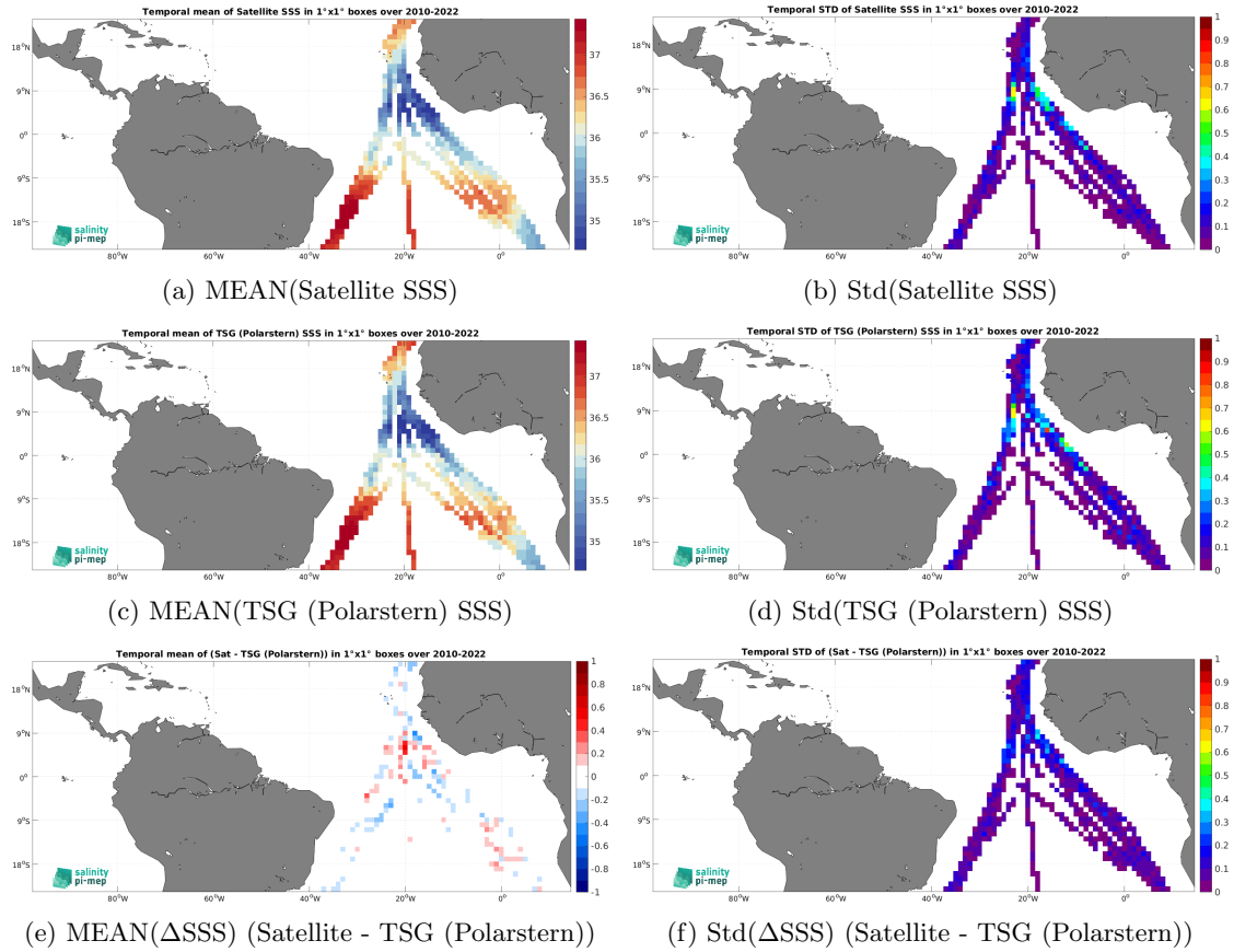
Figure 7: Temporal mean (left) and Std (right) of SSS from CCI SSS L4 Merged-OI v4.41 - 30-day running (ESA) (top), TSG (Polarstern) (middle), and of \Delta\text{SSS} (Satellite - TSG (Polarstern)). Only match-up pairs are used to generate these maps.
