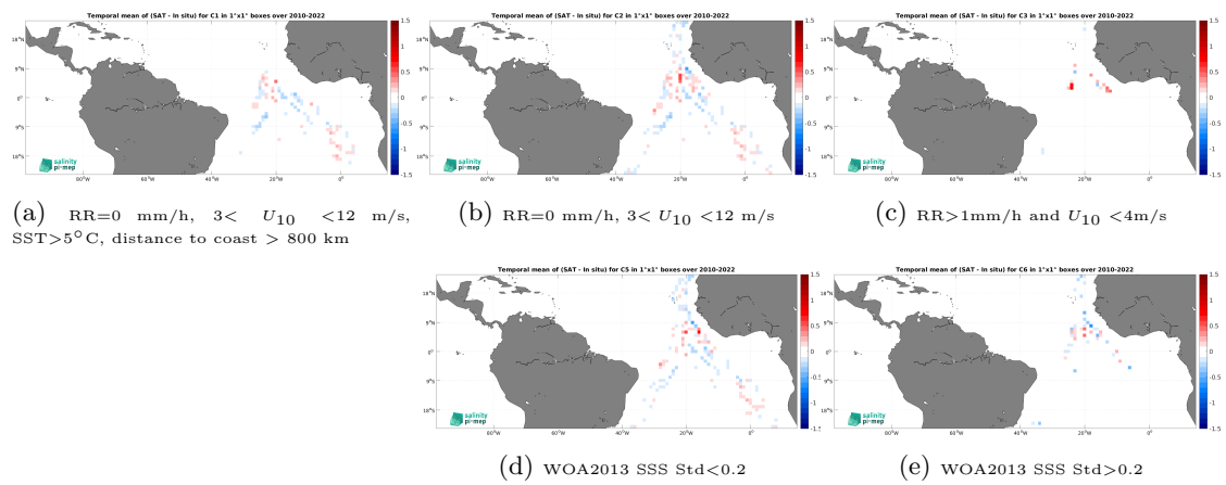
Figure 14: Temporal mean gridded over spatial boxes of size 1^\circ \times 1^\circ of \Delta\text{SSS} (CCI SSS L4 Merged-OI v4.41 - 30-day running (ESA) - TSG (Polarstern)) for 5 different subdatasets corresponding to:RR=0 mm/h, 3 < U_{10} < 12 m/s, SST >5^\circ\text{C} , distance to coast > 800 km (a), RR=0 mm/h, 3 < U_{10} < 12 m/s (b), RR >1 mm/h and U_{10} < 4 m/s (c), WOA2013 SSS Std <0.2 (d), WOA2013 SSS Std >0.2 (e).
