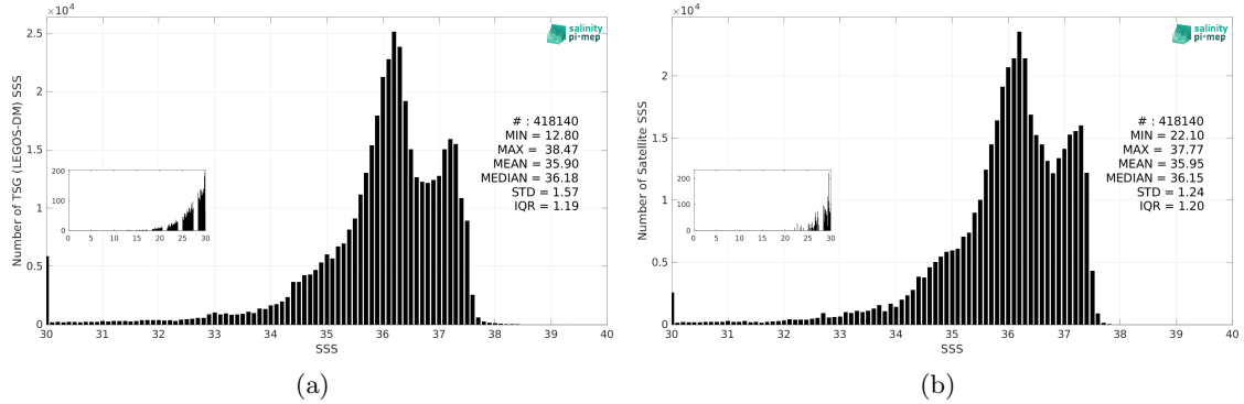
Figure 3: Histograms of SSS from TSG (LEGOS-DM) (a) and CCI SSS L4 Merged-OI v4.41 - 30-day running (ESA) (b) considering all match-up pairs per bins of 0.1 over the Tropical Atlantic Ocean Pi-MEP region and for the full satellite product period.
