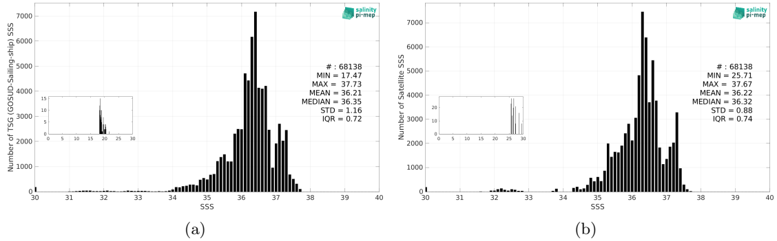
Figure 3: Histograms of SSS from TSG (GOSUD-Sailing-ship) (a) and CCI SSS L4 Merged-OI v4.41 - 30-day running (ESA) (b) considering all match-up pairs per bins of 0.1 over the Tropical Atlantic Ocean Pi-MEP region and for the full satellite product period.
