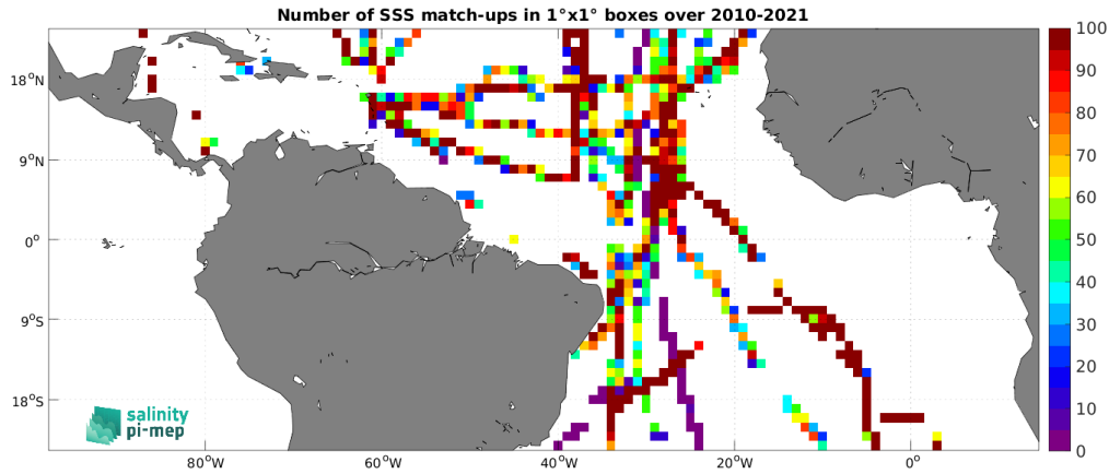
Figure 5: Number of SSS match-ups between TSG (GOSUD-Sailing-ship) SSS and the CCI SSS L4 Merged-OI v4.41 - 30-day running (ESA) SSS product for the Tropical Atlantic Ocean Pi-MEP region over 1^\circ \times 1^\circ boxes and for the full satellite product period.
