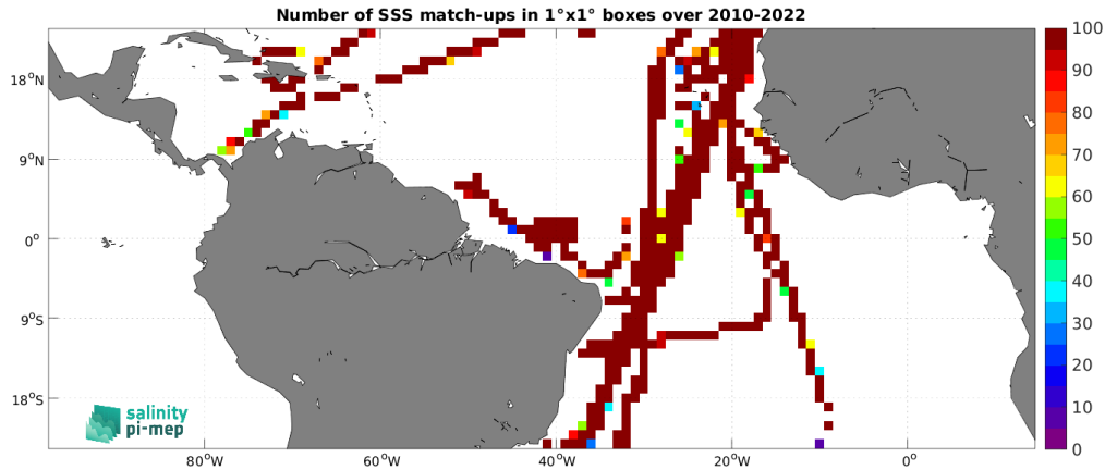
Figure 5: Number of SSS match-ups between TSG (CSIC-UTM) SSS and the CCI SSS L4 Merged-OI v4.41 - 30-day running (ESA) SSS product for the Tropical Atlantic Ocean Pi-MEP region over 1^\circ \times 1^\circ boxes and for the full satellite product period.
