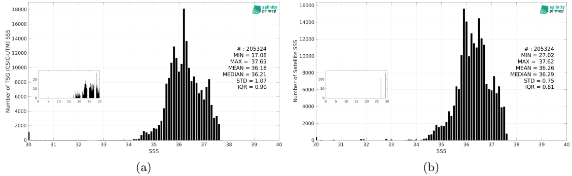
Figure 3: Histograms of SSS from TSG (CSIC-UTM) (a) and CCI SSS L4 Merged-OI v4.41 - 30-day running (ESA) (b) considering all match-up pairs per bins of 0.1 over the Tropical Atlantic Ocean Pi-MEP region and for the full satellite product period.
