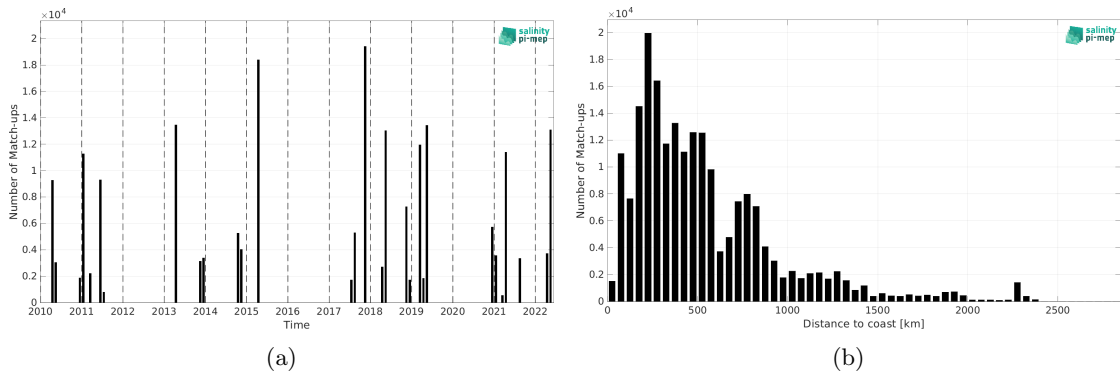
Figure 2: Number of match-ups between TSG (CSIC-UTM) and CCI SSS L4 Merged-OI v4.41 - 30-day running (ESA) SSS as a function of time (a) and as function of the distance to coast (b) over the Tropical Atlantic Ocean Pi-MEP region and for the full satellite product period.
