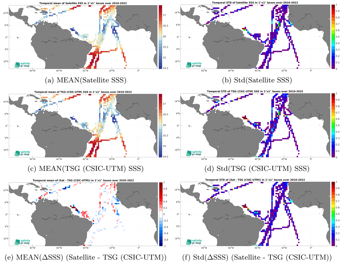
Figure 7: Temporal mean (left) and Std (right) of SSS from CCI SSS L4 Merged-OI v4.41 - 30-day running (ESA) (top), TSG (CSIC-UTM) (middle), and of \Delta\text{SSS} (Satellite - TSG (CSIC-UTM)). Only match-up pairs are used to generate these maps.
