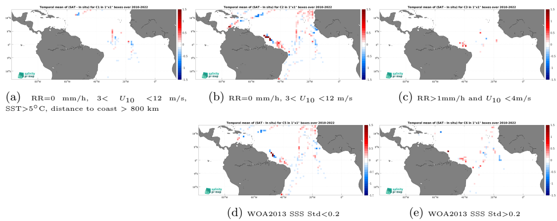
Figure 14: Temporal mean gridded over spatial boxes of size 1^\circ \times 1^\circ of \Delta\text{SSS} (CCI SSS L4 Merged-OI v4.41 - 30-day running (ESA) - TSG (CSIC-UTM)) for 5 different subdatasets corresponding to:RR=0 mm/h, 3 < U_{10} < 12 m/s, SST >5^\circ\text{C} , distance to coast > 800 km (a), RR=0 mm/h, 3 < U_{10} < 12 m/s (b), RR >1 mm/h and U_{10} < 4 m/s (c), WOA2013 SSS Std <0.2 (d), WOA2013 SSS Std >0.2 (e).
