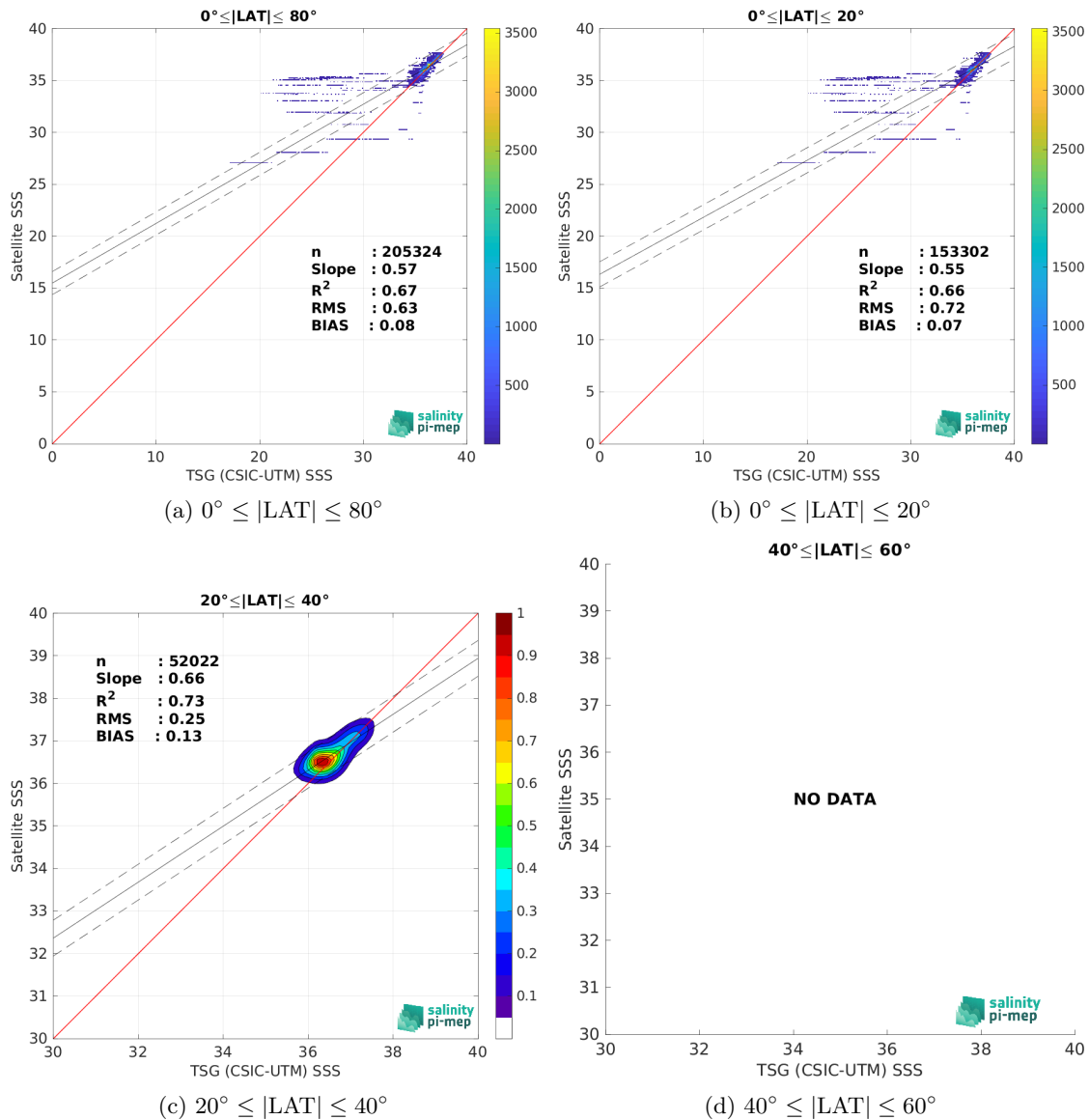
Figure 10: Contour maps of the concentration of CCI SSS L4 Merged-OI v4.41 - 30-day running (ESA) SSS (y-axis) versus TSG (CSIC-UTM) SSS (x-axis) at match-up pairs for different latitude bands. For each plot, the red line shows x=y . The black thin and dashed lines indicate a linear fit through the data cloud and the \pm 95\% confidence levels, respectively. The number match-up pairs n , the slope and R^2 coefficient of the linear fit, the root mean square (RMS) and the mean bias between satellite and in situ data are indicated for each latitude band in each plots.
