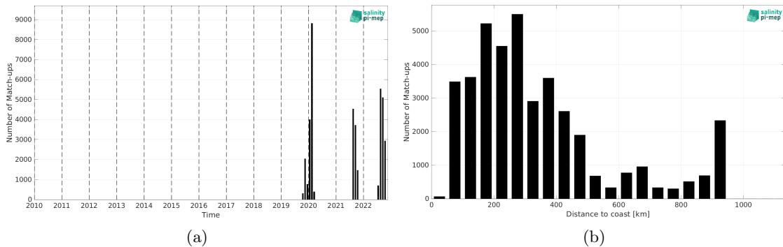
Figure 2: Number of match-ups between Saildrone and CCI SSS L4 Merged-OI v4.41 - 30-day running (ESA) SSS as a function of time (a) and as function of the distance to coast (b) over the Tropical Atlantic Ocean Pi-MEP region and for the full satellite product period.
