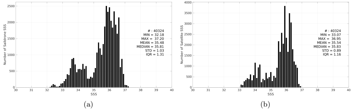
Figure 3: Histograms of SSS from Saildrone (a) and CCI SSS L4 Merged-OI v4.41 - 30-day running (ESA) (b) considering all match-up pairs per bins of 0.1 over the Tropical Atlantic Ocean Pi-MEP region and for the full satellite product period.
