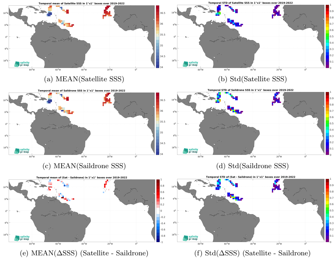
Figure 7: Temporal mean (left) and Std (right) of SSS from CCI SSS L4 Merged-OI v4.41 - 30-day running (ESA) (top), Saildrone (middle), and of \Delta\text{SSS} (Satellite - Saildrone). Only match-up pairs are used to generate these maps.
