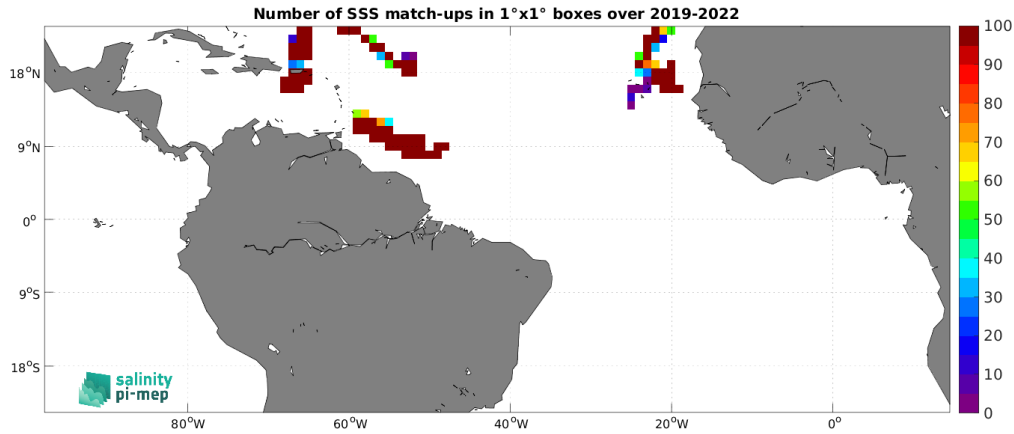
Figure 5: Number of SSS match-ups between Saildrone SSS and the CCI SSS L4 Merged-OI v4.41 - 30-day running (ESA) SSS product for the Tropical Atlantic Ocean Pi-MEP region over 1^\circ \times 1^\circ boxes and for the full satellite product period.
