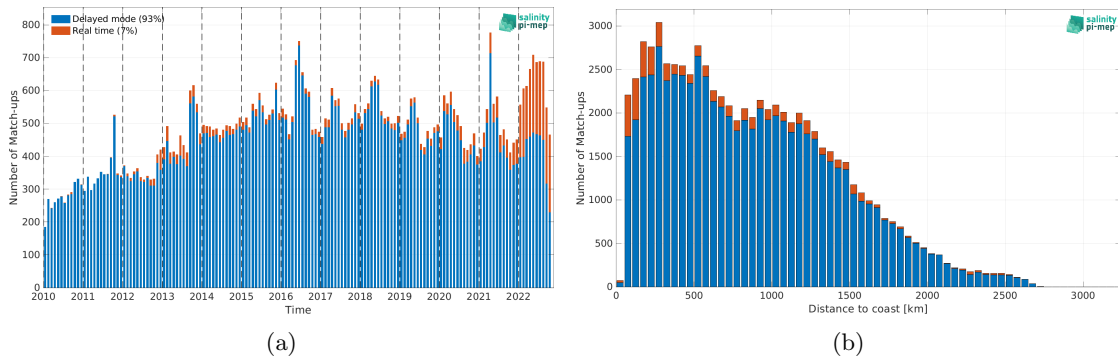
Figure 2: Number of match-ups between Argo and CCI SSS L4 Merged-OI v4.41 - 30-day running (ESA) SSS as a function of time (a) and as function of the distance to coast (b) over the Tropical Atlantic Ocean Pi-MEP region and for the full satellite product period.
