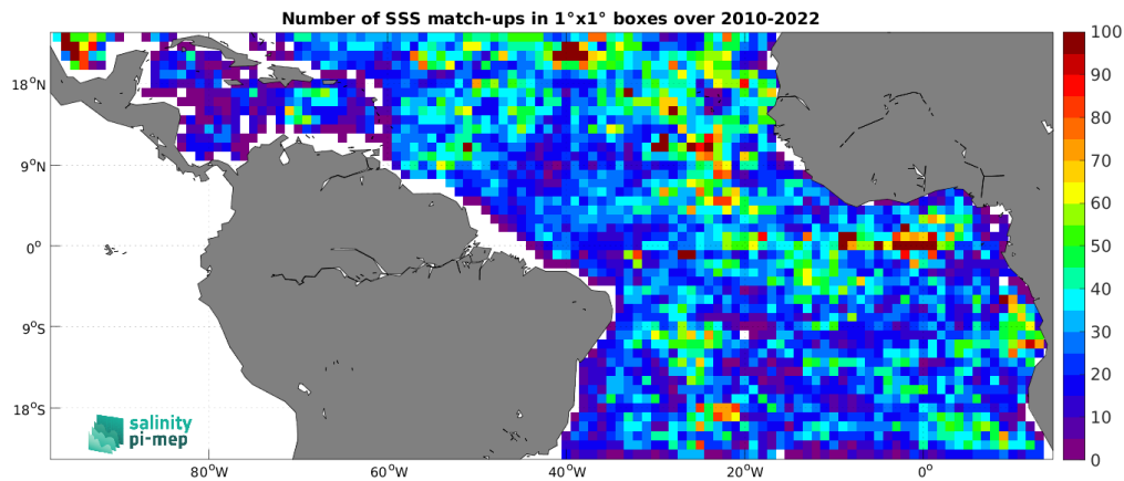
Figure 5: Number of SSS match-ups between Argo SSS and the CCI SSS L4 Merged-OI v4.41 - 30-day running (ESA) SSS product for the Tropical Atlantic Ocean Pi-MEP region over 1^\circ \times 1^\circ boxes and for the full satellite product period.
