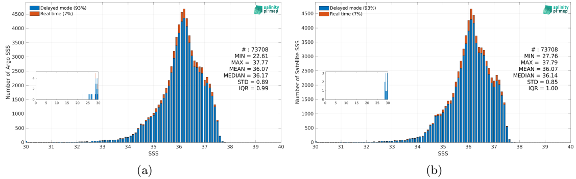
Figure 3: Histograms of SSS from Argo (a) and CCI SSS L4 Merged-OI v4.41 - 30-day running (ESA) (b) considering all match-up pairs per bins of 0.1 over the Tropical Atlantic Ocean Pi-MEP region and for the full satellite product period.
