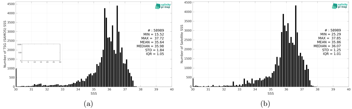
Figure 2: Histograms of SSS from TSG (SAMOS) (a) and CCI SSS L4 Merged-OI v4.4 - 7-day running (ESA) (b) considering all match-up pairs per bins of 0.1 over the Tropical Atlantic Ocean Pi-MEP region and for the full satellite product period.
