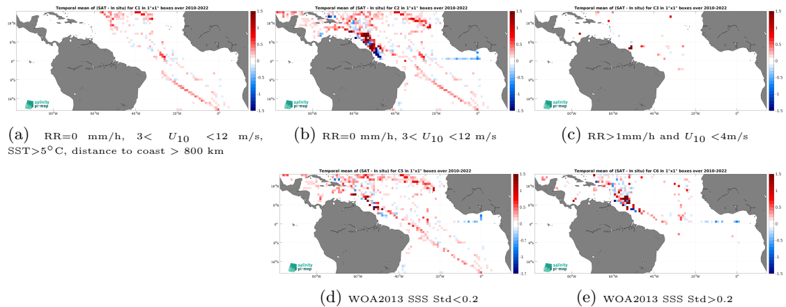
Figure 12: Temporal mean gridded over spatial boxes of size 1^\circ \times 1^\circ of \Delta\text{SSS} (CCI SSS L4 Merged-OI v4.4 - 7-day running (ESA) - TSG (SAMOS)) for 5 different subdatasets corresponding to:RR=0 mm/h, 3 < U_{10} < 12 m/s, SST >5^\circ\text{C} , distance to coast > 800 km (a), RR=0 mm/h, 3 < U_{10} < 12 m/s (b), RR >1 mm/h and U_{10} < 4 m/s (c), WOA2013 SSS Std <0.2 (d), WOA2013 SSS Std >0.2 (e).
