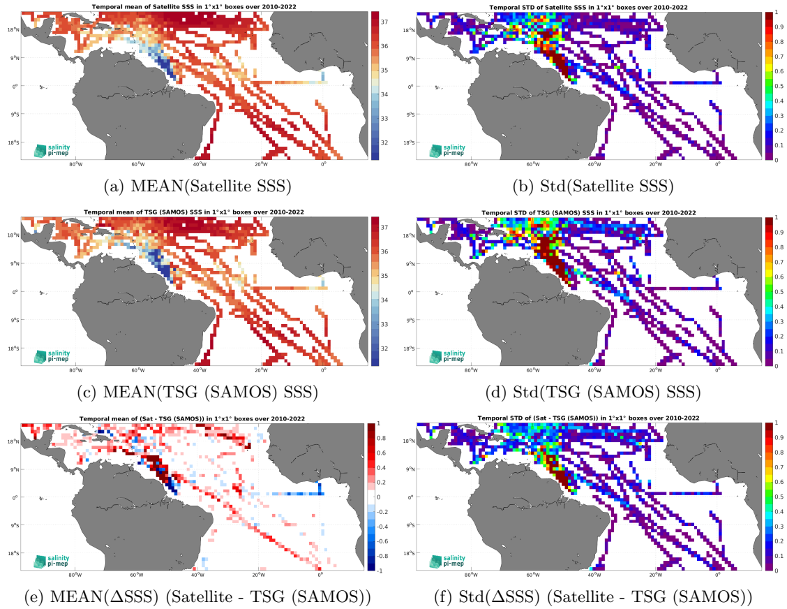
Figure 6: Temporal mean (left) and Std (right) of SSS from CCI SSS L4 Merged-OI v4.4 - 7-day running (ESA) (top), TSG (SAMOS) (middle), and of \Delta\text{SSS} (Satellite - TSG (SAMOS)). Only match-up pairs are used to generate these maps.
