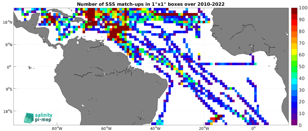
Figure 4: Number of SSS match-ups between TSG (SAMOS) SSS and the CCI SSS L4 Merged-OI v4.4 - 7-day running (ESA) SSS product for the Tropical Atlantic Ocean Pi-MEP region over 1^\circ \times 1^\circ boxes and for the full satellite product period.
