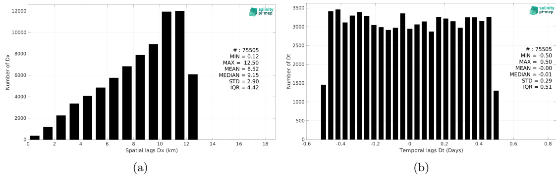
Figure 5: Histograms of the spatial (a) and temporal (b) lags between the location/time of the TSG (Polarstern) measurement and the date of the corresponding CCI SSS L4 Merged-OI v4.4 - 7-day running (ESA) SSS pixel.
