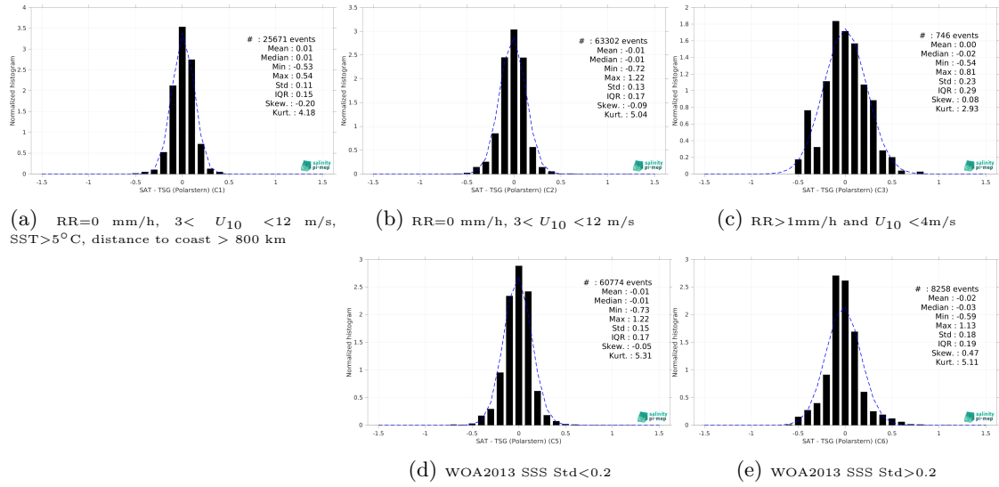
Figure 13: Normalized histogram of \Delta\text{SSS} (CCI SSS L4 Merged-OI v4.4 - 7-day running (ESA) - TSG (Polarstern)) for 5 different subdatasets corresponding to: RR=0 mm/h, 3 < U_{10} < 12 m/s, SST>5°C, distance to coast > 800 km (a), RR=0 mm/h, 3 < U_{10} < 12 m/s (b), RR>1mm/h and U_{10} < 4 m/s (c), WOA2013 SSS Std<0.2 (d), WOA2013 SSS Std>0.2 (e).
