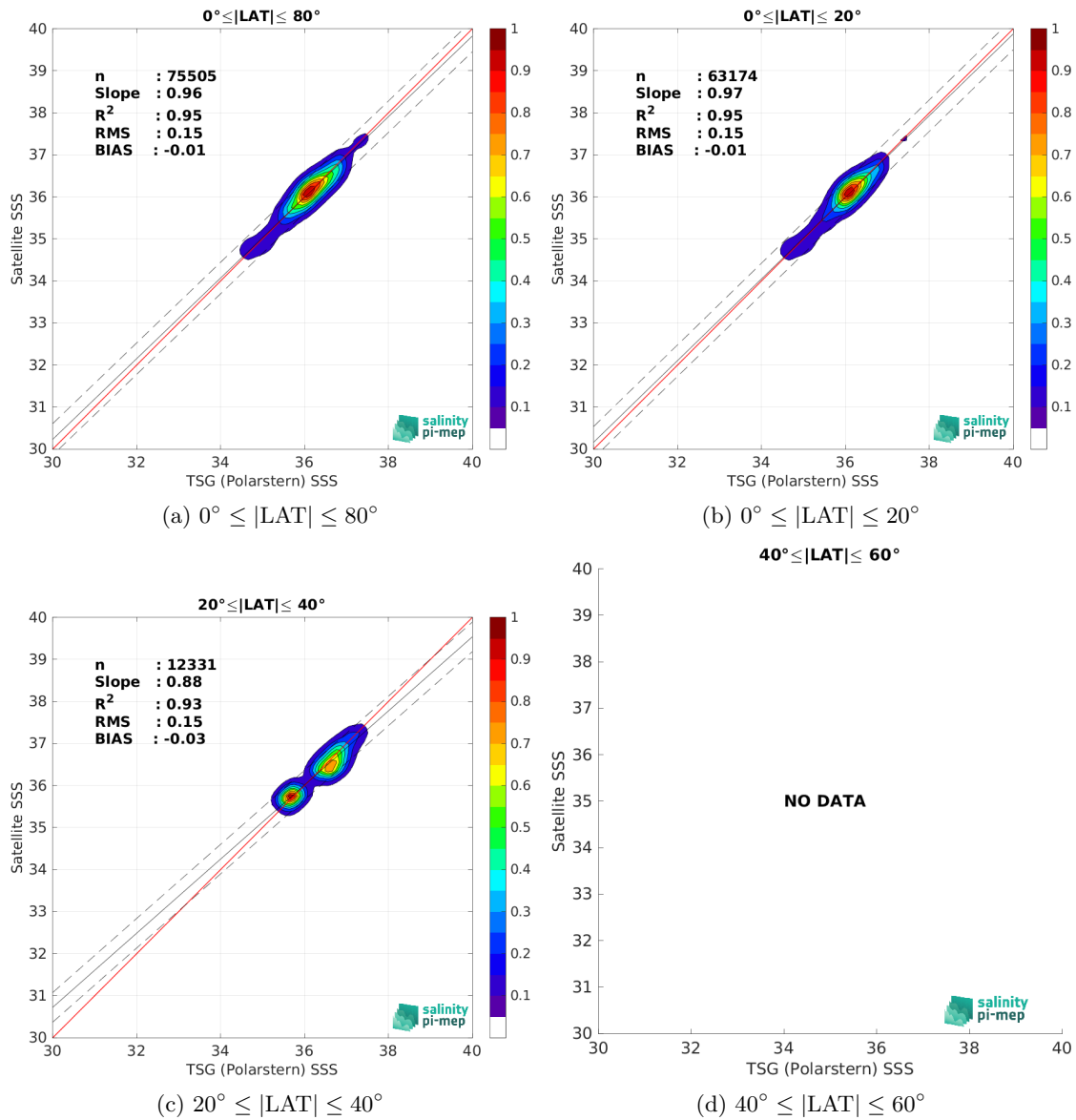
Figure 9: Contour maps of the concentration of CCI SSS L4 Merged-OI v4.4 - 7-day running (ESA) SSS (y-axis) versus TSG (Polarstern) SSS (x-axis) at match-up pairs for different latitude bands. For each plot, the red line shows x=y . The black thin and dashed lines indicate a linear fit through the data cloud and the \pm 95\% confidence levels, respectively. The number match-up pairs n , the slope and R^2 coefficient of the linear fit, the root mean square (RMS) and the mean bias between satellite and in situ data are indicated for each latitude band in each plots.
