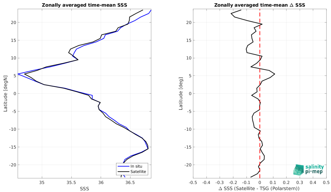
Figure 8: Left panel: Zonal mean SSS from CCI SSS L4 Merged-OI v4.4 - 7-day running (ESA) satellite product (black) and from TSG (Polarstern) (blue). Right panel: Zonal mean of \Delta SSS (Satellite - TSG (Polarstern)) for all the collected Pi-MEP match-up pairs estimated over the full satellite product period.
