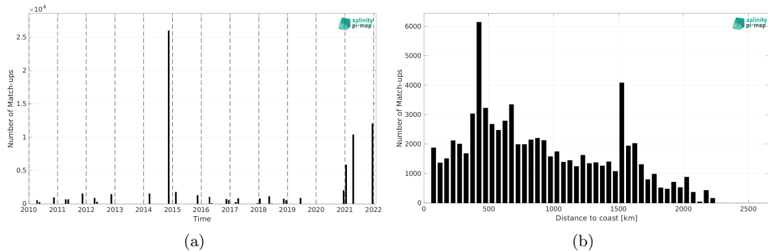
Figure 1: Number of match-ups between TSG (Polarstern) and CCI SSS L4 Merged-OI v4.4 - 7-day running (ESA) SSS as a function of time (a) and as function of the distance to coast (b) over the Tropical Atlantic Ocean Pi-MEP region and for the full satellite product period.
