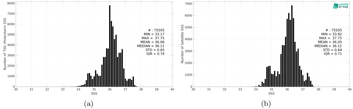
Figure 2: Histograms of SSS from TSG (Polarstern) (a) and CCI SSS L4 Merged-OI v4.4 - 7-day running (ESA) (b) considering all match-up pairs per bins of 0.1 over the Tropical Atlantic Ocean Pi-MEP region and for the full satellite product period.
