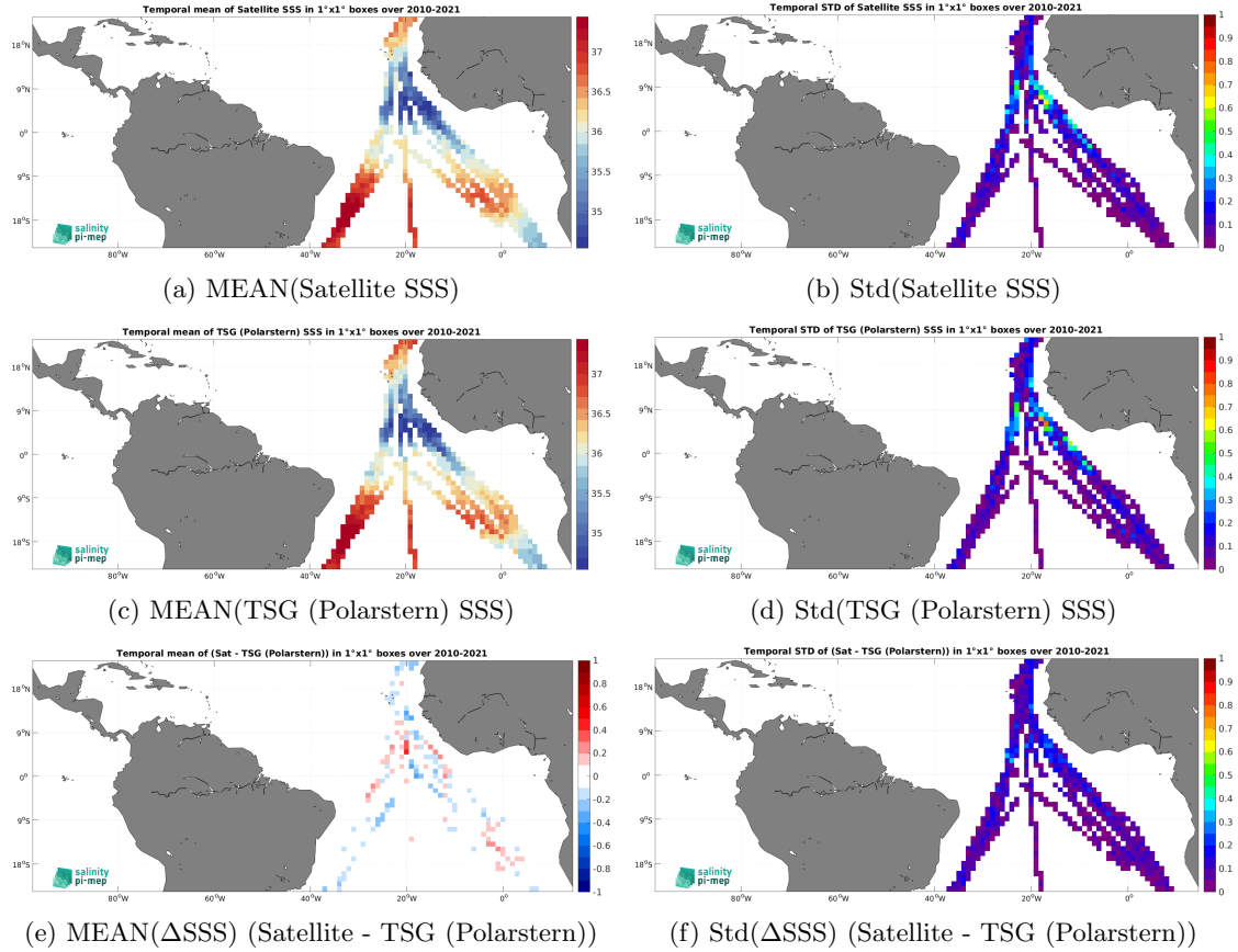
Figure 6: Temporal mean (left) and Std (right) of SSS from CCI SSS L4 Merged-OI v4.4 - 7-day running (ESA) (top), TSG (Polarstern) (middle), and of \Delta\text{SSS} (Satellite - TSG (Polarstern)). Only match-up pairs are used to generate these maps.
