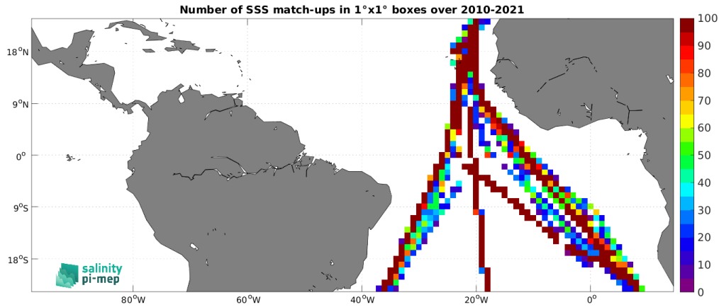
Figure 4: Number of SSS match-ups between TSG (Polarstern) SSS and the CCI SSS L4 Merged-OI v4.4 - 7-day running (ESA) SSS product for the Tropical Atlantic Ocean Pi-MEP region over 1^\circ \times 1^\circ boxes and for the full satellite product period.
