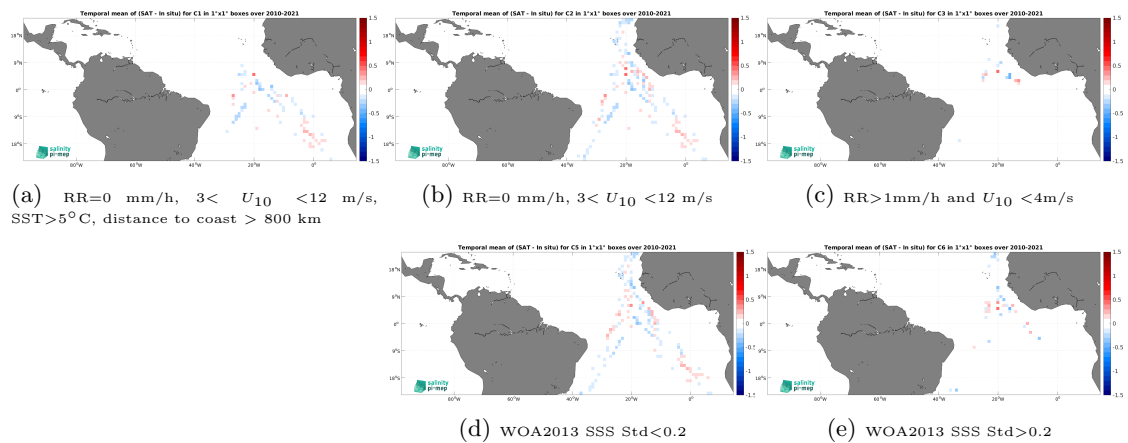
Figure 12: Temporal mean gridded over spatial boxes of size 1^\circ \times 1^\circ of \Delta\text{SSS} (CCI SSS L4 Merged-OI v4.4 - 7-day running (ESA) - TSG (Polarstern)) for 5 different subdatasets corresponding to:RR=0 mm/h, 3 < U_{10} < 12 m/s, SST >5^\circ\text{C} , distance to coast > 800 km (a), RR=0 mm/h, 3 < U_{10} < 12 m/s (b), RR >1 mm/h and U_{10} < 4 m/s (c), WOA2013 SSS Std <0.2 (d), WOA2013 SSS Std >0.2 (e).
