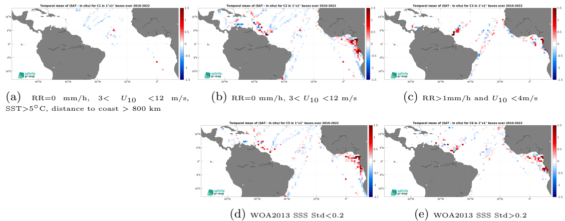
Figure 12: Temporal mean gridded over spatial boxes of size 1^\circ \times 1^\circ of \Delta SSS (CCI SSS L4 Merged-OI v4.4 - 7-day running (ESA) - TSG (LEGOS-DM)) for 5 different subdatasets corresponding to:RR=0 mm/h, 3 < U_{10} < 12 m/s, SST >5^\circ\text{C} , distance to coast > 800 km (a), RR=0 mm/h, 3 < U_{10} < 12 m/s (b), RR >1 mm/h and U_{10} < 4 m/s (c), WOA2013 SSS Std <0.2 (d), WOA2013 SSS Std >0.2 (e).
