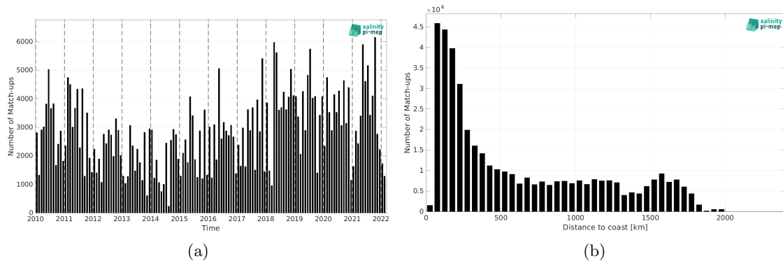
Figure 1: Number of match-ups between TSG (LEGOS-DM) and CCI SSS L4 Merged-OI v4.4 - 7-day running (ESA) SSS as a function of time (a) and as function of the distance to coast (b) over the Tropical Atlantic Ocean Pi-MEP region and for the full satellite product period.
