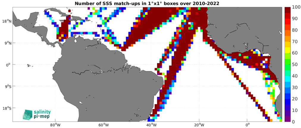
Figure 4: Number of SSS match-ups between TSG (LEGOS-DM) SSS and the CCI SSS L4 Merged-OI v4.4 - 7-day running (ESA) SSS product for the Tropical Atlantic Ocean Pi-MEP region over 1^\circ \times 1^\circ boxes and for the full satellite product period.
