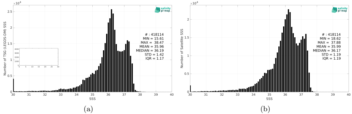
Figure 2: Histograms of SSS from TSG (LEGOS-DM) (a) and CCI SSS L4 Merged-OI v4.4 - 7-day running (ESA) (b) considering all match-up pairs per bins of 0.1 over the Tropical Atlantic Ocean Pi-MEP region and for the full satellite product period.
