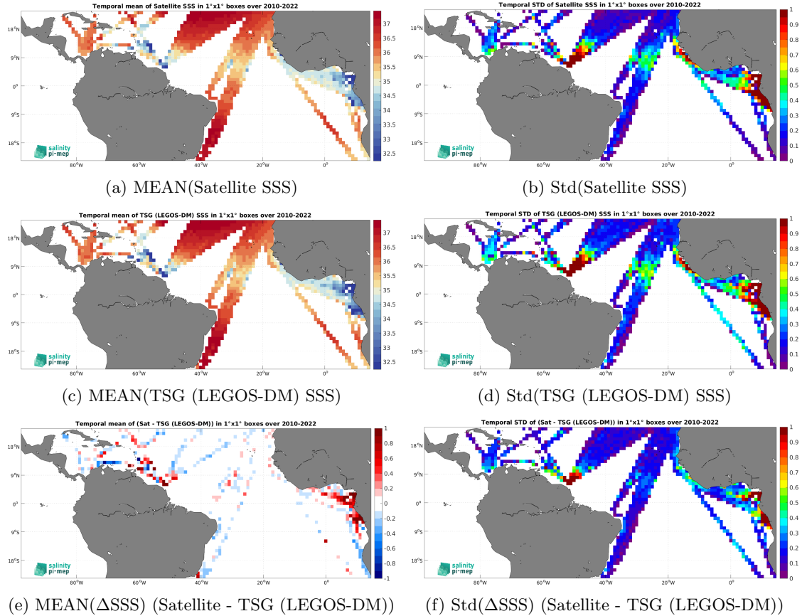
Figure 6: Temporal mean (left) and Std (right) of SSS from CCI SSS L4 Merged-OI v4.4 - 7-day running (ESA) (top), TSG (LEGOS-DM) (middle), and of \Delta\text{SSS} (Satellite - TSG (LEGOS-DM)). Only match-up pairs are used to generate these maps.
