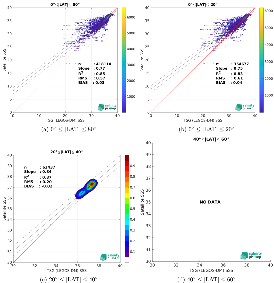
Figure 9: Contour maps of the concentration of CCI SSS L4 Merged-OI v4.4 - 7-day running (ESA) SSS (y-axis) versus TSG (LEGOS-DM) SSS (x-axis) at match-up pairs for different latitude bands. For each plot, the red line shows x=y . The black thin and dashed lines indicate a linear fit through the data cloud and the \pm 95\% confidence levels, respectively. The number match-up pairs n , the slope and R^2 coefficient of the linear fit, the root mean square (RMS) and the mean bias between satellite and in situ data are indicated for each latitude band in each plots.
