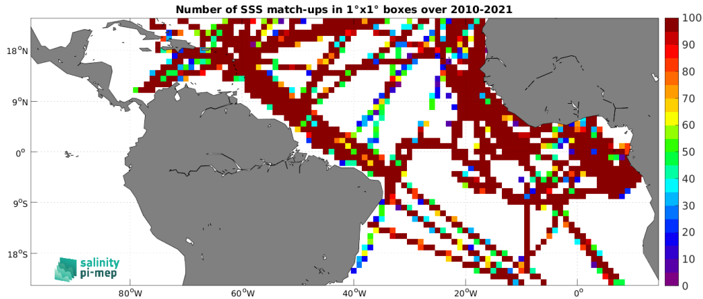
Figure 4: Number of SSS match-ups between TSG (GOSUD-Research-vessel) SSS and the CCI SSS L4 Merged-OI v4.4 - 7-day running (ESA) SSS product for the Tropical Atlantic Ocean Pi-MEP region over 1^\circ \times 1^\circ boxes and for the full satellite product period.
