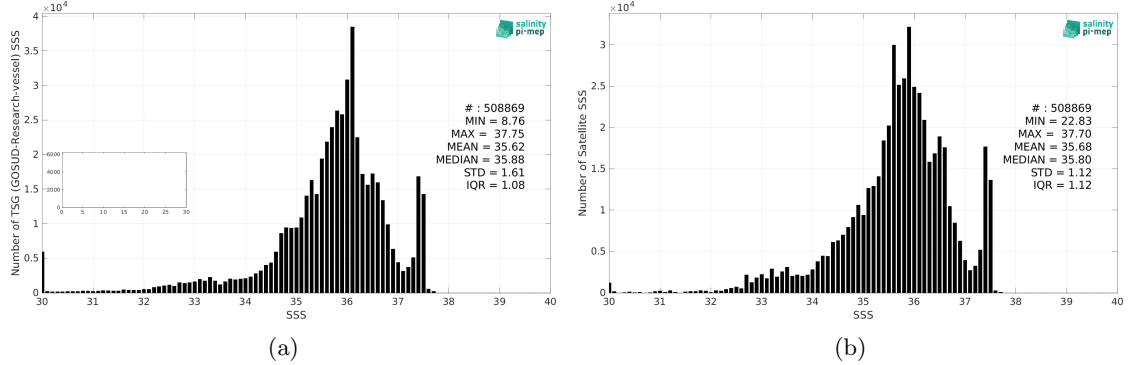
Figure 2: Histograms of SSS from TSG (GOSUD-Research-vessel) (a) and CCI SSS L4 Merged-OI v4.4 - 7-day running (ESA) (b) considering all match-up pairs per bins of 0.1 over the Tropical Atlantic Ocean Pi-MEP region and for the full satellite product period.
