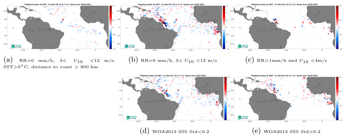
Figure 12: Temporal mean gridded over spatial boxes of size 1^\circ \times 1^\circ of \Delta\text{SSS} (CCI SSS L4 Merged-OI v4.4 - 7-day running (ESA) - TSG (GOSUD-Research-vessel)) for 5 different subdatasets corresponding to:RR=0 mm/h, 3 < U_{10} < 12 m/s, SST >5^\circ\text{C} , distance to coast > 800 km (a), RR=0 mm/h, 3 < U_{10} < 12 m/s (b), RR >1 mm/h and U_{10} < 4 m/s (c), WOA2013 SSS Std <0.2 (d), WOA2013 SSS Std >0.2 (e).
