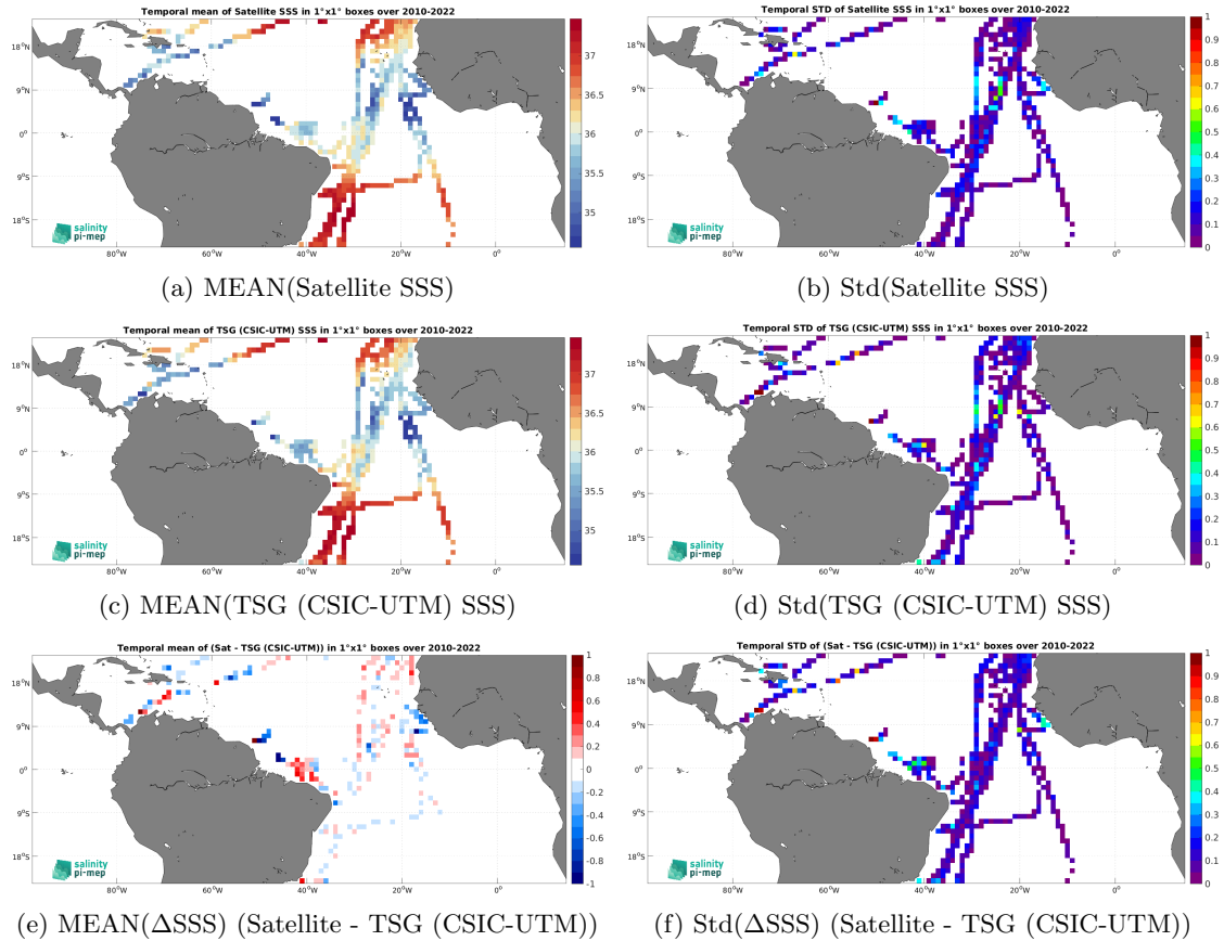
Figure 6: Temporal mean (left) and Std (right) of SSS from CCI SSS L4 Merged-OI v4.4 - 7-day running (ESA) (top), TSG (CSIC-UTM) ( in situ ) (middle), and of \Delta\text{SSS} (Satellite - TSG (CSIC-UTM)). Only match-up pairs are used to generate these maps.
