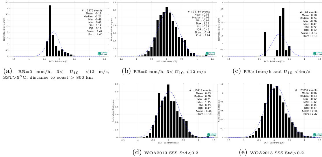
Figure 13: Normalized histogram of \Delta SSS (CCI SSS L4 Merged-OI v4.4 - 7-day running (ESA) - Sailldrone) for 5 different subdatasets corresponding to: RR=0 mm/h, 3 < U_{10} < 12 m/s, SST>5°C, distance to coast > 800 km (a), RR=0 mm/h, 3 < U_{10} < 12 m/s (b), RR>1mm/h and U_{10} < 4 m/s (c), WOA2013 SSS Std<0.2 (d), WOA2013 SSS Std>0.2 (e).
