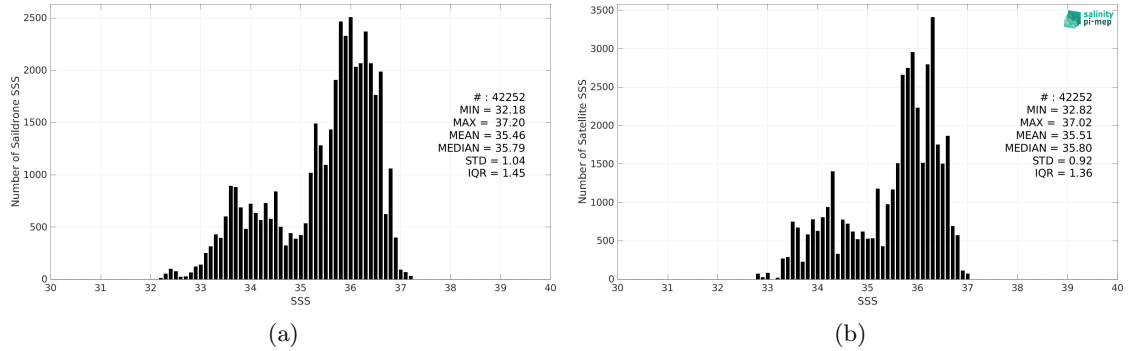
Figure 2: Histograms of SSS from Saildrone (a) and CCI SSS L4 Merged-OI v4.4 - 7-day running (ESA) (b) considering all match-up pairs per bins of 0.1 over the Tropical Atlantic Ocean Pi-MEP region and for the full satellite product period.
