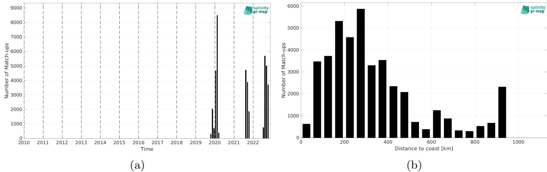
Figure 1: Number of match-ups between Saildrone and CCI SSS L4 Merged-OI v4.4 - 7-day running (ESA) SSS as a function of time (a) and as function of the distance to coast (b) over the Tropical Atlantic Ocean Pi-MEP region and for the full satellite product period.
