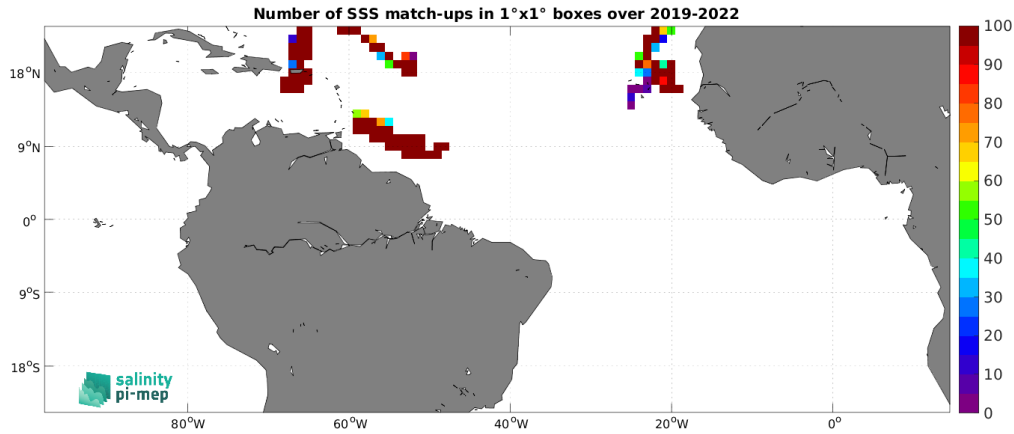
Figure 4: Number of SSS match-ups between Saildrone SSS and the CCI SSS L4 Merged-OI v4.4 - 7-day running (ESA) SSS product for the Tropical Atlantic Ocean Pi-MEP region over 1^\circ \times 1^\circ boxes and for the full satellite product period.
