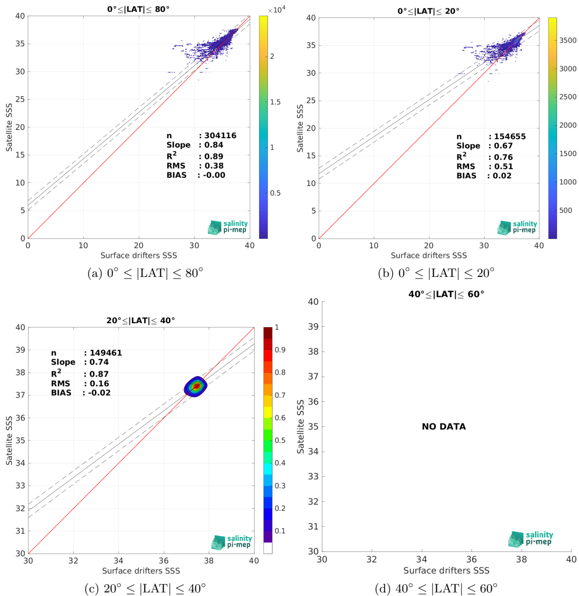
Figure 8: Contour maps of the concentration of CCI SSS L4 Merged-OI v4.4 - 7-day running (ESA) SSS (y-axis) versus Surface drifters SSS (x-axis) at match-up pairs for different latitude bands. For each plot, the red line shows x=y . The black thin and dashed lines indicate a linear fit through the data cloud and the \pm 95\% confidence levels, respectively. The number match-up pairs n , the slope and R^2 coefficient of the linear fit, the root mean square (RMS) and the mean bias between satellite and in situ data are indicated for each latitude band in each plots.
