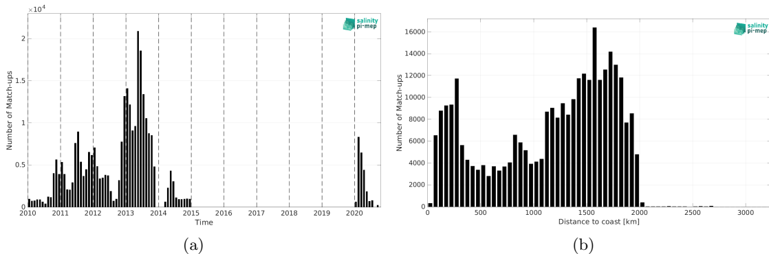
Figure 1: Number of match-ups between Surface drifters and CCI SSS L4 Merged-OI v4.4 - 7-day running (ESA) SSS as a function of time (a) and as function of the distance to coast (b) over the Tropical Atlantic Ocean Pi-MEP region and for the full satellite product period.
