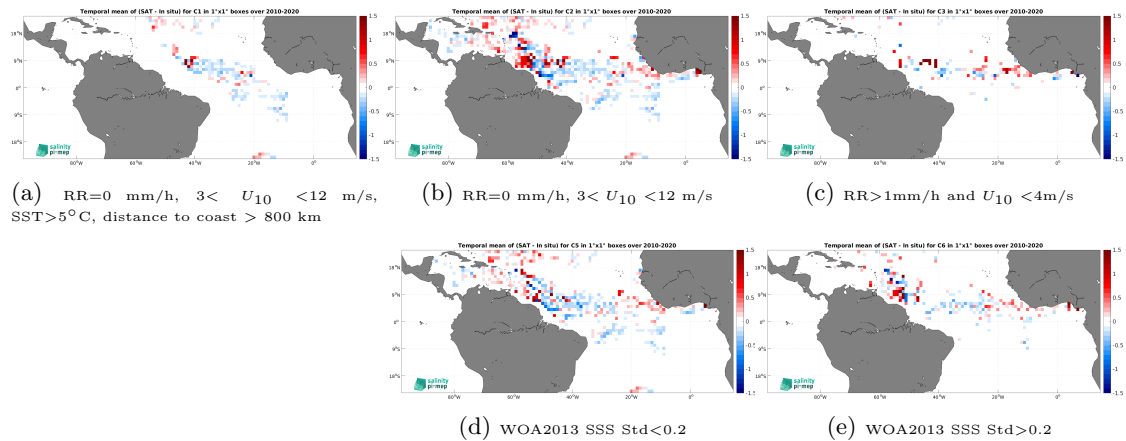
Figure 11: Temporal mean gridded over spatial boxes of size 1^\circ \times 1^\circ of \Delta\text{SSS} (CCI SSS L4 Merged-OI v4.4 - 7-day running (ESA) - Surface drifters) for 5 different subdatasets corresponding to:RR=0 mm/h, 3 < U_{10} < 12 m/s, SST >5^\circ\text{C} , distance to coast > 800 km (a), RR=0 mm/h, 3 < U_{10} < 12 m/s (b), RR >1 mm/h and U_{10} < 4 m/s (c), WOA2013 SSS Std <0.2 (d), WOA2013 SSS Std >0.2 (e).
