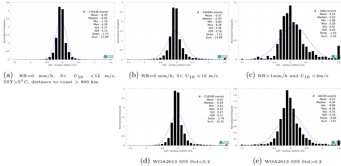
Figure 12: Normalized histogram of \Delta\text{SSS} (CCI SSS L4 Merged-OI v4.4 - 7-day running (ESA) - Surface drifters) for 5 different subdatasets corresponding to: RR=0 mm/h, 3 < U_{10} < 12 m/s, SST>5°C, distance to coast > 800 km (a), RR=0 mm/h, 3 < U_{10} < 12 m/s (b), RR>1mm/h and U_{10} < 4 m/s (c), WOA2013 SSS Std<0.2 (d), WOA2013 SSS Std>0.2 (e).
