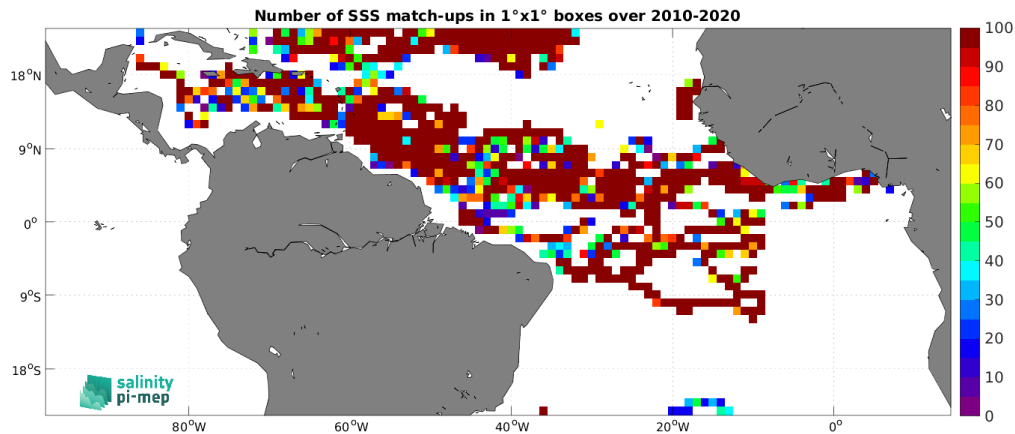
Figure 3: Number of SSS match-ups between Surface drifters SSS and the CCI SSS L4 Merged-OI v4.4 - 7-day running (ESA) SSS product for the Tropical Atlantic Ocean Pi-MEP region over 1^\circ \times 1^\circ boxes and for the full satellite product period.
