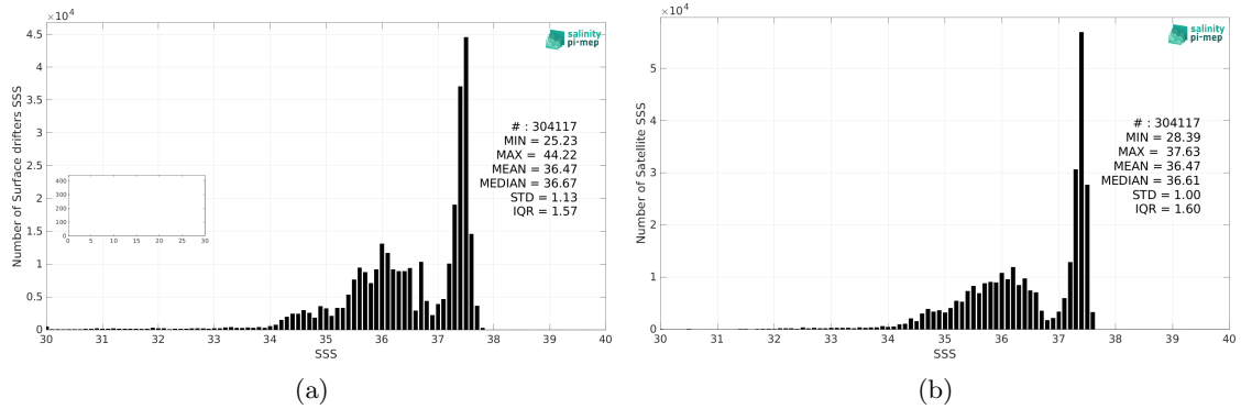
Figure 2: Histograms of SSS from Surface drifters (a) and CCI SSS L4 Merged-OI v4.4 - 7-day running (ESA) (b) considering all match-up pairs per bins of 0.1 over the Tropical Atlantic Ocean Pi-MEP region and for the full satellite product period.
