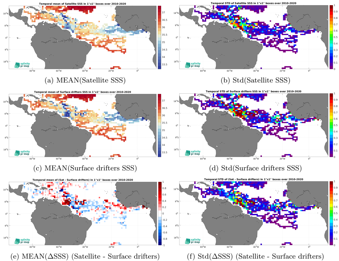
Figure 5: Temporal mean (left) and Std (right) of SSS from CCI SSS L4 Merged-OI v4.4 - 7-day running (ESA) (top), Surface drifters (middle), and of \Delta SSS (Satellite - Surface drifters). Only match-up pairs are used to generate these maps.
