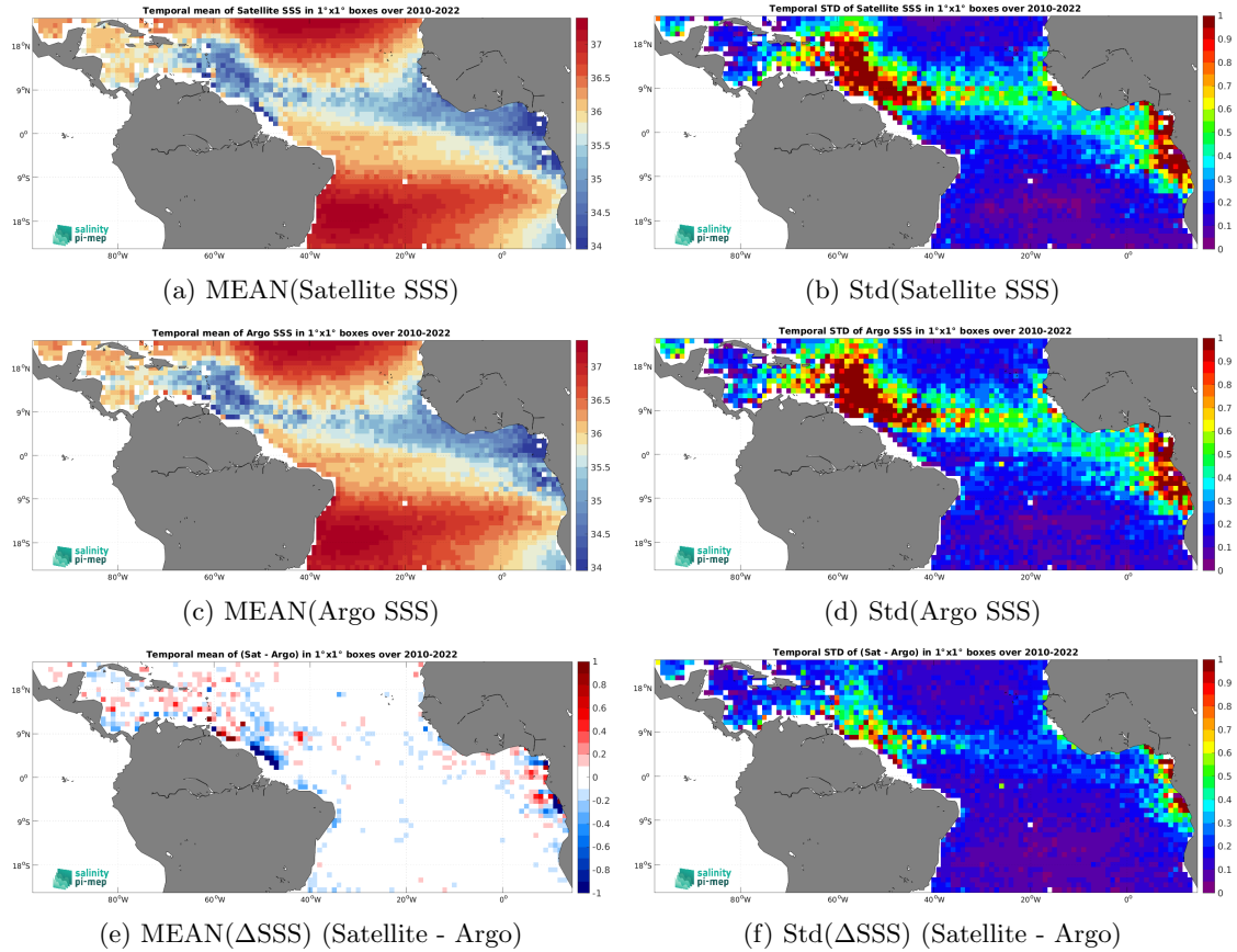
Figure 6: Temporal mean (left) and Std (right) of SSS from CCI SSS L4 Merged-OI v4.4 - 7-day running (ESA) (top), Argo (middle), and of \Delta\text{SSS} (Satellite - Argo). Only match-up pairs are used to generate these maps.
