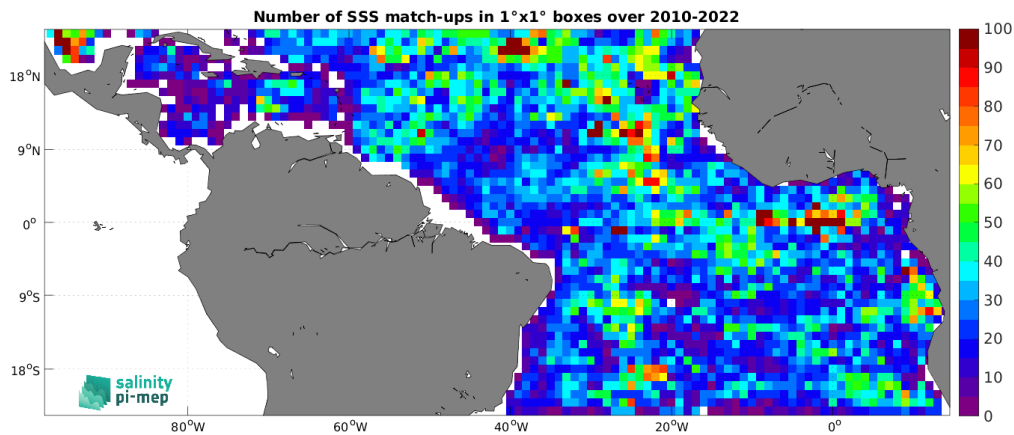
Figure 4: Number of SSS match-ups between Argo SSS and the CCI SSS L4 Merged-OI v4.4 - 7-day running (ESA) SSS product for the Tropical Atlantic Ocean Pi-MEP region over 1^\circ \times 1^\circ boxes and for the full satellite product period.
