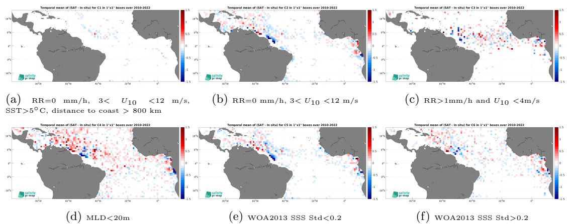
Figure 12: Temporal mean gridded over spatial boxes of size 1^\circ \times 1^\circ of \Delta SSS (CCI SSS L4 Merged-OI v4.4 - 7-day running (ESA) - Argo) for 6 different subdatasets corresponding to:RR=0 mm/h, 3 < U_{10} < 12 m/s, SST >5^\circ\text{C} , distance to coast > 800 km (a), RR=0 mm/h, 3 < U_{10} < 12 m/s (b), RR >1 mm/h and U_{10} < 4 m/s (c),MLD <20 m (d),WOA2013 SSS Std <0.2 (e),WOA2013 SSS Std >0.2 (f).
