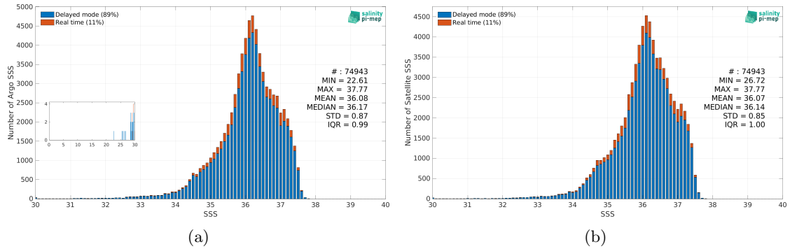
Figure 2: Histograms of SSS from Argo (a) and CCI SSS L4 Merged-OI v4.4 - 7-day running (ESA) (b) considering all match-up pairs per bins of 0.1 over the Tropical Atlantic Ocean Pi-MEP region and for the full satellite product period.
