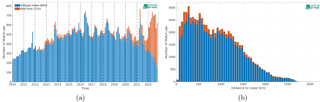
Figure 1: Number of match-ups between Argo and CCI SSS L4 Merged-OI v4.4 - 7-day running (ESA) SSS as a function of time (a) and as function of the distance to coast (b) over the Tropical Atlantic Ocean Pi-MEP region and for the full satellite product period.
