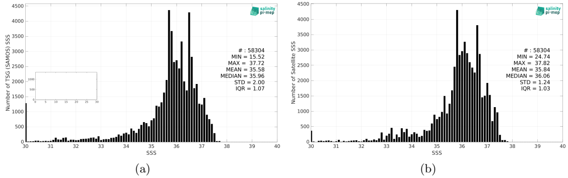
Figure 2: Histograms of SSS from TSG (SAMOS) (a) and CCI SSS L4 Merged-OI v4.4 - 30-day running (ESA) (b) considering all match-up pairs per bins of 0.1 over the Tropical Atlantic Ocean Pi-MEP region and for the full satellite product period.
