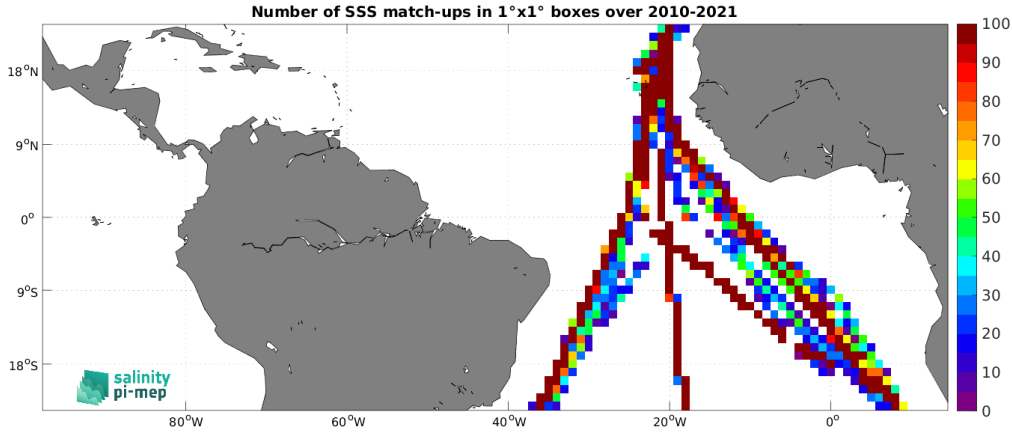
Figure 4: Number of SSS match-ups between TSG (Polarstern) SSS and the CCI SSS L4 Merged-OI v4.4 - 30-day running (ESA) SSS product for the Tropical Atlantic Ocean Pi-MEP region over 1^\circ \times 1^\circ boxes and for the full satellite product period.
