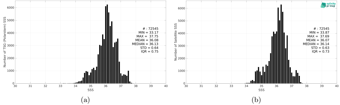
Figure 2: Histograms of SSS from TSG (Polarstern) (a) and CCI SSS L4 Merged-OI v4.4 - 30-day running (ESA) (b) considering all match-up pairs per bins of 0.1 over the Tropical Atlantic Ocean Pi-MEP region and for the full satellite product period.
