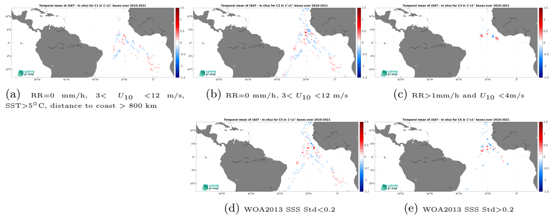
Figure 12: Temporal mean gridded over spatial boxes of size 1^\circ \times 1^\circ of \Delta\text{SSS} (CCI SSS L4 Merged-OI v4.4 - 30-day running (ESA) - TSG (Polarstern)) for 5 different subdatasets corresponding to:RR=0 mm/h, 3 < U_{10} < 12 m/s, SST >5^\circ\text{C} , distance to coast > 800 km (a), RR=0 mm/h, 3 < U_{10} < 12 m/s (b), RR >1 mm/h and U_{10} < 4 m/s (c), WOA2013 SSS Std <0.2 (d), WOA2013 SSS Std >0.2 (e).
