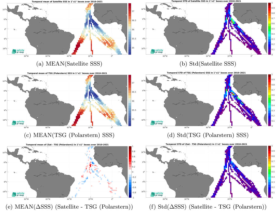
Figure 6: Temporal mean (left) and Std (right) of SSS from CCI SSS L4 Merged-OI v4.4 - 30-day running (ESA) (top), TSG (Polarstern) (middle), and of \Delta\text{SSS}(\text{Satellite} - \text{TSG}(\text{Polarstern})) . Only match-up pairs are used to generate these maps.
