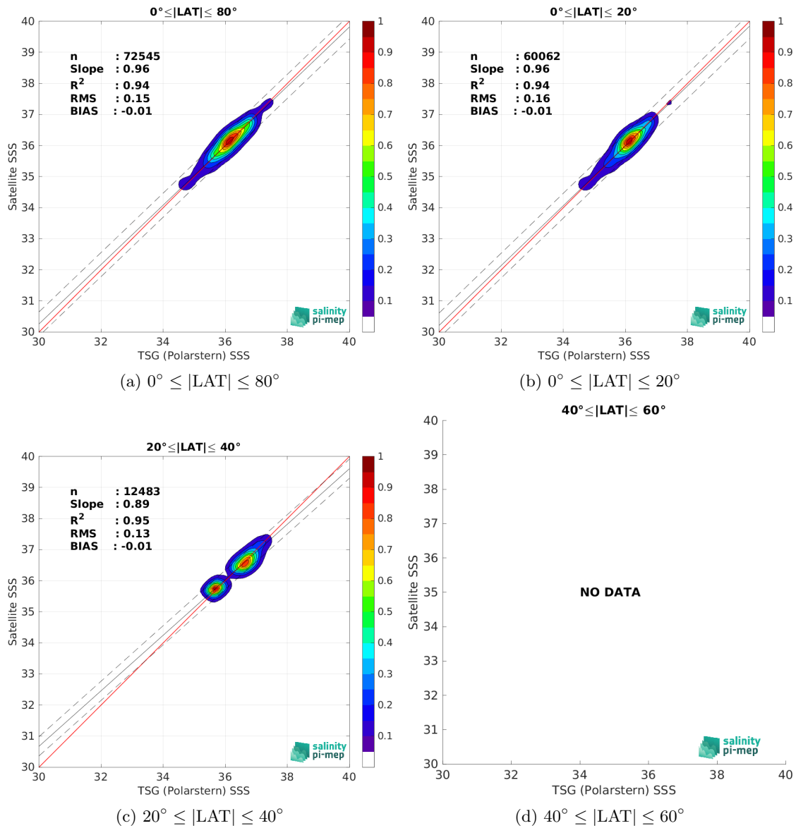
Figure 9: Contour maps of the concentration of CCI SSS L4 Merged-OI v4.4 - 30-day running (ESA) SSS (y-axis) versus TSG (Polarstern) SSS (x-axis) at match-up pairs for different latitude bands. For each plot, the red line shows x=y . The black thin and dashed lines indicate a linear fit through the data cloud and the \pm 95\% confidence levels, respectively. The number match-up pairs n , the slope and R^2 coefficient of the linear fit, the root mean square (RMS) and the mean bias between satellite and in situ data are indicated for each latitude band in each plots.
