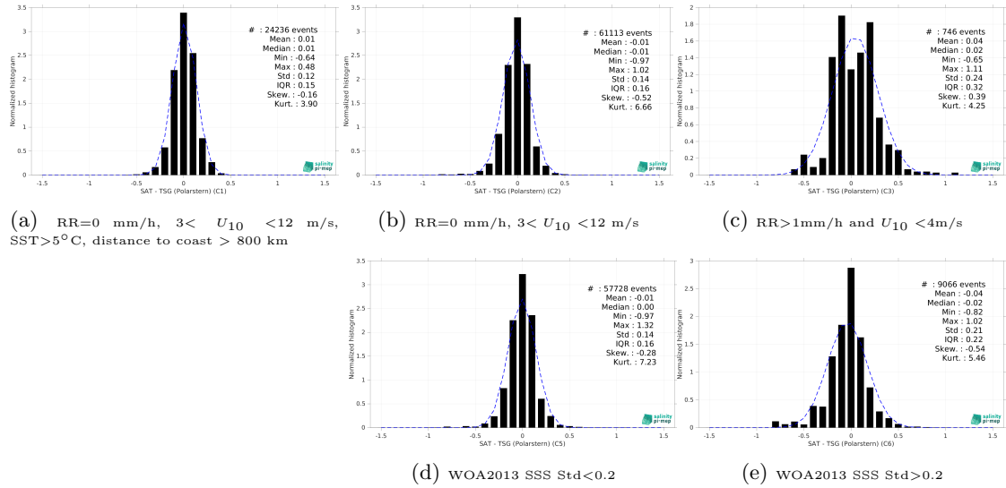
Figure 13: Normalized histogram of \Delta SSS (CCI SSS L4 Merged-OI v4.4 - 30-day running (ESA) - TSG (Polarstern)) for 5 different subdatasets corresponding to: RR=0 mm/h, 3 < U_{10} < 12 m/s, SST>5°C, distance to coast > 800 km (a), RR=0 mm/h, 3 < U_{10} < 12 m/s (b), RR>1mm/h and U_{10} < 4 m/s (c), WOA2013 SSS Std<0.2 (d), WOA2013 SSS Std>0.2 (e).
