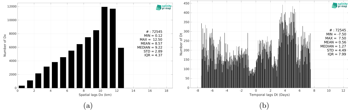
Figure 5: Histograms of the spatial (a) and temporal (b) lags between the location/time of the TSG (Polarstern) measurement and the date of the corresponding CCI SSS L4 Merged-OI v4.4 - 30-day running (ESA) SSS pixel.
