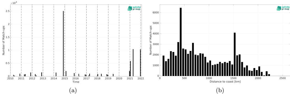
Figure 1: Number of match-ups between TSG (Polarstern) and CCI SSS L4 Merged-OI v4.4 - 30-day running (ESA) SSS as a function of time (a) and as function of the distance to coast (b) over the Tropical Atlantic Ocean Pi-MEP region and for the full satellite product period.
