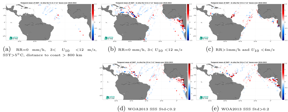
Figure 12: Temporal mean gridded over spatial boxes of size 1^\circ \times 1^\circ of \Delta\text{SSS} (CCI SSS L4 Merged-OI v4.4 - 30-day running (ESA) - TSG (LEGOS-DM)) for 5 different subdatasets corresponding to:RR=0 mm/h, 3 < U_{10} < 12 m/s, SST >5^\circ\text{C} , distance to coast > 800 km (a), RR=0 mm/h, 3 < U_{10} < 12 m/s (b), RR >1 mm/h and U_{10} < 4 m/s (c), WOA2013 SSS Std <0.2 (d), WOA2013 SSS Std >0.2 (e).
