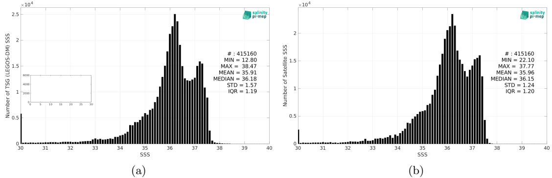
Figure 2: Histograms of SSS from TSG (LEGOS-DM) (a) and CCI SSS L4 Merged-OI v4.4 - 30-day running (ESA) (b) considering all match-up pairs per bins of 0.1 over the Tropical Atlantic Ocean Pi-MEP region and for the full satellite product period.
