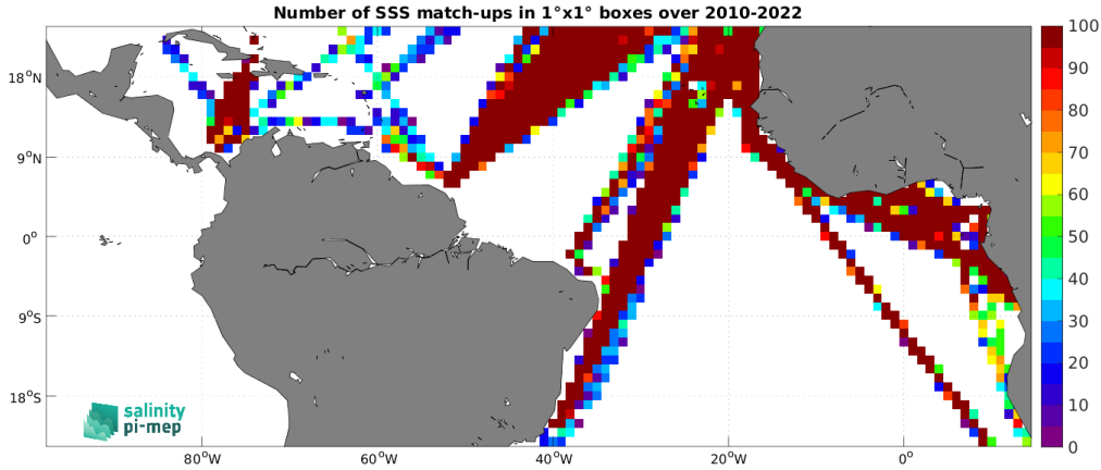
Figure 4: Number of SSS match-ups between TSG (LEGOS-DM) SSS and the CCI SSS L4 Merged-OI v4.4 - 30-day running (ESA) SSS product for the Tropical Atlantic Ocean Pi-MEP region over 1^\circ \times 1^\circ boxes and for the full satellite product period.
