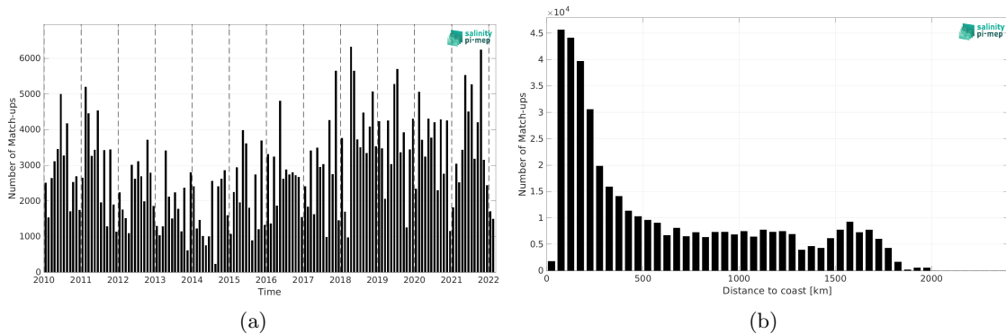
Figure 1: Number of match-ups between TSG (LEGOS-DM) and CCI SSS L4 Merged-OI v4.4 - 30-day running (ESA) SSS as a function of time (a) and as function of the distance to coast (b) over the Tropical Atlantic Ocean Pi-MEP region and for the full satellite product period.
