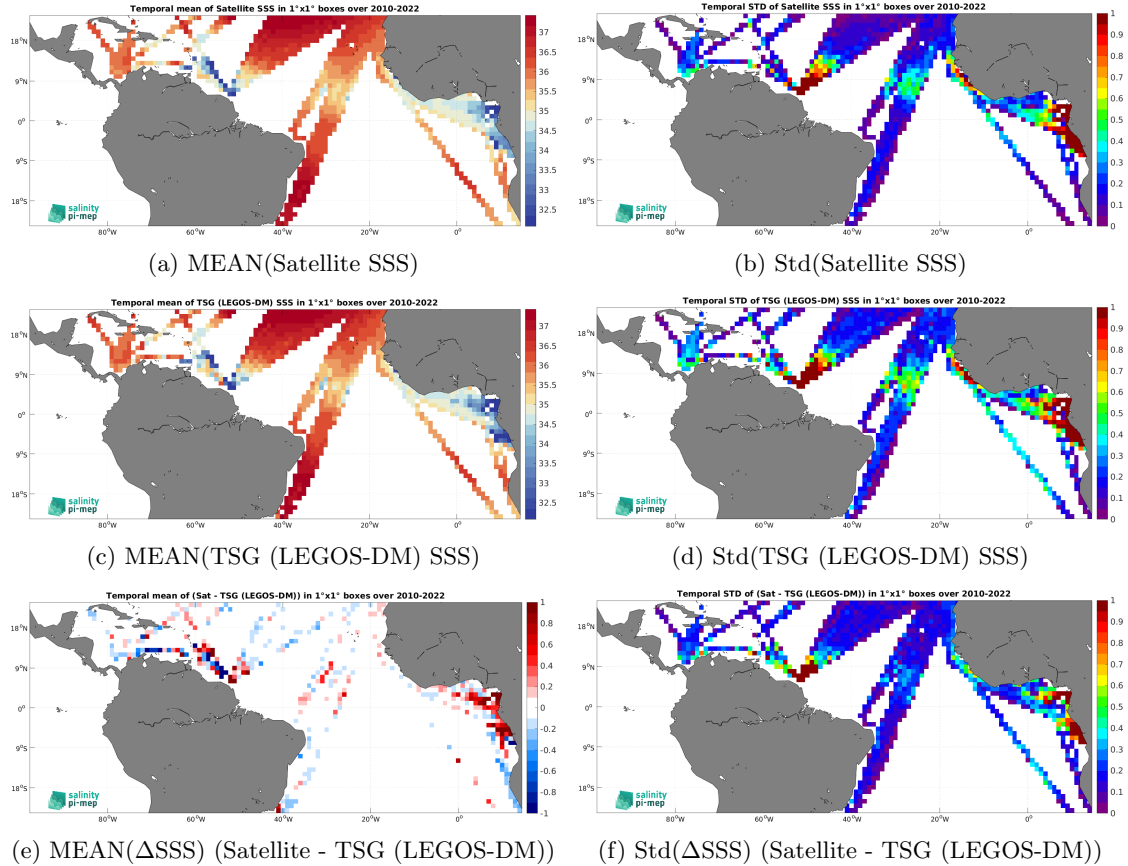
Figure 6: Temporal mean (left) and Std (right) of SSS from CCI SSS L4 Merged-OI v4.4 - 30-day running (ESA) (top), TSG (LEGOS-DM) (middle), and of \Delta\text{SSS} (Satellite - TSG (LEGOS-DM)). Only match-up pairs are used to generate these maps.
