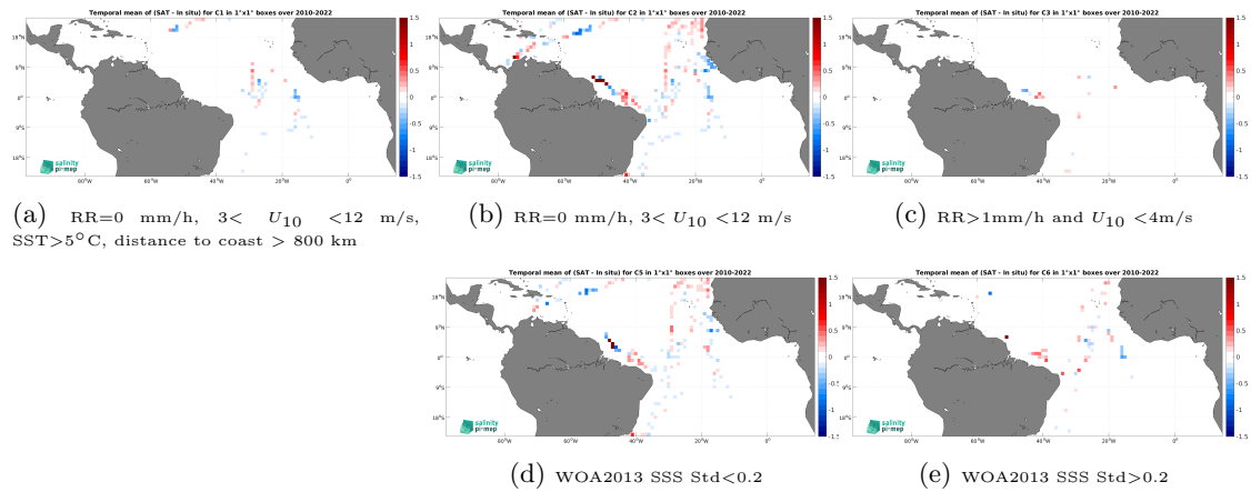
Figure 12: Temporal mean gridded over spatial boxes of size 1^\circ \times 1^\circ of \Delta\text{SSS} (CCI SSS L4 Merged-OI v4.4 - 30-day running (ESA) - TSG (CSIC-UTM)) for 5 different subdatasets corresponding to:RR=0 mm/h, 3 < U_{10} < 12 m/s, SST >5^\circ\text{C} , distance to coast > 800 km (a), RR=0 mm/h, 3 < U_{10} < 12 m/s (b), RR >1 mm/h and U_{10} < 4 m/s (c), WOA2013 SSS Std <0.2 (d), WOA2013 SSS Std >0.2 (e).
