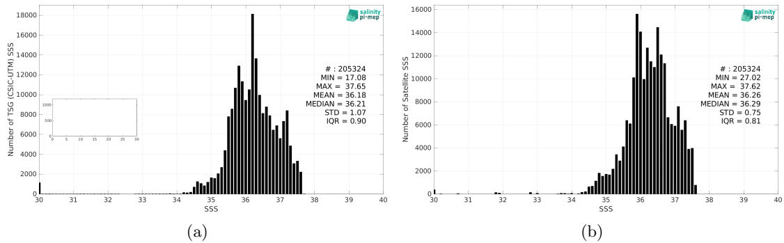
Figure 2: Histograms of SSS from TSG (CSIC-UTM) (a) and CCI SSS L4 Merged-OI v4.4 - 30-day running (ESA) (b) considering all match-up pairs per bins of 0.1 over the Tropical Atlantic Ocean Pi-MEP region and for the full satellite product period.
