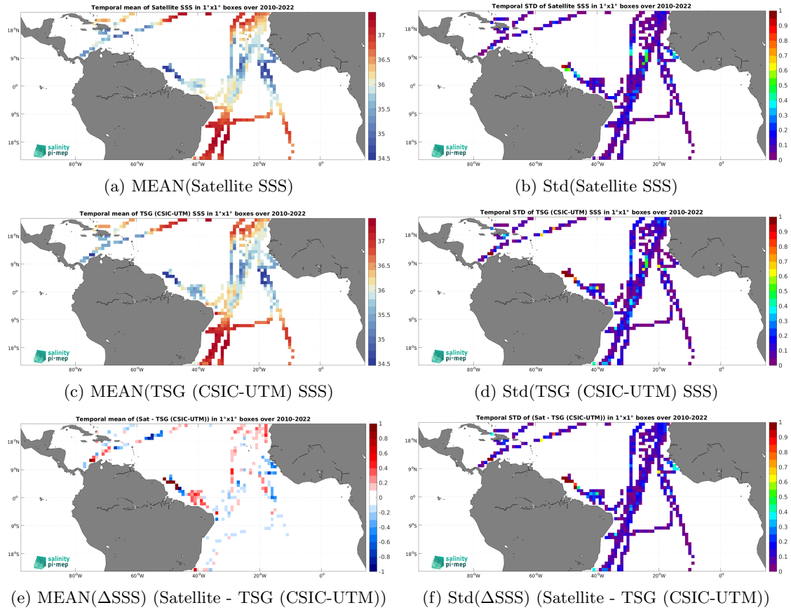
Figure 6: Temporal mean (left) and Std (right) of SSS from CCI SSS L4 Merged-OI v4.4 - 30-day running (ESA) (top), TSG (CSIC-UTM) (middle), and of \Delta\text{SSS} (Satellite - TSG (CSIC-UTM)). Only match-up pairs are used to generate these maps.
