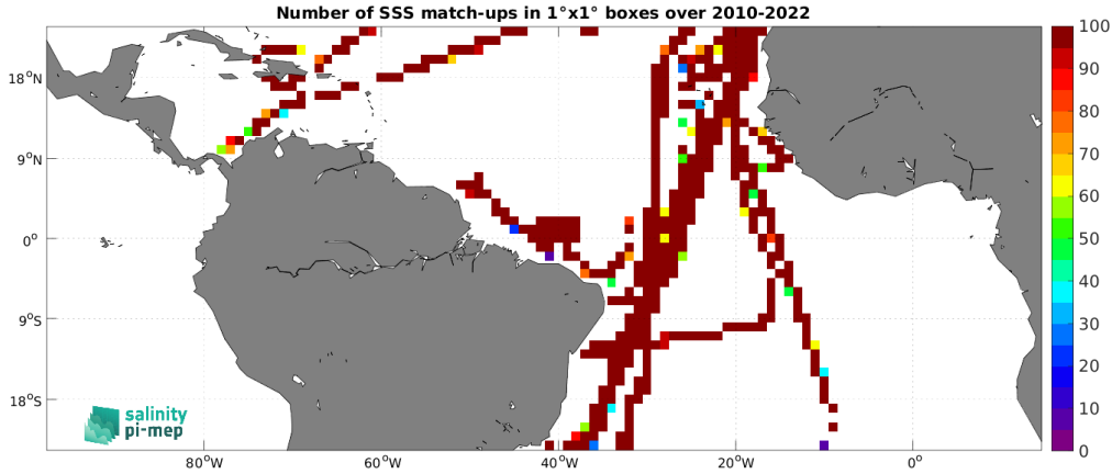
Figure 4: Number of SSS match-ups between TSG (CSIC-UTM) SSS and the CCI SSS L4 Merged-OI v4.4 - 30-day running (ESA) SSS product for the Tropical Atlantic Ocean Pi-MEP region over 1^\circ \times 1^\circ boxes and for the full satellite product period.
