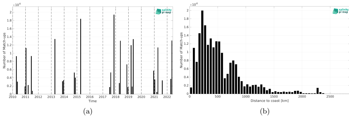
Figure 1: Number of match-ups between TSG (CSIC-UTM) and CCI SSS L4 Merged-OI v4.4 - 30-day running (ESA) SSS as a function of time (a) and as function of the distance to coast (b) over the Tropical Atlantic Ocean Pi-MEP region and for the full satellite product period.
