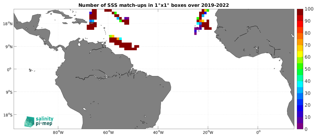
Figure 4: Number of SSS match-ups between Saildrone SSS and the CCI SSS L4 Merged-OI v4.4 - 30-day running (ESA) SSS product for the Tropical Atlantic Ocean Pi-MEP region over 1^\circ \times 1^\circ boxes and for the full satellite product period.
