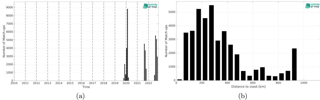
Figure 1: Number of match-ups between Saildrone and CCI SSS L4 Merged-OI v4.4 - 30-day running (ESA) SSS as a function of time (a) and as function of the distance to coast (b) over the Tropical Atlantic Ocean Pi-MEP region and for the full satellite product period.
