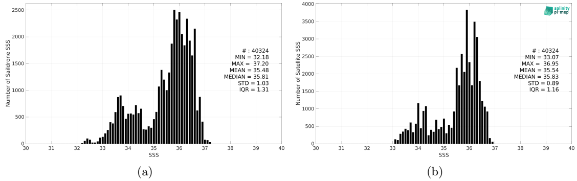
Figure 2: Histograms of SSS from Saildrone (a) and CCI SSS L4 Merged-OI v4.4 - 30-day running (ESA) (b) considering all match-up pairs per bins of 0.1 over the Tropical Atlantic Ocean Pi-MEP region and for the full satellite product period.
