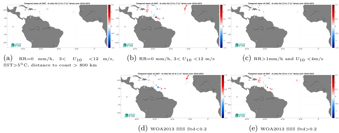
Figure 12: Temporal mean gridded over spatial boxes of size 1^\circ \times 1^\circ of \Delta\text{SSS} (CCI SSS L4 Merged-OI v4.4 - 30-day running (ESA) - Saildrone) for 5 different subdatasets corresponding to:RR=0 mm/h, 3 < U_{10} < 12 m/s, SST >5^\circ\text{C} , distance to coast > 800 km (a), RR=0 mm/h, 3 < U_{10} < 12 m/s (b), RR >1 mm/h and U_{10} < 4 m/s (c), WOA2013 SSS Std <0.2 (d), WOA2013 SSS Std >0.2 (e).
