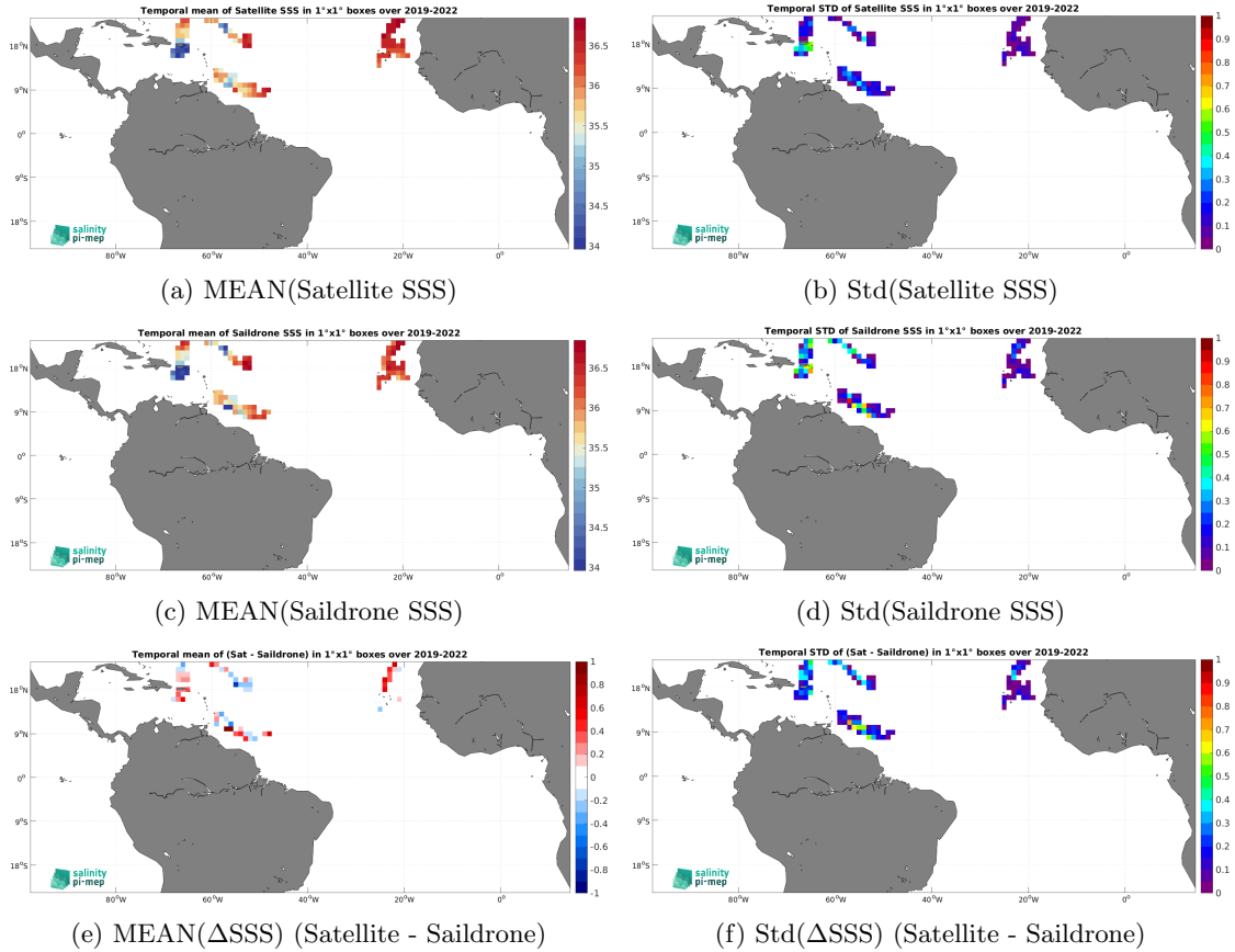
Figure 6: Temporal mean (left) and Std (right) of SSS from CCI SSS L4 Merged-OI v4.4 - 30-day running (ESA) (top), Saildrone (middle), and of \Delta\text{SSS} (Satellite - Saildrone). Only match-up pairs are used to generate these maps.
