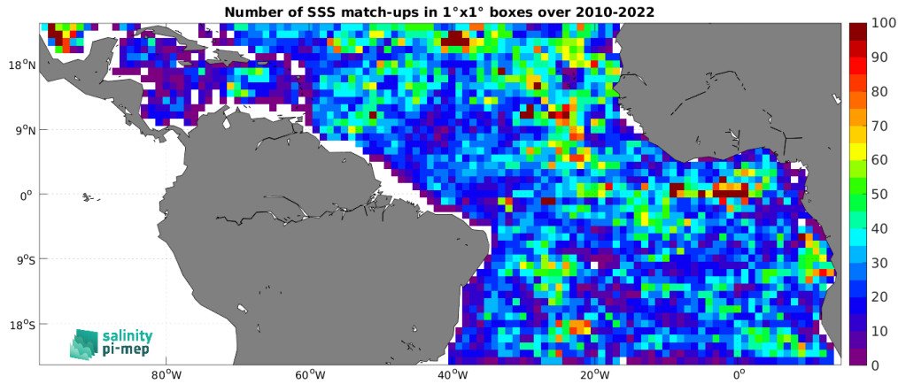
Figure 4: Number of SSS match-ups between Argo SSS and the CCI SSS L4 Merged-OI v4.4 - 30-day running (ESA) SSS product for the Tropical Atlantic Ocean Pi-MEP region over 1^\circ \times 1^\circ boxes and for the full satellite product period.
