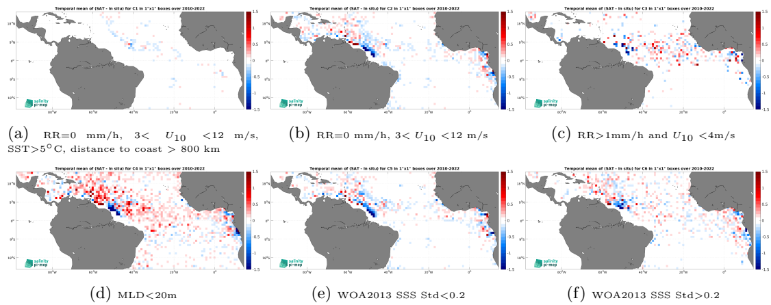
Figure 12: Temporal mean gridded over spatial boxes of size 1^\circ \times 1^\circ of \Delta SSS (CCI SSS L4 Merged-OI v4.4 - 30-day running (ESA) - Argo) for 6 different subdatasets corresponding to:RR=0 mm/h, 3 < U_{10} < 12 m/s, SST >5^\circ C, distance to coast > 800 km (a), RR=0 mm/h, 3 < U_{10} < 12 m/s (b), RR >1 mm/h and U_{10} < 4 m/s (c),MLD <20 m (d),WOA2013 SSS Std <0.2 (e),WOA2013 SSS Std >0.2 (f).
