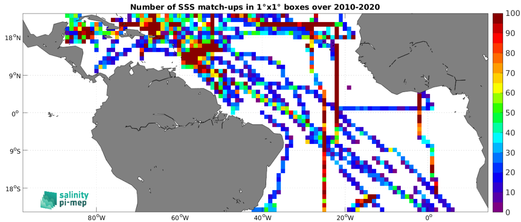
Figure 4: Number of SSS match-ups between TSG (SAMOS) SSS and the CCI SSS L4 Merged-OI v3.2 - 7-day running (ESA) SSS product for the Tropical Atlantic Ocean Pi-MEP region over 1^\circ \times 1^\circ boxes and for the full satellite product period.
