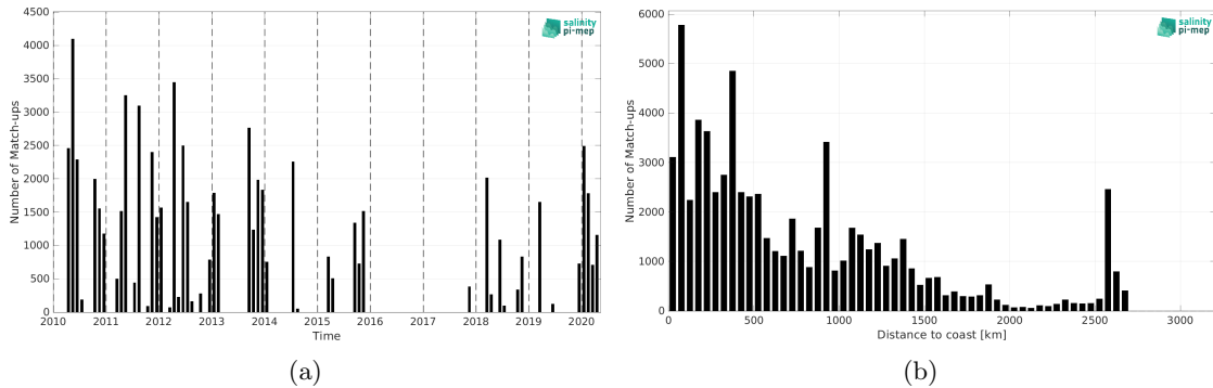
Figure 1: Number of match-ups between TSG (SAMOS) and CCI SSS L4 Merged-OI v3.2 - 7-day running (ESA) SSS as a function of time (a) and as function of the distance to coast (b) over the Tropical Atlantic Ocean Pi-MEP region and for the full satellite product period.
