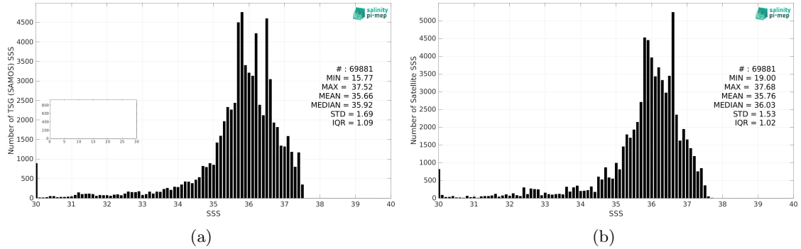
Figure 2: Histograms of SSS from TSG (SAMOS) (a) and CCI SSS L4 Merged-OI v3.2 - 7-day running (ESA) (b) considering all match-up pairs per bins of 0.1 over the Tropical Atlantic Ocean Pi-MEP region and for the full satellite product period.
