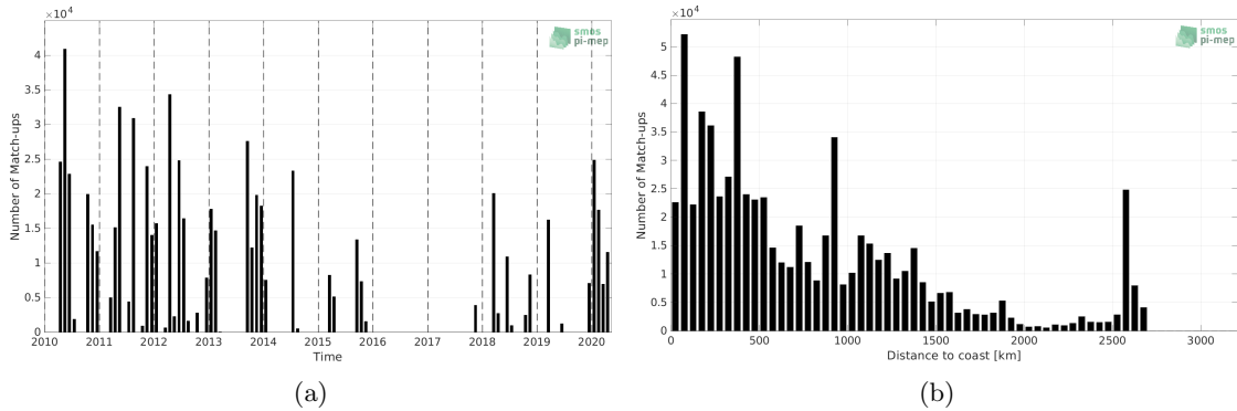
Figure 1: Number of match-ups between TSG (SAMOS) and CCI SSS L4 Merged-OI v3.2 - 7-day running (ESA) SSS as a function of time (a) and as function of the distance to coast (b) over the Tropical Atlantic Ocean Pi-MEP region and for the full satellite product period.
