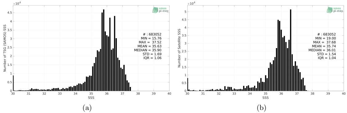
Figure 2: Histograms of SSS from TSG (SAMOS) (a) and CCI SSS L4 Merged-OI v3.2 - 7-day running (ESA) (b) considering all match-up pairs per bins of 0.1 over the Tropical Atlantic Ocean Pi-MEP region and for the full satellite product period.
