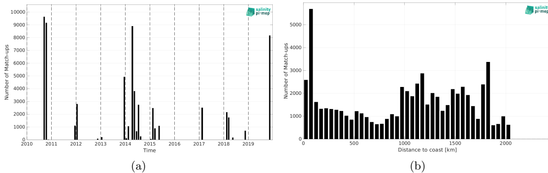
Figure 1: Number of match-ups between TSG (GOSUD-Sailing-ship) and CCI SSS L4 Merged-OI v3.2 - 7-day running (ESA) SSS as a function of time (a) and as function of the distance to coast (b) over the Tropical Atlantic Ocean Pi-MEP region and for the full satellite product period.
