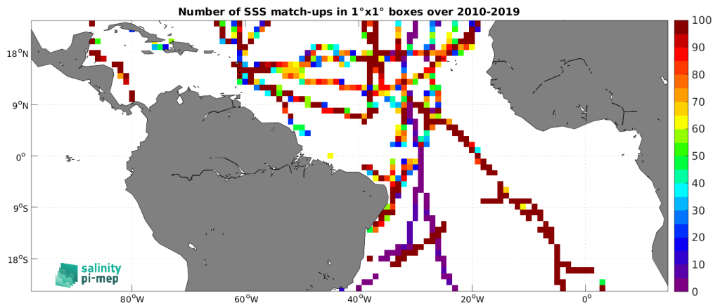
Figure 4: Number of SSS match-ups between TSG (GOSUD-Sailing-ship) SSS and the CCI SSS L4 Merged-OI v3.2 - 7-day running (ESA) SSS product for the Tropical Atlantic Ocean Pi-MEP region over 1^\circ \times 1^\circ boxes and for the full satellite product period.
