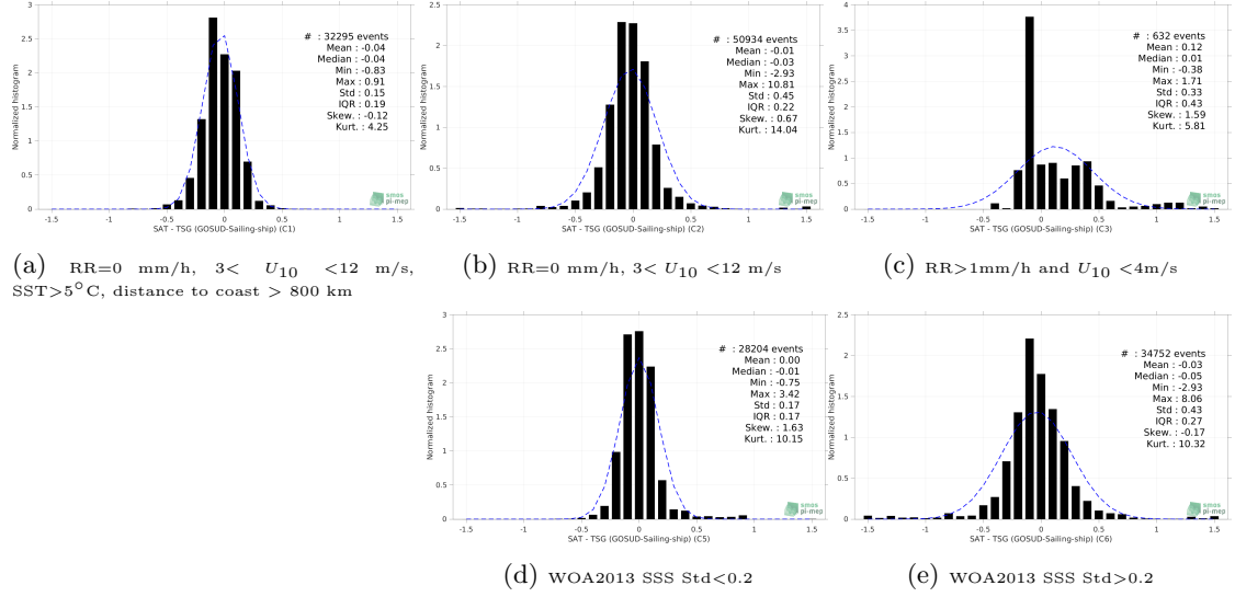
Figure 13: Normalized histogram of \Delta\text{SSS} (CCI SSS L4 Merged-OI v3.2 - 7-day running (ESA) - TSG (GOSUD-Sailing-ship)) for 5 different subdatasets corresponding to: RR=0 mm/h, 3 < U_{10} < 12 m/s, SST>5°C, distance to coast > 800 km (a), RR=0 mm/h, 3 < U_{10} < 12 m/s (b), RR>1mm/h and U_{10} < 4 m/s (c), WOA2013 SSS Std<0.2 (d), WOA2013 SSS Std>0.2 (e).
