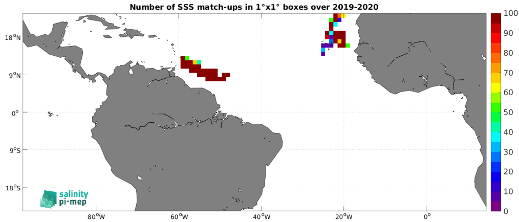
Figure 4: Number of SSS match-ups between Saildrone SSS and the CCI SSS L4 Merged-OI v3.2 - 7-day running (ESA) SSS product for the Tropical Atlantic Ocean Pi-MEP region over 1^\circ \times 1^\circ boxes and for the full satellite product period.
