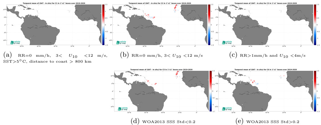
Figure 12: Temporal mean gridded over spatial boxes of size 1^\circ \times 1^\circ of \Delta SSS (CCI SSS L4 Merged-OI v3.2 - 7-day running (ESA) - Sailability) for 5 different subdatasets corresponding to:RR=0 mm/h, 3 < U_{10} < 12 m/s, SST >5^\circ\text{C} , distance to coast > 800 km (a), RR=0 mm/h, 3 < U_{10} < 12 m/s (b), RR >1 mm/h and U_{10} < 4 m/s (c), WOA2013 SSS Std <0.2 (d), WOA2013 SSS Std >0.2 (e).
